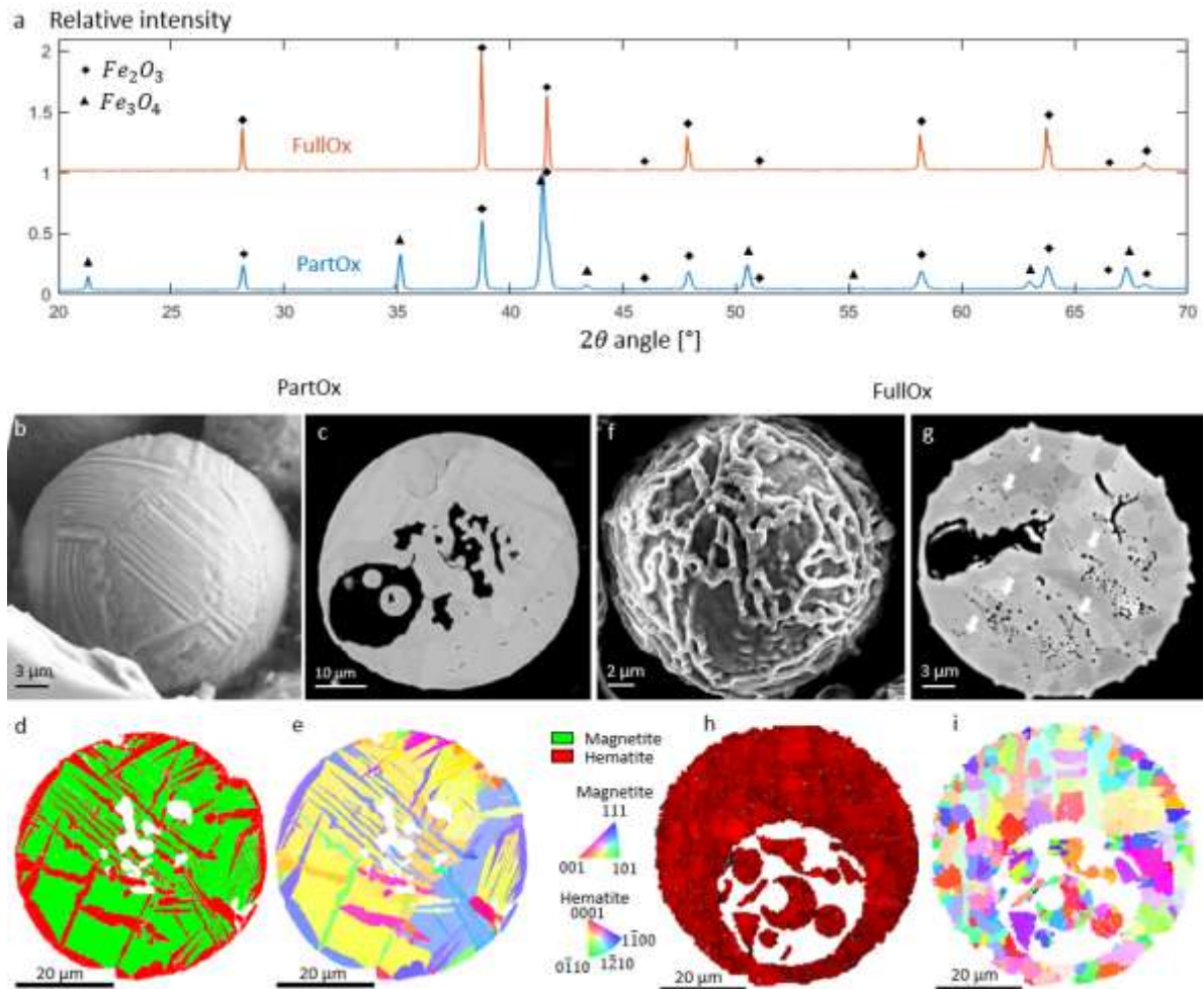
Figure 1 Microstructural characterization of the combusted iron particles, prior to the reduction process: (a) X-ray diffraction (XRD) analysis (with a Co target); (b-e) combusted powder (PartOx) and (f-i) combusted powder subjected to an additional deep pre-oxidation treatment (FullOx). (b, f) Scanning electron microscopy (SEM) image of the surface, with secondary electrons contrast, and (c, g) of the cross section of a particle, with backscattered electrons contrast. (d, h) Electron backscatter diffraction (EBSD) phase map and (e, i) crystalline orientation map. The arrows in (g) highlight the additional porosities formed during the deep pre-oxidation treatment.
