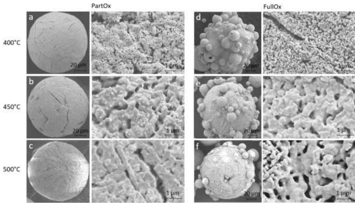
Figure 8 Scanning electron microscopy (SEM) images with secondary electrons contrast of the surface porosity formed after full reduction of (a-c) PartOx powder and (d-f) FullOx powder at (a, d) 400°C, (b, e) 450°C and (c, f) 500°C in the thermogravimetry (TG) reactor.
