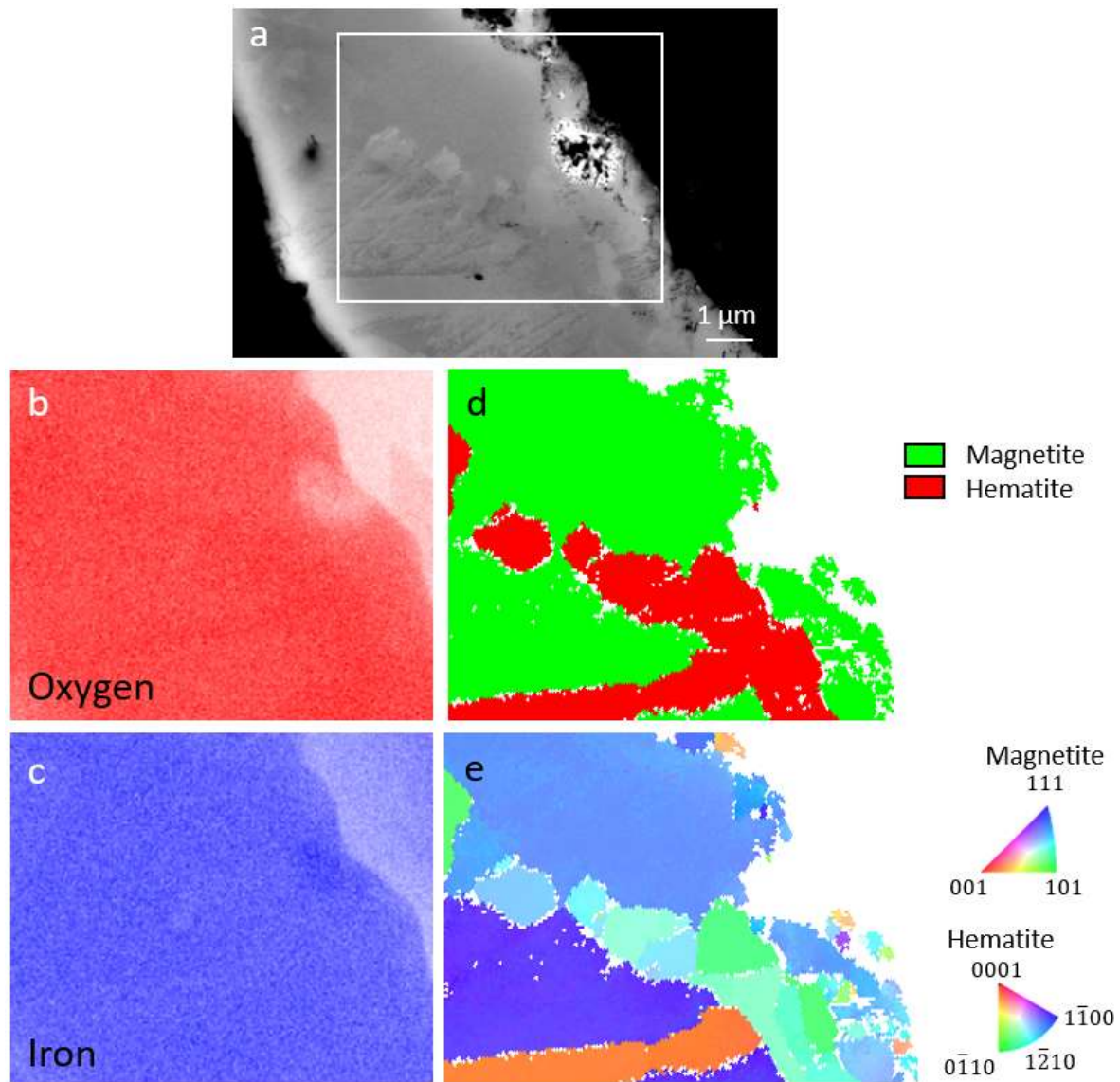
Figure 5 Electron backscatter diffraction (EBSD) and energy dispersive spectroscopy (EDS) maps of a PartOx particle partially reduced to a reduction level of 0.03 in the thermogravimetry (TG) reactor at 500 °C. (a) The corresponding scanning electron microscopy (SEM) image, (b) oxygen and (c) iron EDS map, (d) EBSD phase map, and (e) EBSD inverse pole figure (IPF) related to the sample normal direction.
