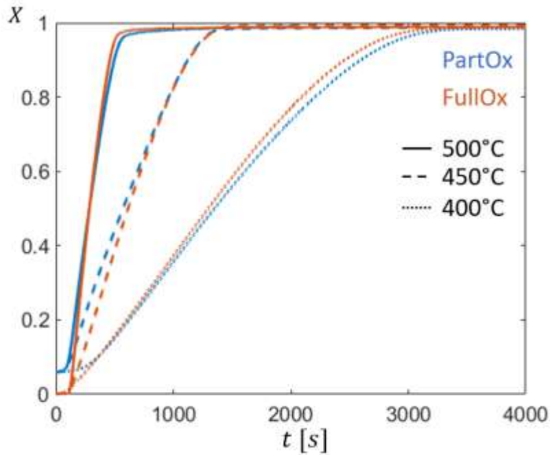
Figure 2 Reduction kinetics of the combusted powder (PartOx) and the pre-oxidized powder (FullOx) at 400-500°C, calculated based on the thermogravimetry analysis (TGA).
