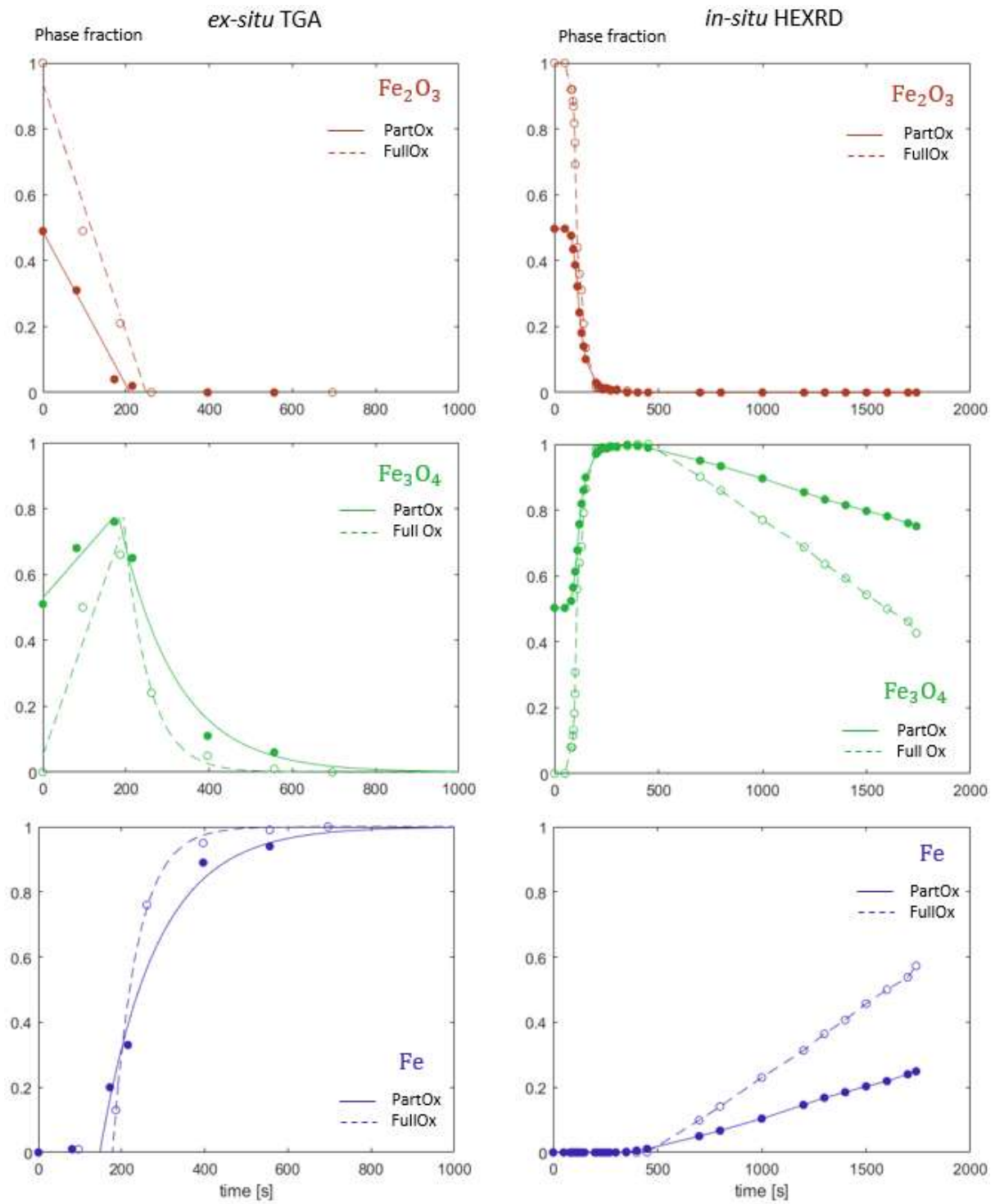
3 Figure 6 Phase evolution of individual phases in PartOx and FullOx samples during hydrogen-based 4 direct reduction at 500°C, investigated by ex-situ X-ray diffraction (XRD) at various reduction levels in 5 interrupted thermogravimetry analysis (TGA), and by in-situ high-energy X-ray diffraction (HEXRD).
