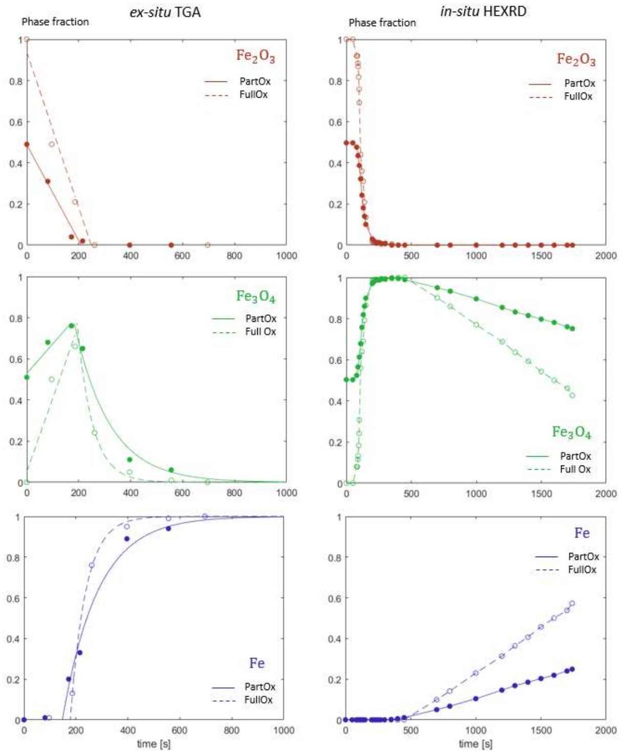
Figure 3 Phase evolution of individual phases in PartOx and FullOx samples during hydrogen-based direct reduction at 500°C, investigated by ex-situ X-ray diffraction (XRD) at various reduction levels in interrupted thermogravimetry analysis (TGA) experiments, and by in-situ high-energy X-ray diffraction (HEXRD).
