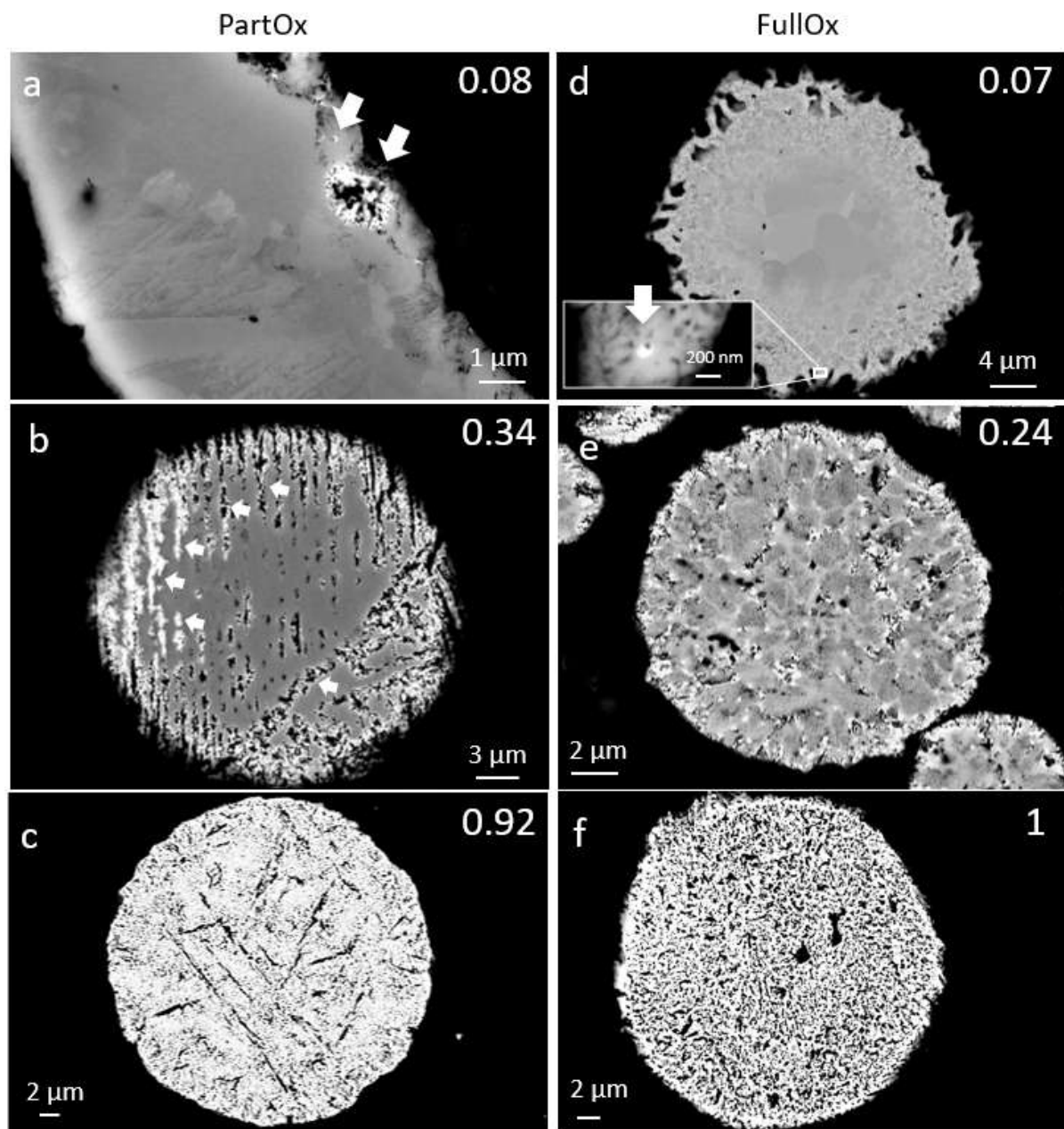
3 Figure 4 Scanning electron microscopy (SEM) images with backscattered electrons detector 4 presenting the cross-section of partially reduced particles of (a-c) PartOx and (d-f) FullOx 5 powders during their reduction at 500°C in the thermogravimetry (TG) reactor, with their 6 average reduction level estimated from XRD measurements given in the top right corner. The 7 white arrows highlight the presence of porous \alpha -iron grains.
