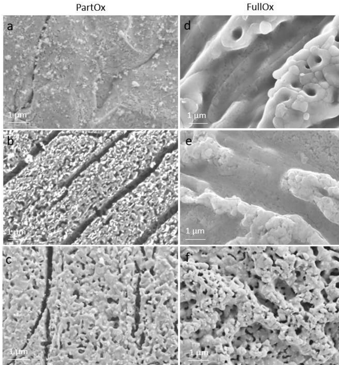
Figure 7 Scanning electron microscopy (SEM) images with secondary electrons contrast of the evolution of the surface morphology of (a-c) PartOx and (d-f) FullOx powders during their reduction at 500°C in the thermogravimetry (TG) reactor, for a reduction level of (a) 0.08, (b) 0.34, (c) 0.92, (d) 0.07, (e) 0.24, and (f) 1.
