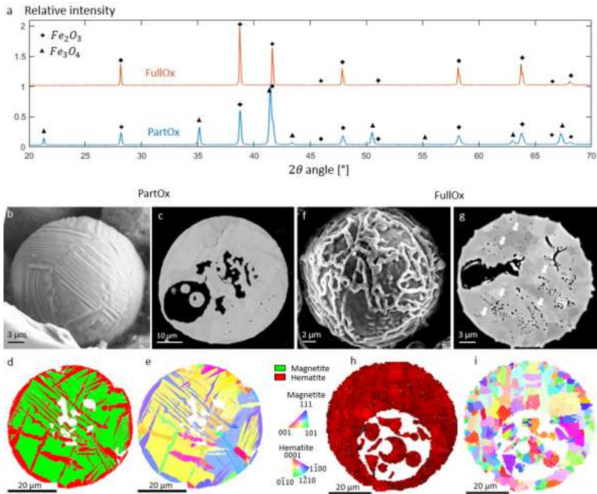
Figure 5 Microstructural characterization of the combusted iron particles, prior to the reduction process: (a) X-ray diffraction (XRD) analysis (with a Co target); (b-e) combusted powder (PartOx) and (f-i) combusted powder subjected to an additional deep pre-oxidation treatment (FullOx). (b, f) Scanning electron microscopy (SEM) image of the surface, with secondary electrons contrast, and (c, g) of the cross section of a particle, with backscattered electrons contrast. (d, h) Electron backscatter diffraction (EBSD) phase map and (e, i) crystalline orientation map. The arrows in (g) highlight the additional porosities formed during the deep pre-oxidation treatment.
