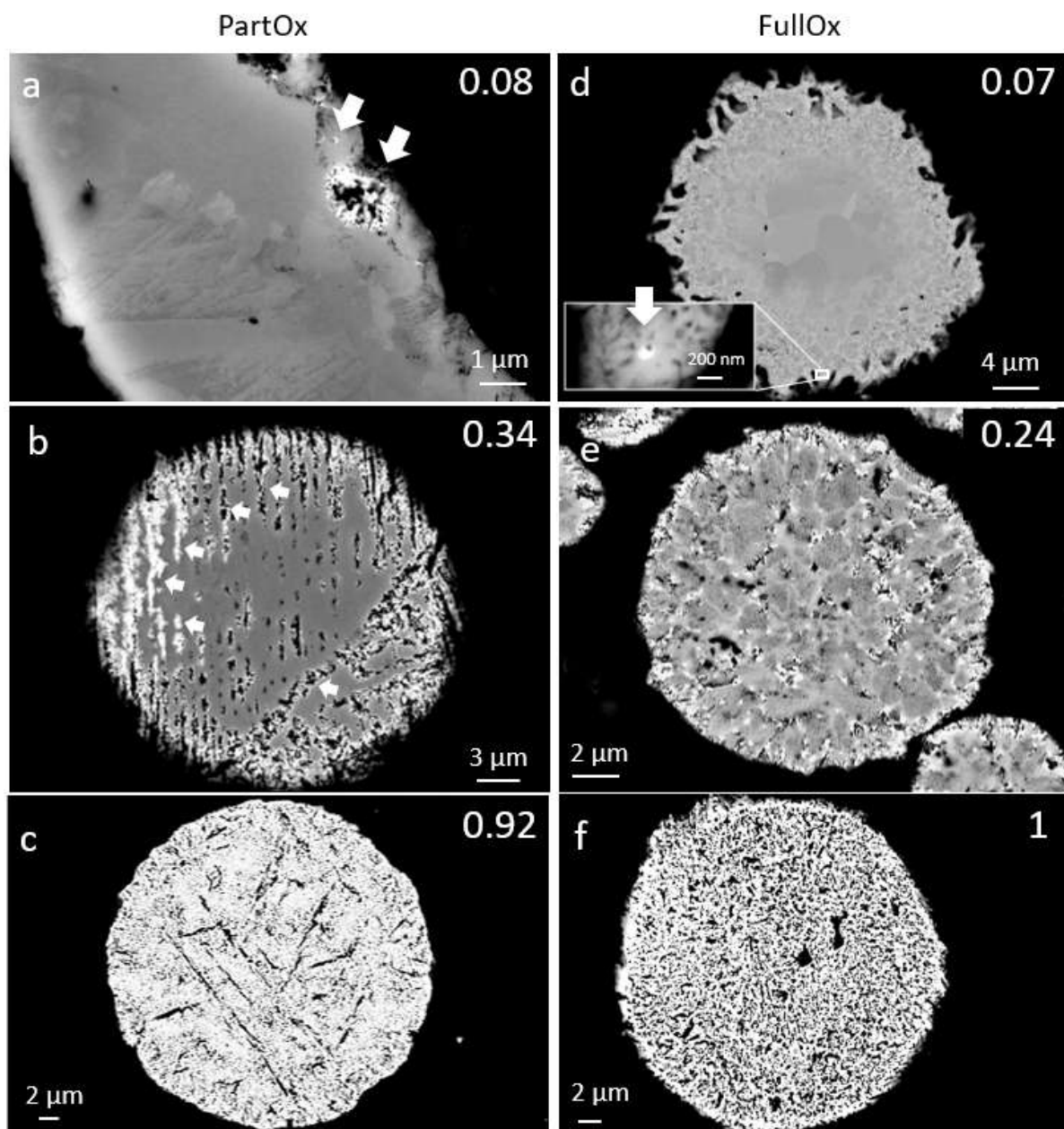
Figure 4 Scanning electron microscopy (SEM) images with backscattered electrons detector presenting the cross-section of partially reduced particles of (a-c) PartOx and (d-f) FullOx powders during their reduction at 500°C in the thermogravimetry (TG) reactor, with their average reduction level estimated from XRD measurements given in the top right corner. The white arrows highlight the presence of porous \alpha -iron grains.
