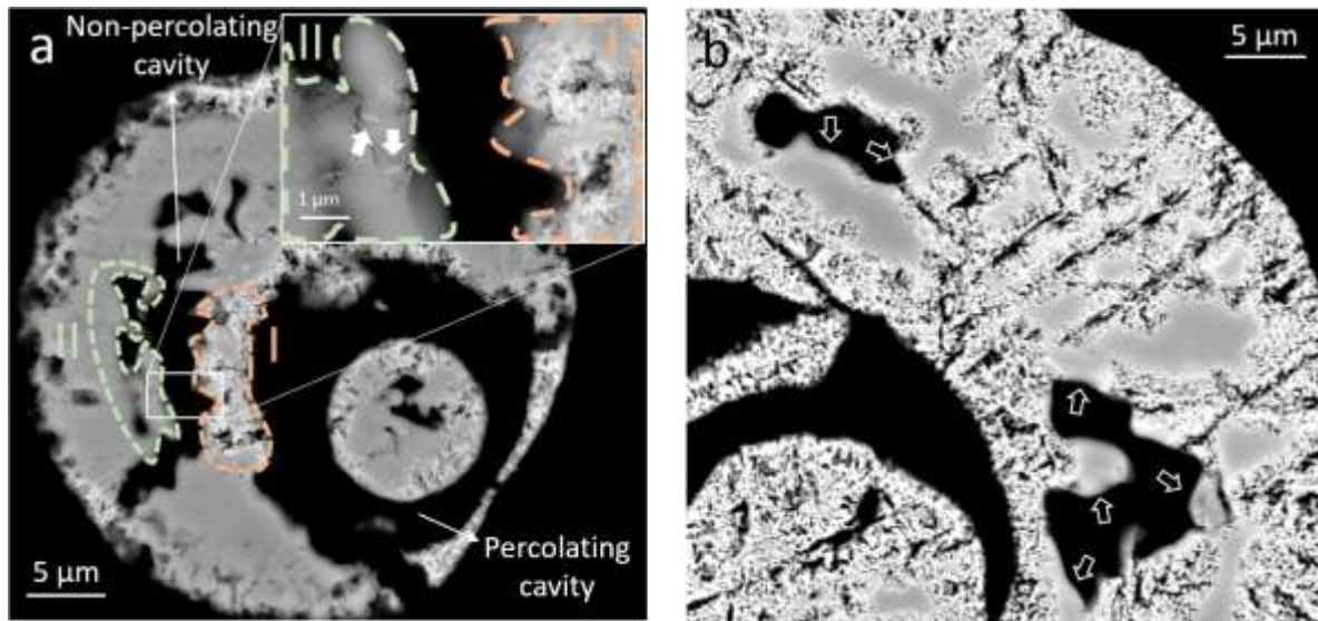
Figure 6 Influence of the porosities on the reduction process. Scanning electron microscopy (SEM) images with backscattered electrons contrast of the cross-section of PartOx particles, partially reduced in the thermogravimetry (TG) reactor at 500°C at a reduction level of (a) 0.32 and (b) 0.92. The white arrows highlight the presence of \alpha -iron in the inset of (a) and of remaining magnetite near the porosities in (b).
