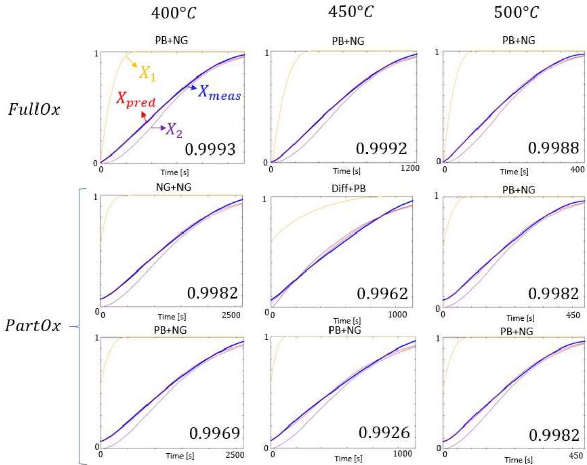
Figure 9. Multi-model fitting the total conversion X using Equation (11) and the models listed in Table 1 for X_1 and X_2 . The graphics presenting the best goodness of fit, given in the bottom-right corners, are presented. The abbreviations PB, NG and SD correspond to a phase boundary, nucleation and growth, and 3D solid diffusion model, given as the models representing X_1 and X_2 , respectively. The multi-models considering a phase boundary for X_1 and a nucleation and growth model for X_2 for PartOx are also given for all temperatures, for sake of comparison.
