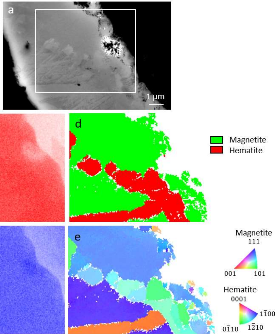
Figure 5 Electron backscatter diffraction (EBSD) and energy dispersive spectroscopy (EDS) maps of a PartOx particle partially reduced to a reduction level of 0.08 in the thermogravimetry (TG) reactor at 500 °C. (a) The corresponding scanning electron microscopy (SEM) image, (b) oxygen and (c) iron EDS map, (d) EBSD phase map, and (e) EBSD inverse pole figure (IPF) related to the sample normal direction.
