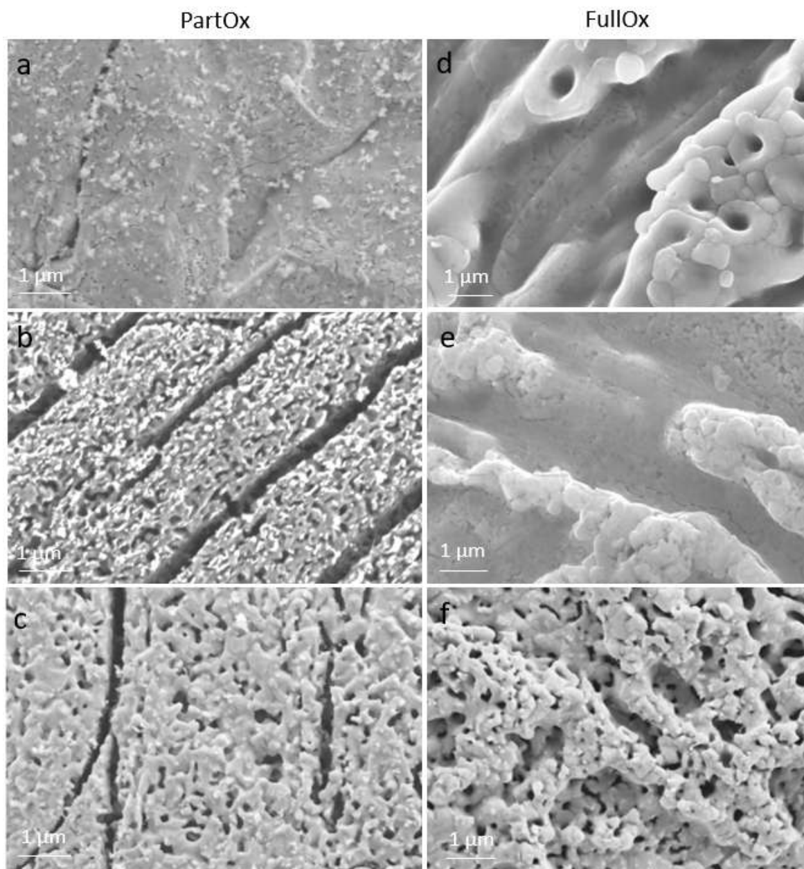
Figure 7 Scanning electron microscopy (SEM) images with secondary electrons contrast of the evolution of the surface morphology of (a-c) PartOx and (d-f) FullOx powders during their reduction at 500°C in the thermogravimetry (TG) reactor, for a reduction level of (a) 0.08, (b) 0.34, (c) 0.92, (d) 0.07, (e) 0.24, and (f) 1.
