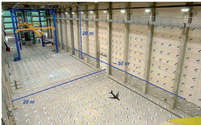
Figure 5 - B20 catapult facility with a very large transport aircraft model.
