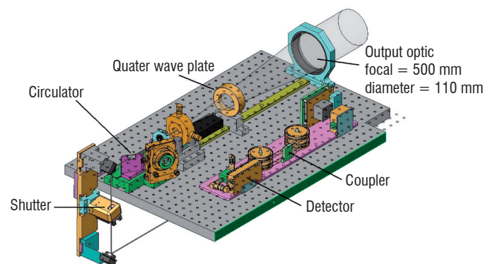
Figure 16 - Lidar optical layout.
