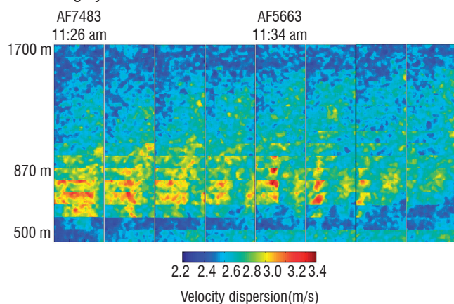
Figure 18 - Velocity dispersion images, calculated by UCL, obtained for 8 successive scans of 16 range gates of 75m after the passing of two successive aircraft. Each box represents the 12^\circ \times 3^\circ field of view image acquired at different ranges (vertical axis) and at different times (horizontal axis).
