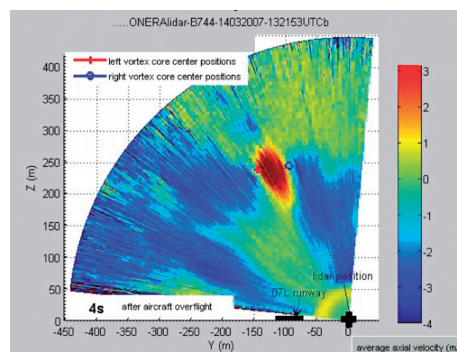
Figure 14 - Example of average velocity map display. The core positions are post processed. This shows the first measurement of a B747-400 on March 14th. This is a movie (Click on it to run).
