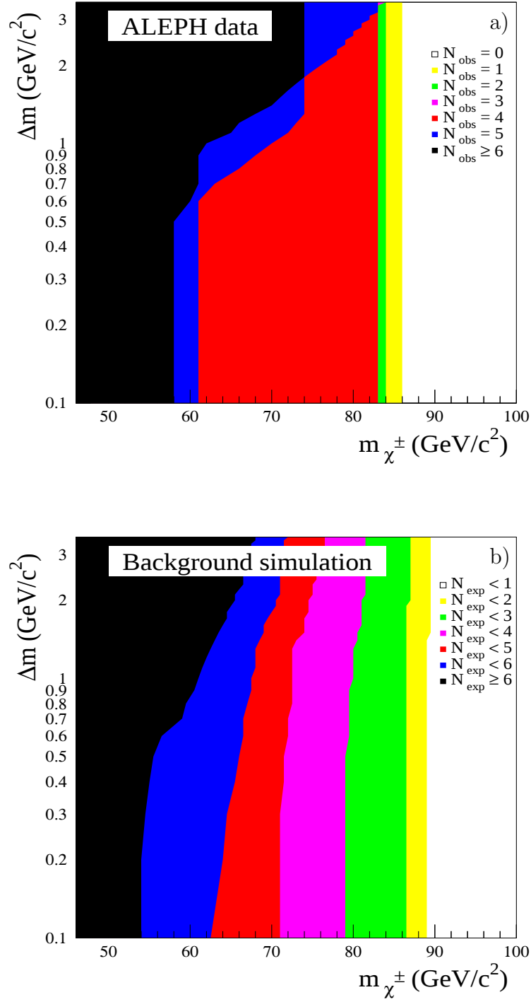
Figure 2: Number of events a) observed and b) expected from standard background sources in the (m_{\chi^\pm}, \Delta m) plane. The number of events decreases for large chargino masses or low \Delta m due to the tightening of the cuts on the transverse missing momentum and on the total energy not associated with the reconstructed photons. No events compatible with m_{\chi^\pm} > 86 \text{ GeV}/c^2 are observed in the data.
