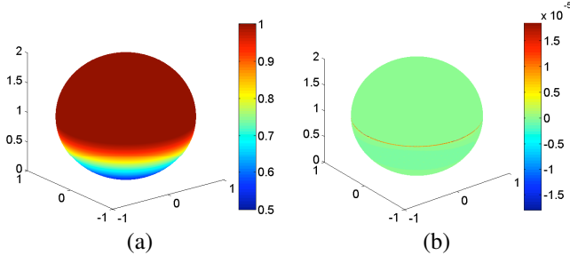
Figure 1: (a) The graph of the function f(\theta, \varphi) defined in (4); (b) Its analysis with the spherical wavelet associated to the Daubechies wavelet db3, the familiar 6-coefficient filter.
