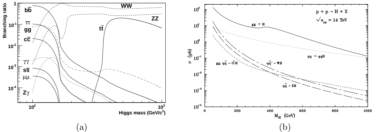
Figure 1: (a) Next-to-leading order (NLO) calculations for the Standard-Model Higgs boson branching ratios from HDECAY 1 ; (b) NLO cross-section calculations for the Standard-Model Higgs boson at LHC 2 .
