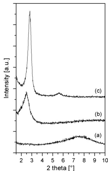
Fig. 2. XRD patterns at small angle of (a) the PW12-C18 hybrid, (b) the PW4-C18 hybrid and (c) the pure C18 copolymer matrix.
