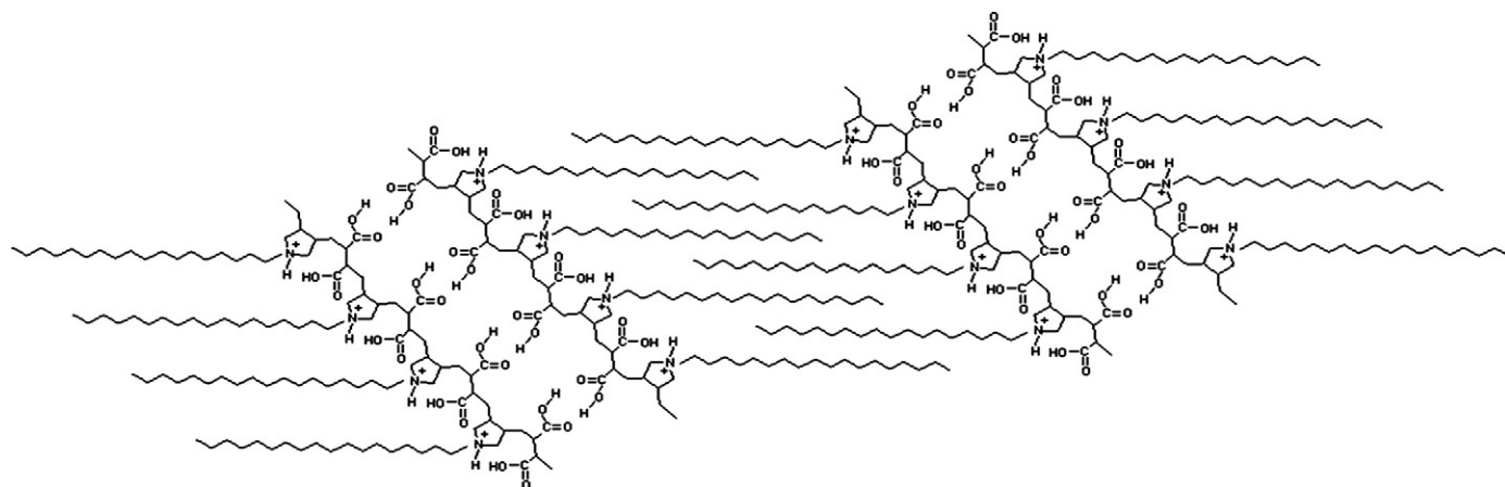
Scheme 1. Scheme of the supramolecular organization of the self-assembled amphiphilic poly(ampholytic) copolymer (inspired from [13]).
