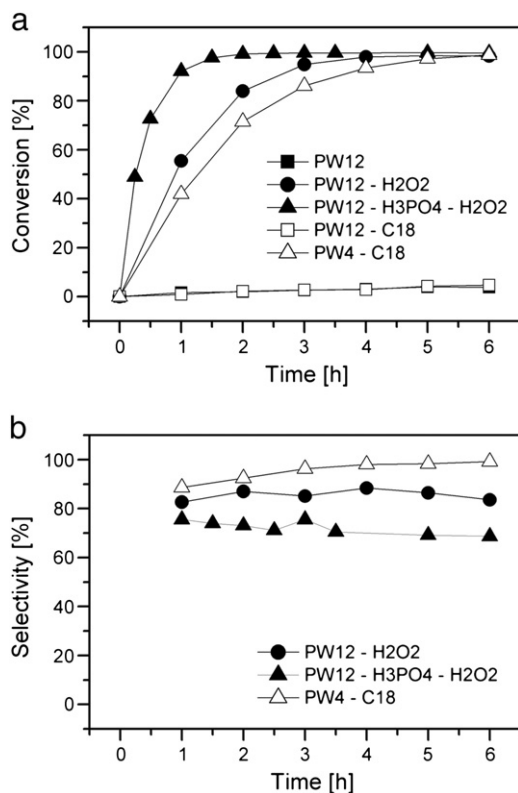
Fig. 3. Catalytic performance of homogeneous and hybrid catalysts for cyclooctene epoxidation in CH 3 CN. A better conversion is obtained for homogeneous catalysts (a) but PW4 hybrid catalyst presents a higher selectivity in epoxycyclooctane (b).
