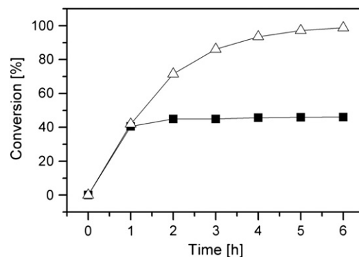
Fig. 4. Hot catalyst filtration experiment on hybrid for cyclooctene epoxidation. (Δ) Conversion without recovery and (■) test with catalyst recovery after 1 h by centrifugation and filtration.
