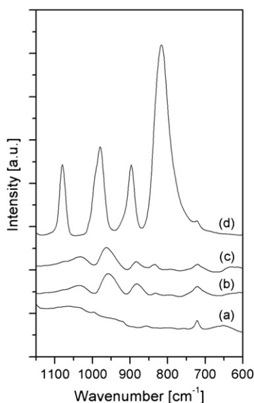
Fig. 1. IR spectra of hybrid materials in the low frequency region of polyoxometalate species: (a) the pure C18 copolymer matrix, (b) the PW4-C18 hybrid, (c) the PW4-C18 hybrid recovered after four catalytic tests and (d) the PW12-C18 hybrid.
