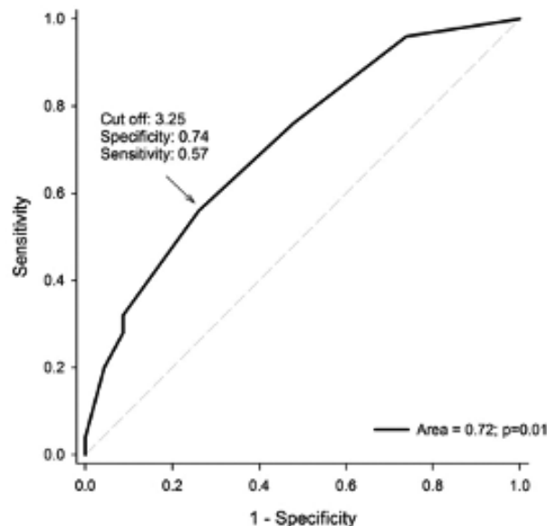
Figure 3. — ROC curve of KLIC score (all PJI).
