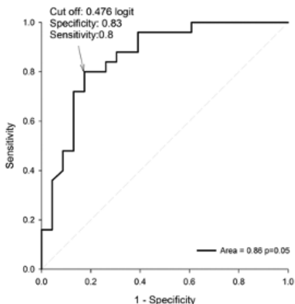
Figure 2. — ROC curve of equation 1.
