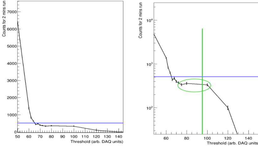
Figure 4.44. | The number of coincidences in the PMT as a function of the threshold. The left panel displays the count axis in linear scale, while the right panel depicts it in logarithmic scale for enhanced visibility of the plateau.
