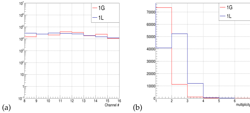
Figure 4.52. | (a) Distribution of occupancy for prototype 1.L (depicted in blue) and prototype 1.G (represented in red). (b) Distribution of multiplicity for both prototypes 1.L and 1.G. [161]
