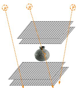
Figure 5.1. | In scattering muography, the object under investigation is "sandwiched" between muon trackers.
