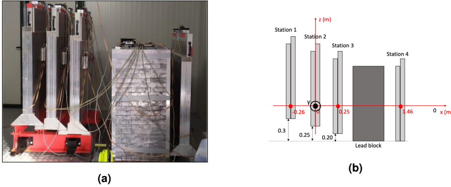
Figure 3.3. | (a) One of the MURAVES hodoscopes. (b) A schematic view of the reference frame of the MURAVES hodoscopes.
