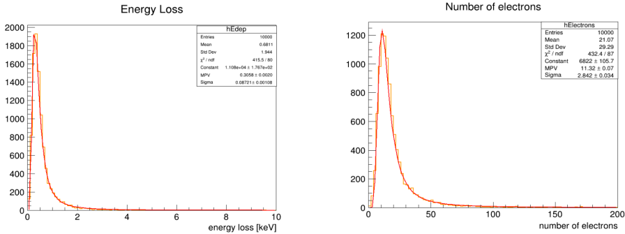
Figure 4.59. | Energy loss (left) and number of electron (right) caused by muon interaction within a 1mm thick gas.
