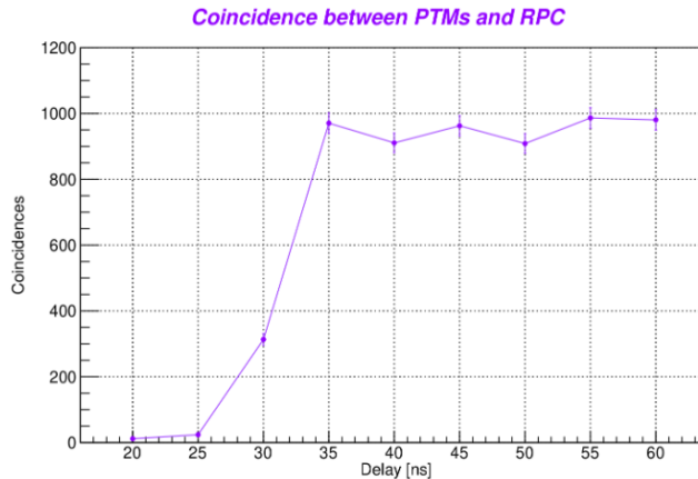
Figure 4.46. | Count of coincidences at various RPC signal delay values.
