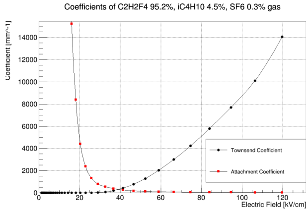
Figure 4.60. | Townsend and Attachment Coefficients for the CMS gas mixture.
