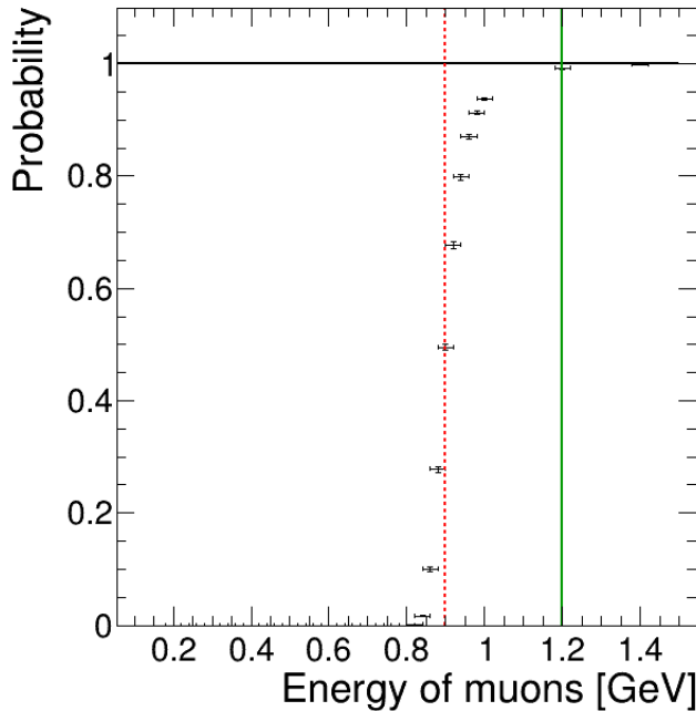
Figure 3.19. | Probability for a muon to survive the passage through the lead wall, as a function of its energy.
