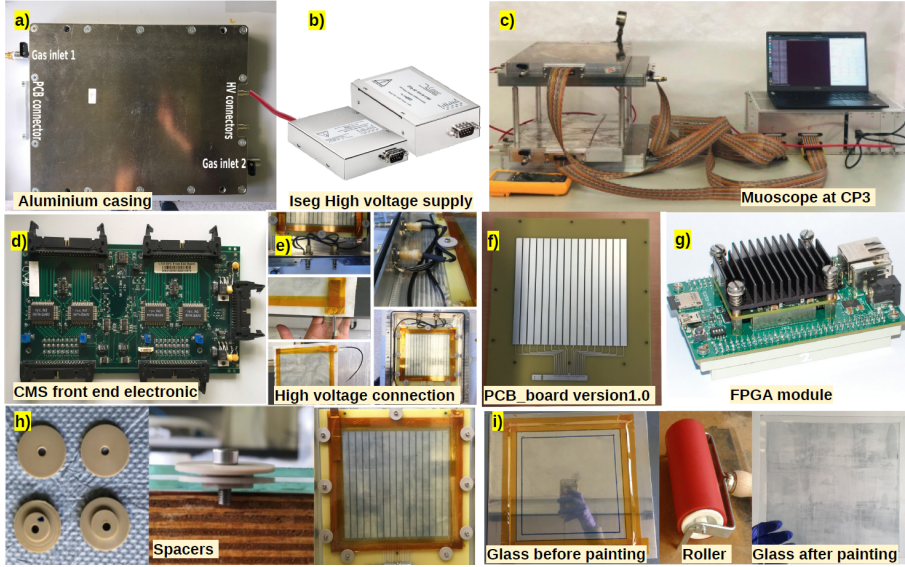
Figure 4.3. | Experimental setup elements [127]. a) Aluminium casing. b) Iseg high voltage supply. c) Muoscope at CP3/UCLouvain with DAQ. d) CMS front end electronic board. e) High voltage connection. f) Version 1.0 readout board. g) FPGA module. h) Round spacers. i) Resistive coating.
