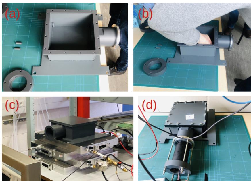
Figure 4.6. | Assembly process of the external trigger.
