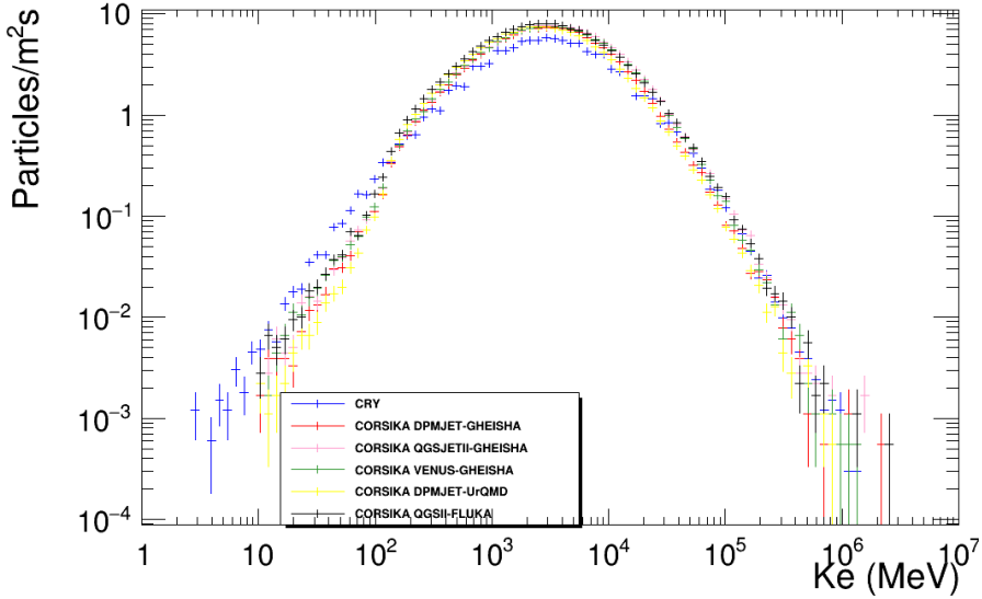
Figure 2.1. | Muon energy distribution obtained through CRY and five different hadronic interaction models in CORSIKA [93].
