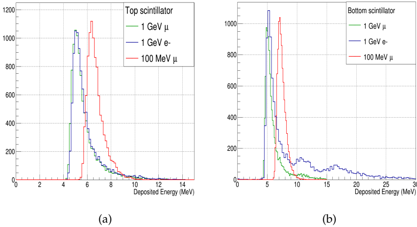
Figure 5.12. | Deposited energy in two scintillators installed at the top and at the bottom of our current prototype, for muons of 100 MeV (red) and 1 GeV (green) and electrons of 1 GeV (blue) that cross our current prototype. Simulated with GEANT4.
