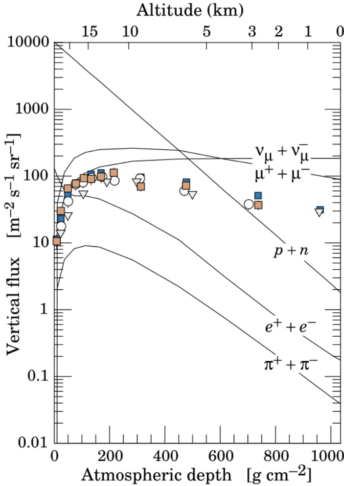
Figure 1.2. | Vertical fluxes of various particles, for momenta larger than 1 GeV. Points correspond to measurements of the vertical flux of negative muons only, with different symbols corresponding to different experiments [10].
