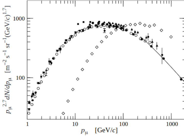
Figure 1.3. | Spectrum of muons at \theta = 0^\circ ( \circ, \bullet, \blacksquare, \blacktriangledown, \times, + ) and \theta = 75^\circ ( \diamond ) [10]. The line plots the result from eq 1.9 for vertical showers.
