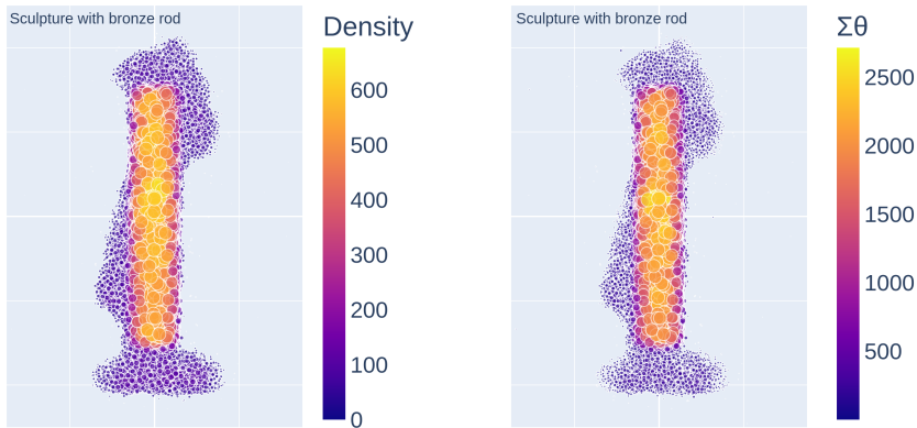
Figure 5.7. | Using Neighborhood Sum clustering algorithm (orange: hidden bronze bar, magenta: wood statue), taking as input only the POCA positions (left) and also the scattering angles (right).
