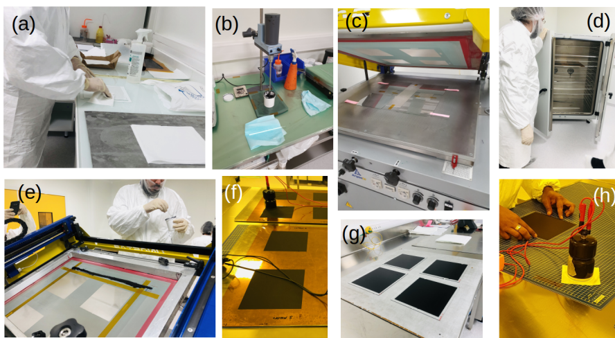
Figure 4.23. | Steps involved in producing the resistive plate using the serigraphy method.
