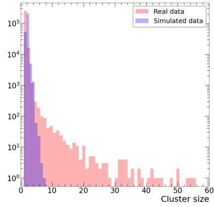
Figure 3.27. | Comparison of the sizes of the clusters involved in the selected tracks ( \chi^2 < 5 ) for real and simulated data.
