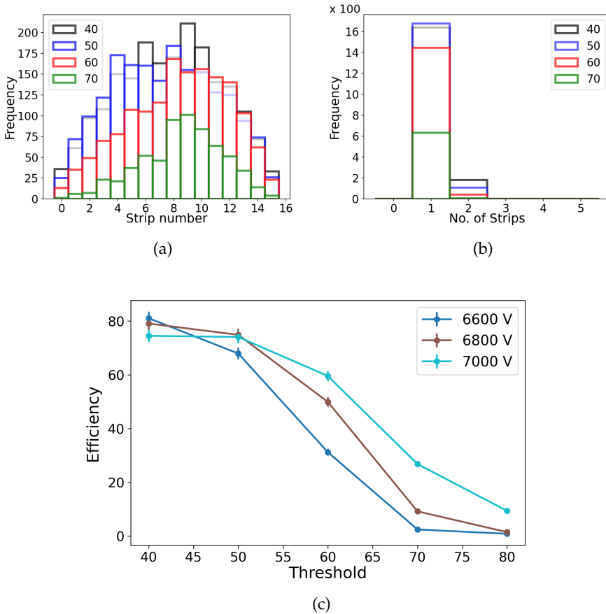
Figure 4.55. | The obtained measurements illustrate (a) occupancy and (b) multiplicity, conducted at an HV of -7 kV with varying threshold values (in DAQ units); (c) illustrates the efficiency variations with respect to thresholds at three distinct working points.
