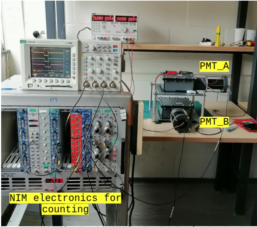
Figure 4.12. | Setup for the calibration for the control voltage.
