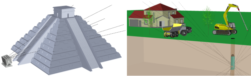
Figure 1.11. | The geometry of the detector in absorption muography depends on the application, left: scan of a large open-air structure (e.g. a pyramid), right: borehole application for underground imaging. From [31].
