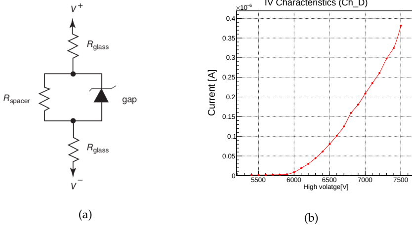
Figure 4.56. (a) Electrical circuit equivalent to an gRPC. At low voltage levels, the gas multiplication processes are negligible, resulting in a high gas resistance ( R_{\text{gap}} \sim \infty ) and a voltage-current relationship dV/dI = 2R_{\text{glass}} + R_{\text{spacer}} . Conversely, at high voltage levels, the gas resistance R_{\text{gap}} \sim 0 leading to a dV/dI = 2R_{\text{glass}} (b) Ohmic behavior of one of our gRPC.
