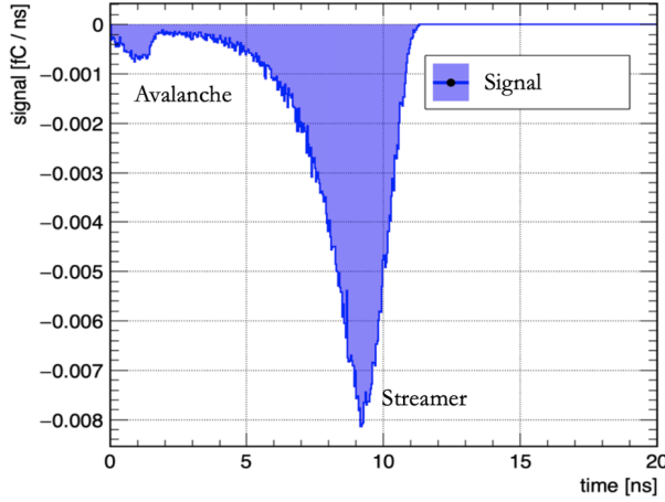
Figure 4.63. | Signal showing the Avalanche and Streamer Modes.
