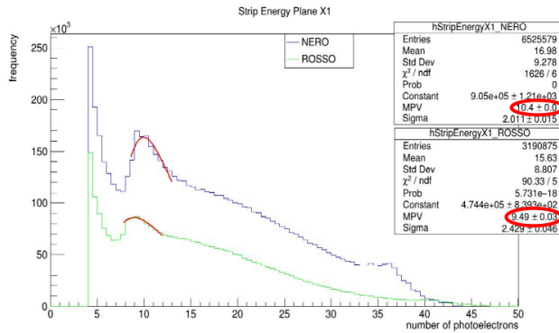
Figure 3.24. | Energy deposition distribution per bar in plane 1X based on the data obtained from NERO and ROSSO detectors.
