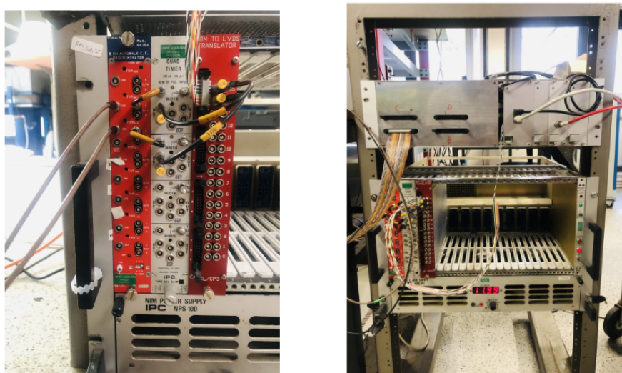
Figure 4.16. | Three modules employed to integrate the external trigger to the DAQ system (left). The electronic setup of the DAQ system with the integrated external trigger (right).
