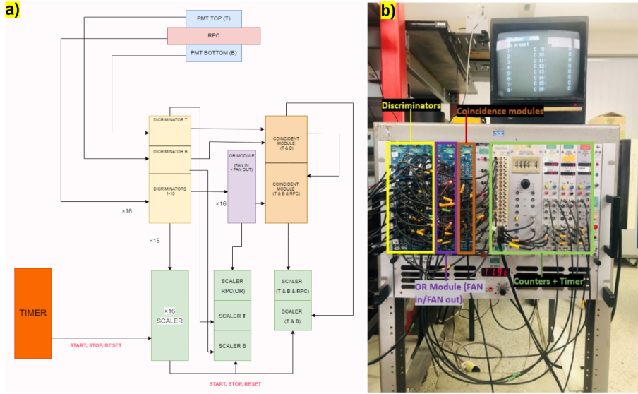
Figure 4.39. (a) Sketch for the setup. (b) NIM crate setup.
