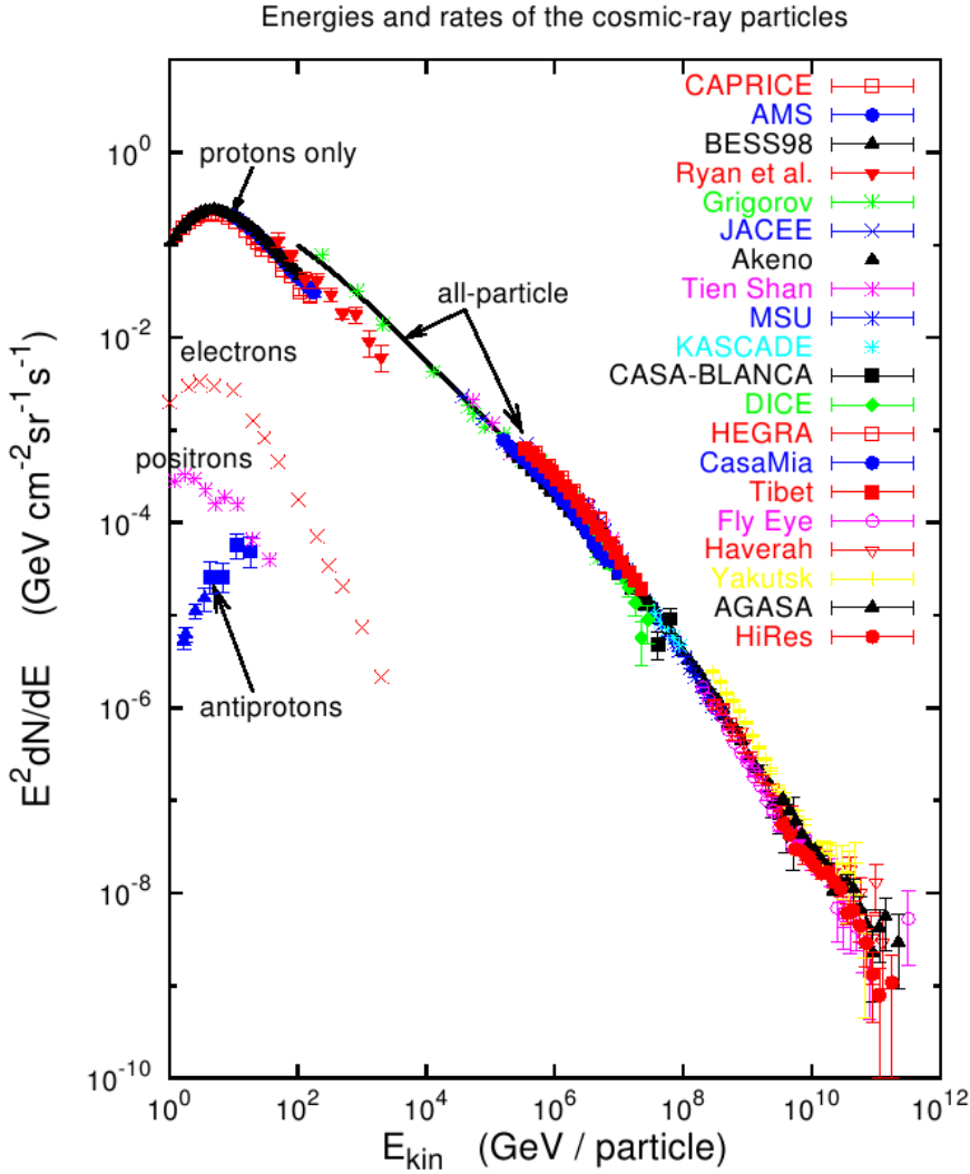
Figure 1.1. | The intensity spectrum of cosmic rays extends over more than ten orders of magnitude in energy with a smooth spectrum I(E) \sim E^{-2.7 \dots 3.0} . Figure from [6]
