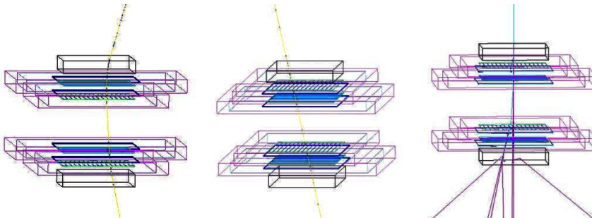
Figure 2.8. | Simulation with GEANT4 of the passage of a 48 MeV muon (left), a 1 GeV muon (centre) and a 1 GeV electron (right) with the addition of two plastic scintillator slabs. Muons are in yellow, electrons in blue and photons (from bremsstrahlung) in pink.
