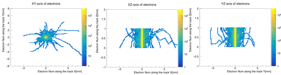
Figure 4.58. | Electron trajectory within the gas gap from different view.
