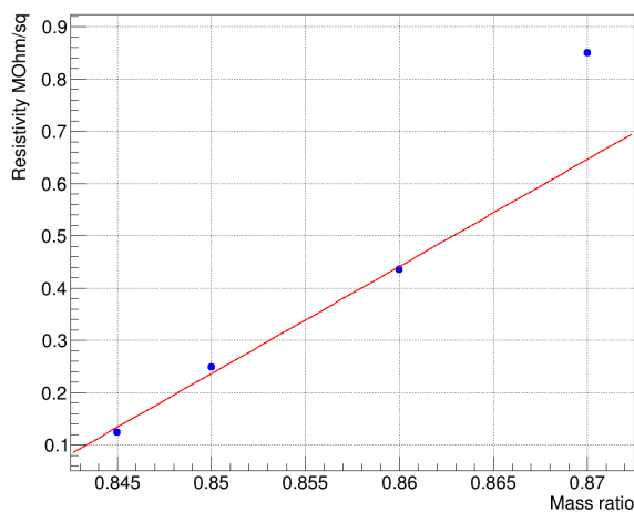
Figure 4.30. | Surface resistivity plotted against mass ratio. Experimental data points are represented by blue dots, and the red line indicates the linear fit, expressed by the equation R = 20.5 \cdot r_c - 17.2 .
