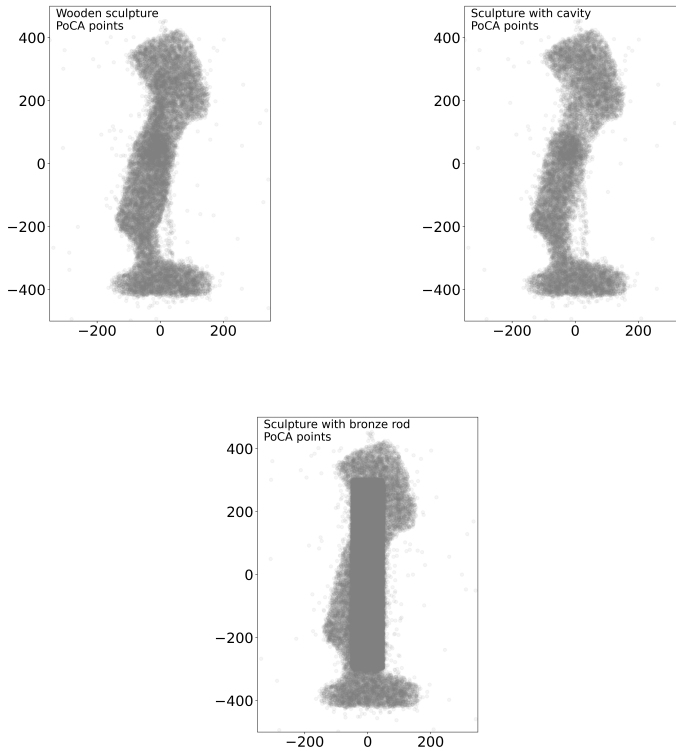
Figure 5.5. | Distribution of POCA points, projected to a 2D plane for clarity, in three simulated scenarios: (left) actual wooden sculpture, (middle) with a cylindrical cavity, (right) with a cylindrical bronze rod.
