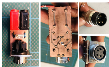
Figure 4.8. | (a) Potentiometer board and banana connectors (colored in red and black) along with a DIN female connector, (b) Rear view of the board, (c) DIN 4 male connector, (d) 71251-040/0800 DIN female connector.
