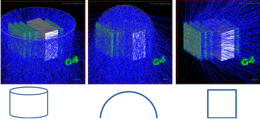
Figure 2.2. | The three EcoMug modes: cylindrical (left), hemispheric (center) and flat (right) generation surfaces, here shown interfaced to the GEANT4 model of the MURAVES hodoscope described in section 3.2.
