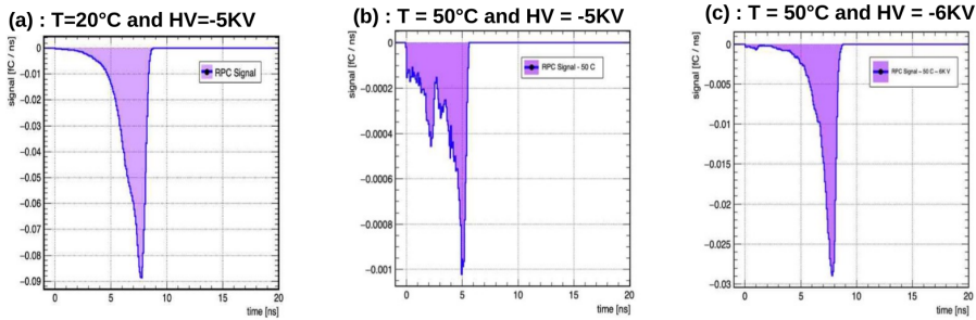
Figure 4.64. | Observing RPC signals under varying temperatures and voltages.
