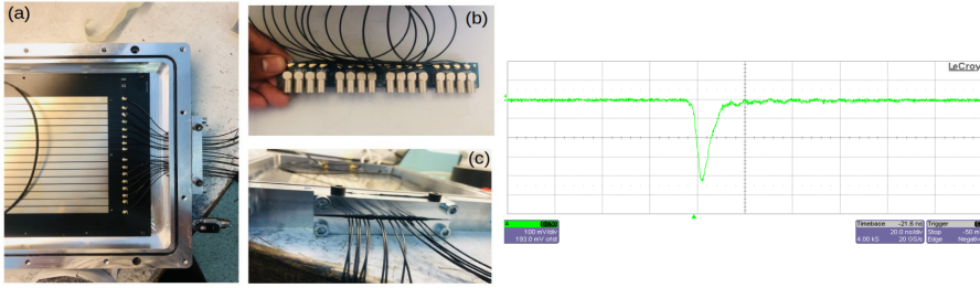
Figure 4.37. | Left: (a) Readout board inside the Chamber. (b) Board with 50 \Omega NIM standard female connectors. (c) New sealing "piece" for RPC. Right: RPC observed signal with HV = -7.2KV.
