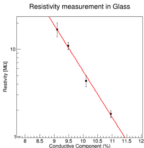
Figure 4.22. | Surface resistivity plotted against the conductive component of the paste. The black data points were utilized for fitting, producing the continuous red line represented by the equation R = 13.94 \cdot e^{-1.22} .
