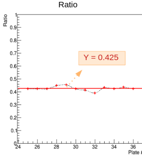
Figure 4.21. | The graph illustrates the measured ratio between R_{s_2} and R_{s_1} for different glass plates, with a corresponding fitting line corresponding to y = 0.425 .
