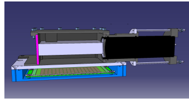
Figure 4.5. | The housing cross-section for the trigger scintillator, with the plastic scintillator represented by the white box.
