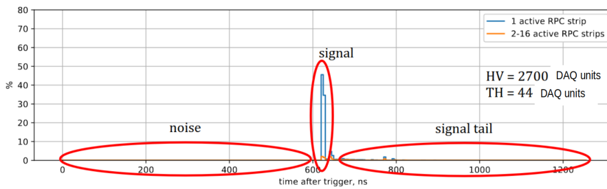
Figure 4.53. | Noise, signal and signal tail of the RPC. The Y-axis denotes the efficiency with respect to the PMT trigger.
