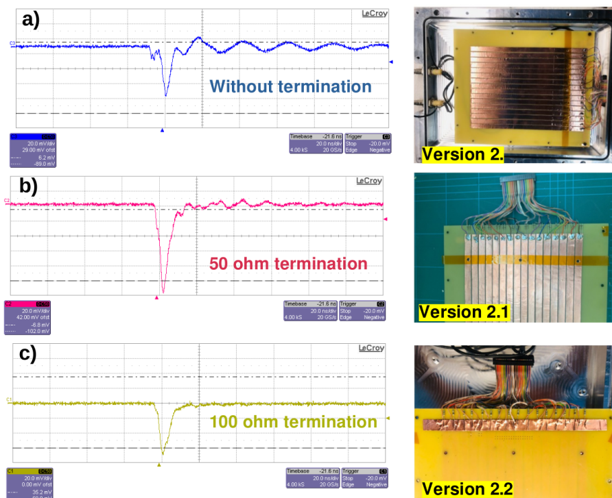
Figure 4.35. | RPC signal observed from each readout board with a 7.2KV applied high voltage.
