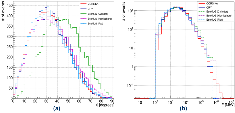
Figure 2.3. | Distributions of zenith angle \theta (a) and kinetic energy E (b) generated using CRY, CORSIKA and three EcoMug modes (corresponding to flat, cylindrical and hemispherical generation planes).
