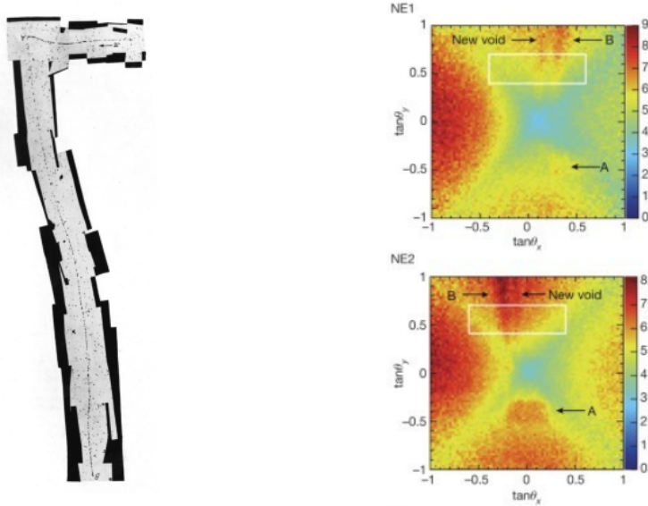
Figure 1.12. | Left: Photomicrographs of one example of pion decay into muon taken from [4], Right : Muograph of the Khufu pyramid obtained by using nuclear emulsion detector (A: King’s chamber, B: Grand Gallery), reproduced from [39].
