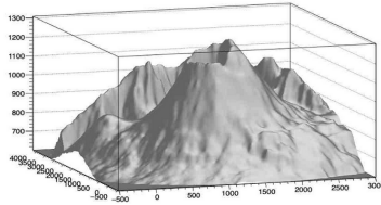
Figure 3.17. | Digital terrain model of Vesuvius crater. Based on data from [111].
