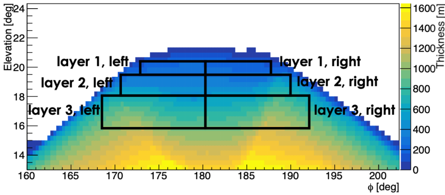
Figure 3.15. | Definition of the angular regions utilized for the first measurement of density projection asymmetries. Reproduced from Ref. [110].
