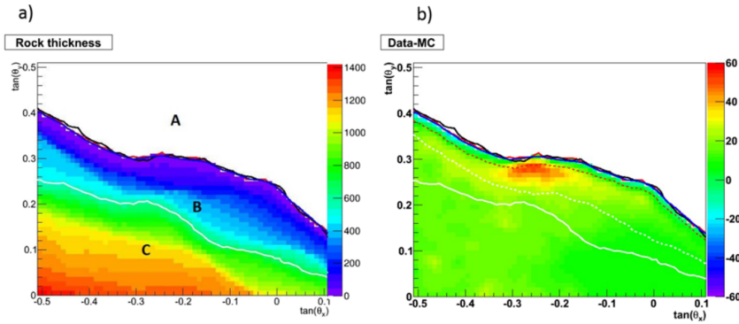
Figure 1.7. (a) Visualization of rock thickness and the Stromboli's crater profile captured by the emulsion detector. The color scale illustrates rock thickness in meters. (b) Representation of the discrepancy between the observed muon flux and the flux predicted by Monte Carlo simulation within an angular range centered on the crater region. The color scale indicates muon counts. Variables \theta_x and \theta_y represent azimuthal and elevation angles, respectively. "Region A" corresponds to the open sky, while "Regions B and C," separated by a white line (indicating the sensitivity limit based on Monte Carlo simulations assuming zero background), define the accessible muography area and the "deep rock" region (unreachable by muography). The sensitivity limit corresponds to an anticipated flux of 2.3 muons (90% confidence level, assuming zero background) per 20 \times 20 \text{ mrad}^2 bin (equivalent to approximately 10 \times 10 \text{ m}^2 projected at the crater). Reproduced from [53].
