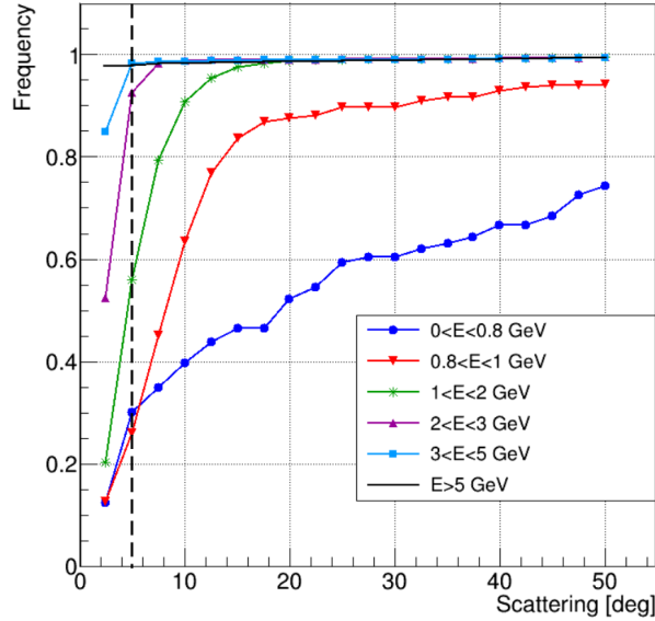
Figure 3.20. | Efficiency of various possible upper cuts on the scattering angle for different ranges of incoming muons energy.
