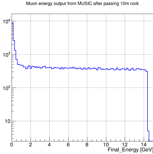
Figure 2.6. | Energy of muons after passing through a 10m rock in MUSIC code.
