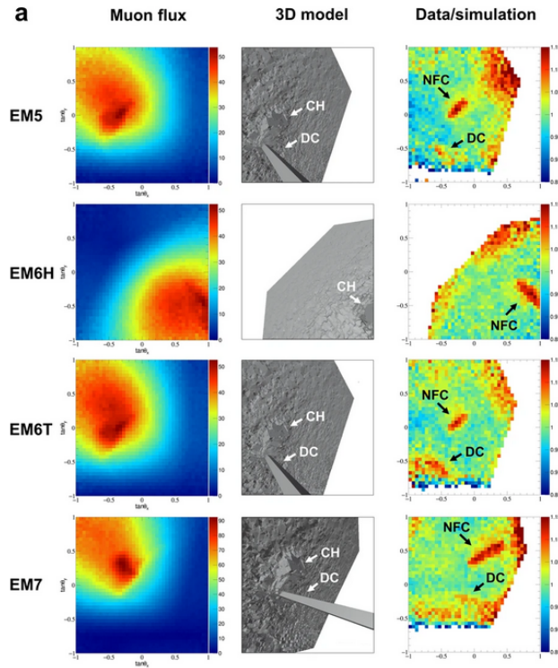
Figure 1.5. | Two-dimensional angular distribution for EM5 to EM7. (★) From left to right: observed muon flux ( \text{tracks}/\text{cm}^2/\text{day}/\text{sr} ), 3D model, ratio of muon flux of the data to simulation. Adapted from [40].
