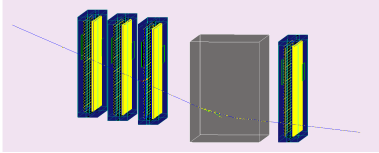
Figure 2.7. | Interaction of a 1 GeV muon with one of the MURAVES hodoscopes in GEANT4.
