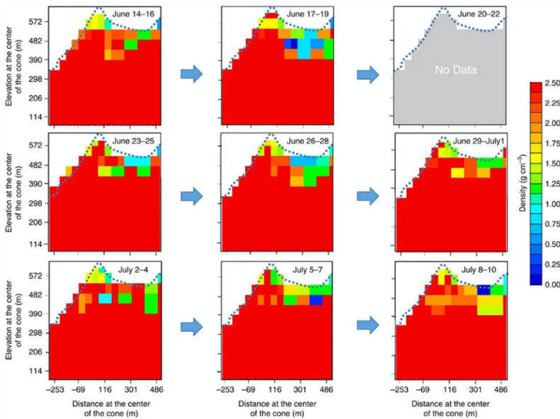
Figure 1.6. | The dynamics of magma during the Satsuma-Iwojima eruption are illustrated in the diagrams. These visual representations depict the angular distribution of the upper limit of the average density along the muon path at a 1\sigma (68% Confidence Level). The frame rate consists of 10 frames per month. It's important to note that data collection was interrupted from June 20 to 22 due to a blackout. To enhance statistical precision, two horizontally adjacent bins were combined. The figures also provide information on the elevation and horizontal distances from the center of the cone. From [49].
