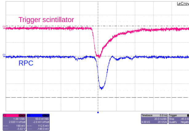
Figure 4.45. | The coincidence of signals between a single strip of the RPC and the scintillator, with a 50 ns delay introduced in the RPC signal using cables and a delay module.
