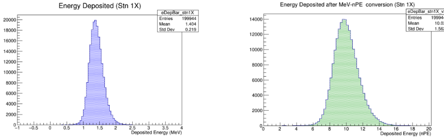
Figure 3.25. | Left: Simulated energy deposition (in MeV) before conversion, Right: Simulated energy distribution (in nPE) after conversion.
