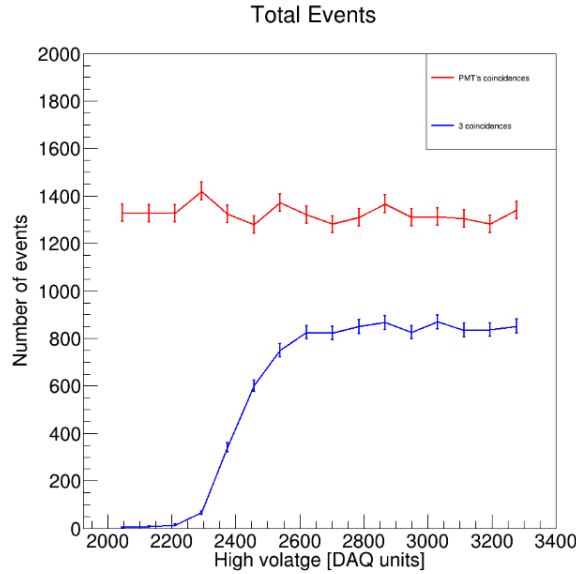
Figure 4.48. | Performance of RPCs (readout version 2.2, indicated in blue) and PMTs (shown in red) with supplied high voltage.
