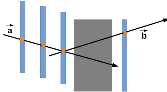
Figure 3.21. | Schema illustrating the scattering within the lead wall, where \vec{a} represents the vector created from hits in the first and third stations, and \vec{b} represents the vector formed from hits in the third and fourth stations.
