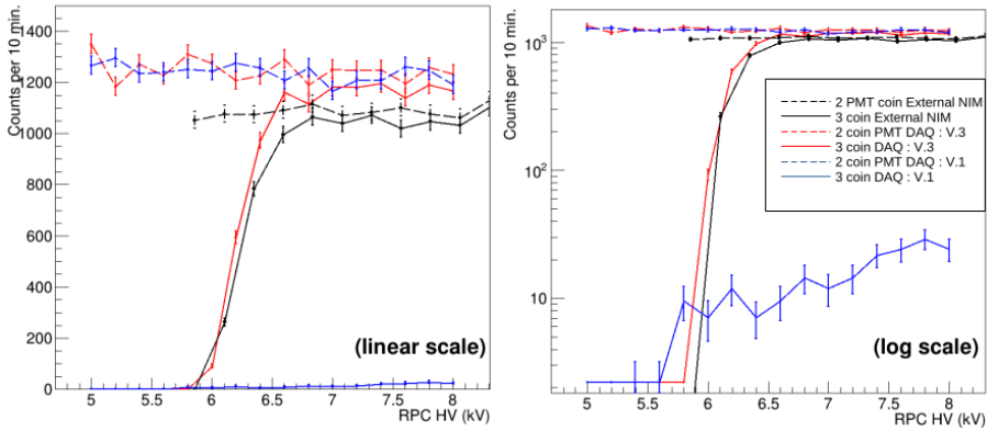
Figure 4.47. | Comparison of the performance of RPCs (readout version 1.0 in blue and version 3.0 in red) and PMTs with respect to the supplied high voltage using both external NIM electronics and DAQ. The data on the left are presented in linear scale, while the ones on the right are in logarithmic scale.
