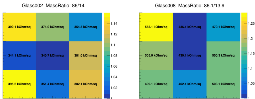
Figure 4.29. | Measurement of surface resistivity of two glass plates at 9 distinct locations, employing two different mass ratios.
