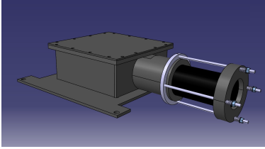
Figure 4.4. | Computer-aided design (CAD) representation showcasing the external appearance of the finalized external trigger setup.
