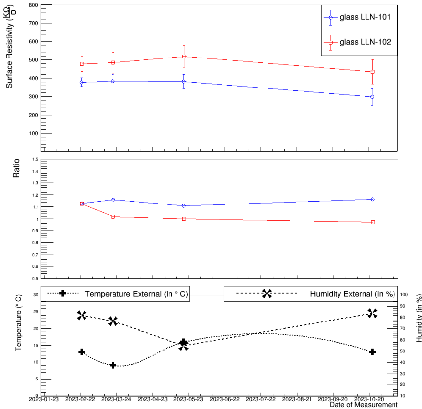
Figure 4.31. | Temporal evolution of key parameters: average surface resistivity of two selected glass plates (top), ratio between the resistivity at the center and the average resistivity of other locations on the same plate (middle), and external measurements of temperature and humidity (bottom).
