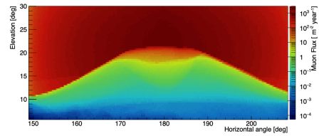
Figure 3.18. | Expected muon flux per year considering the geometrical acceptance of the detector, estimated with PUMAS.
