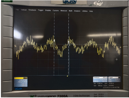
Figure 4.32. | Oscilloscope displaying a noise signal at a frequency around 144 MHz.
