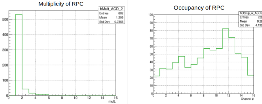
Figure 4.50. | Occupancy and multiplicity plots at -8 kV of high voltage.
