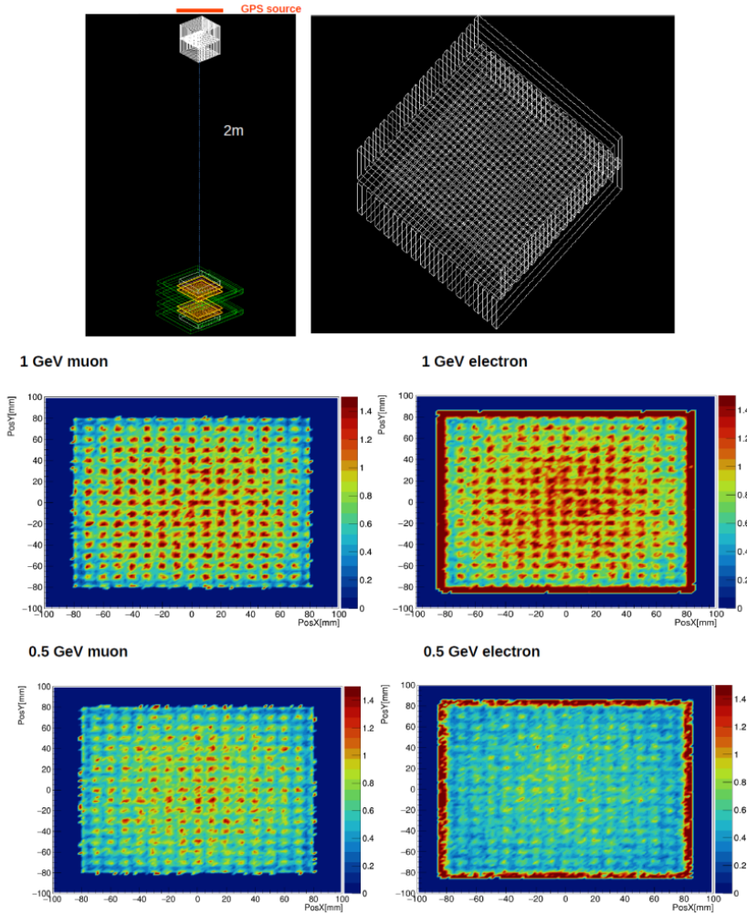
Figure 5.13. | GEANT4 simulation depicting the experiment with the current detector and an idealized 16 \times 16 \text{ cm}^2 marble structure within a vacuum environment. Top left: overall setup with muons and electrons generated from the 'GPS source' area (highlighted in red) covering the marble structure. Top right: detailed view of the marble structure, featuring orthogonal layers of 1 cm wide and 5 cm thick alternating marble strips. Bottom panels: Ratio of flux observed by RPCs after absorption and scattering through the marble structure, compared to free-sky flux, for 1 GeV (middle) and 0.5 GeV (bottom) muons (left) and electrons (right). The figures highlight the substantial impact of absorption and scattering on the electron flux, ignoring RPC spatial resolution.
