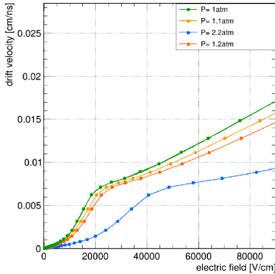
Figure 4.61. | Electron drift velocity in CMS gas mixtures for different pressure values. The temperature of the gas is T = 20^\circ .
