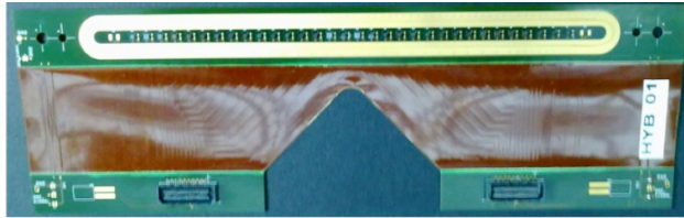
Figure 3.5. | Hybrid board with 32 SiPMs housed.
