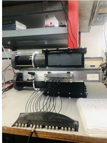
Figure 4.38. | RPC configuration setup.
