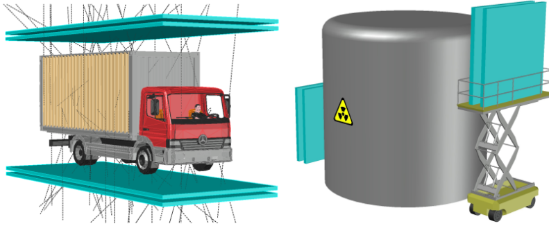
Figure 1.10. | Detector geometry depends on the application, left: cargo inspection, right: nuclear storage inspection. From [31].
