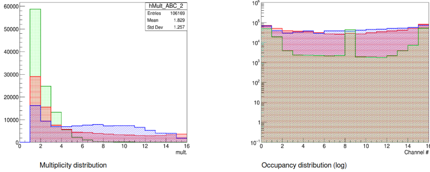
Figure 4.42. | The multiplicity and occupancy distributions of three distinct RPCs were examined in the RPC lab. The green plot corresponds to readout version 2.1 (refer to section 4.5.2), the blue plot corresponds to the RPC with readout board version 3.0 (refer to section 4.5.3), and the red plot represents the chamber with readout board Version 1.0 (refer to section 4.2).
