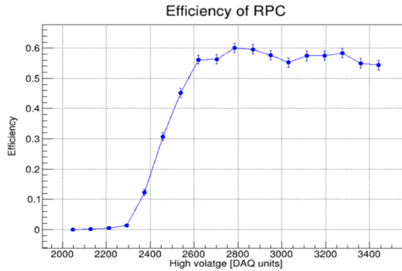
Figure 4.49. | Variation in efficiency of the RPC (readout version 2.2) with high voltage.
