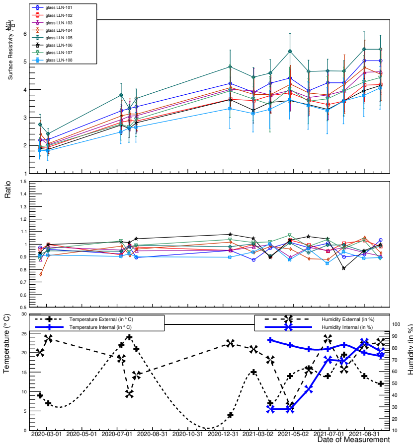
Figure 4.26. | Evolution of observables over time: Top: Average surface resistivity of eight selected glass plates with standard deviations at nine locations. Middle: Ratios of resistivity at the center to the average resistivity of other eight locations for each glass plate. Bottom: Temperature and humidity measurements from external weather data and internal Arduino-based sensor.
