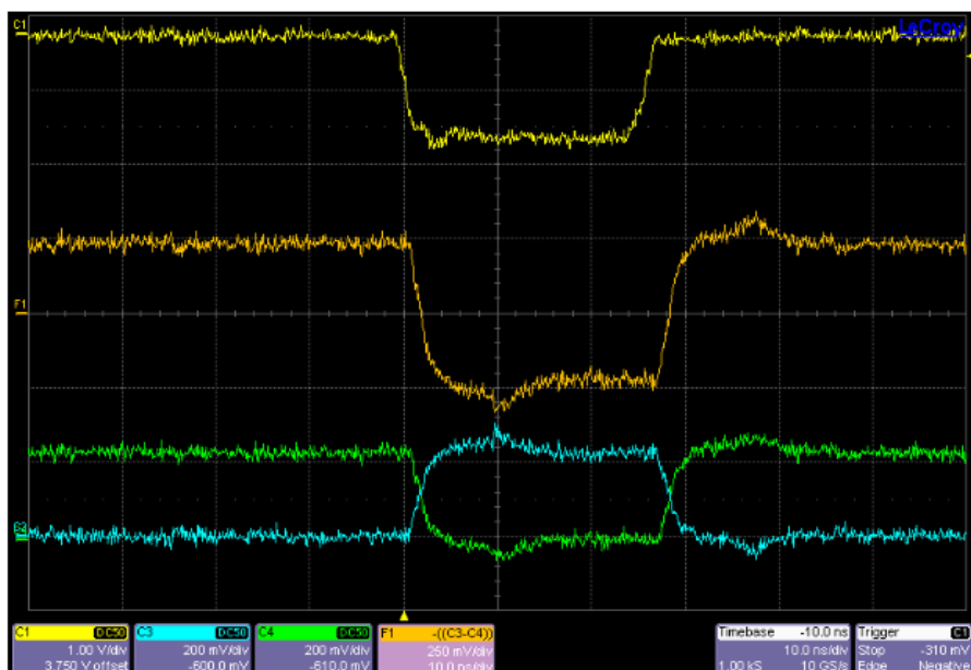
Figure 4.17. | Oscillogram of the LVDS output and monostable output. Channel 1 (yellow) represents the monostable output, while channels 3 and 4 (blue and green respectively) depict the outputs from two lines of the LVDS module.
