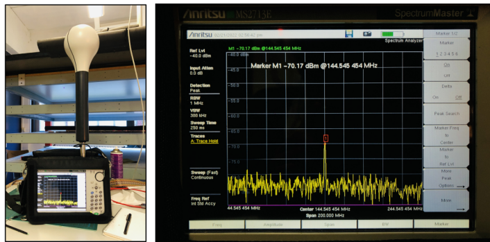
Figure 4.34. | Left: ANRITSU MS2713E spectrum analyzer [159]. Right: The screenshot of the spectrum analyzer screen in the RPC lab, displaying a signal at the frequency of 144.5 MHz.
