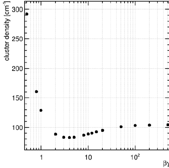
Figure 4.57. | Average clusters per cm as calculated by Heed++ for CMS gas mixture at 20° and 1.1 atm.
