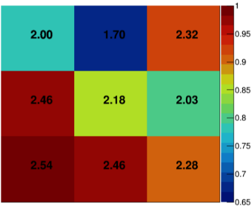
Figure 4.25. | Measurement of surface resistivity (in M\Omega/\square ) on one of the glass plates at 9 distinct locations. In the color code, a value of 1 corresponds to the highest value of surface resistivity.
