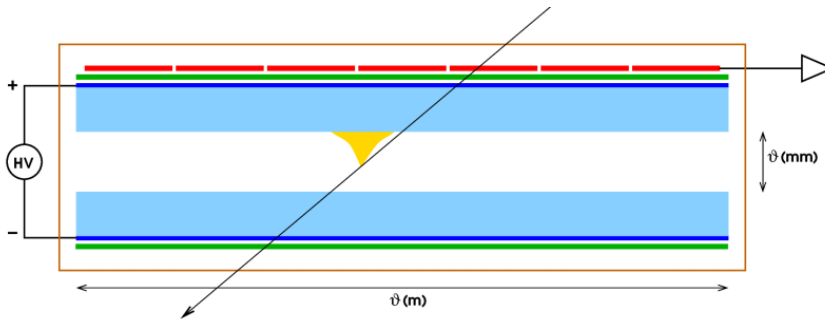
Figure 4.1. | Illustration of a single-gap RPC: The gas space is confined between resistive electrodes (light blue) coated with a semiconductive layer (dark blue) on their outer surfaces. These electrodes are protected by insulating layers above and below (green). When charged particles traverse the active area, they ionize the gas, triggering an avalanche effect (yellow) and generating a signal on the strips or pads of the readout board (red). From [126]
