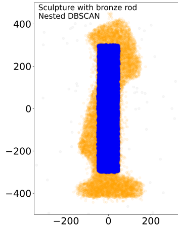
Figure 5.6. | Using DBScan clustering algorithm (blue: hidden bronze bar, yellow: wood statue).
