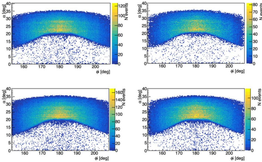
Figure 3.13. | Muon counts as a function of \alpha and \phi for the Vesuvius datasets for NERO (top row) and ROSSO (bottom row) in WP15 (left column) and WP20 (right column) [107].
