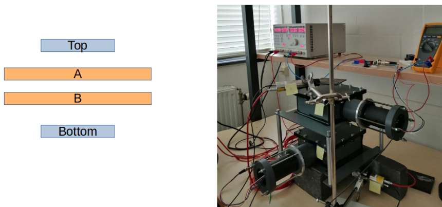
Figure 4.15. | Configuration of PMTs for evaluating the efficiency of the two scintillators.
