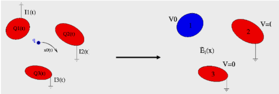
Figure 4.2. | Visualization of Ramo's theorem and the concept of the weighting field enables the calculation of the induced current on a grounded electrode caused by a charge q moving along a trajectory x_0(t) . Figure from [127].
