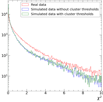
Figure 3.26. | Comparison of the \chi^2 of the tracks in real data and simulated data (the latter with and without clustering thresholds).
