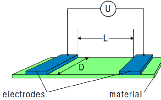
Figure 4.18. | Basic setup for surface resistance and surface resistivity measurement [157].
