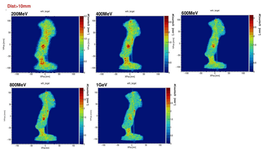
Figure 5.14. | 2D XY view after normalizing with respect to the traveled distance by muon for different energy beam (200-400-600-800-1000MeV).
