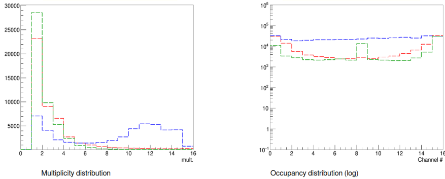
Figure 4.43. | The multiplicity and occupancy distributions of three distinct RPCs were examined in the CMS clean room. The green plot corresponds to readout version 2.1 (refer to section 4.5.2), the blue plot corresponds to the RPC with readout board version 3.0 (refer to section 4.5.3), and the red plot represents the chamber with readout board Version 1.0 (refer to section 4.2).
