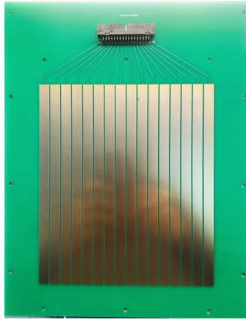
Figure 4.36. | Printed readout board with better quality copper and connection compatible with the DAQ with 110\Omega termination.
