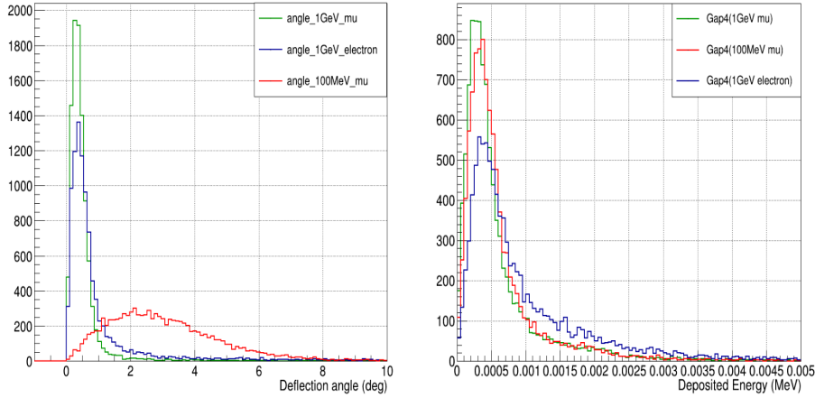
Figure 5.11. | Deflection angle with respect to the entry direction (left) and deposited energy in the gas gap of the last RPC (right) for muons of 100 MeV (red) and 1 GeV (green) and electrons of 1 GeV (blue) that cross our current prototype. Simulated with GEANT4.
