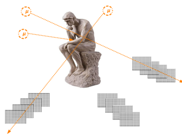
Figure 5.2. | In absorption muography, muon trackers are downstream of the object of interest; 3D imaging can be obtained by combining multiple viewpoints.
