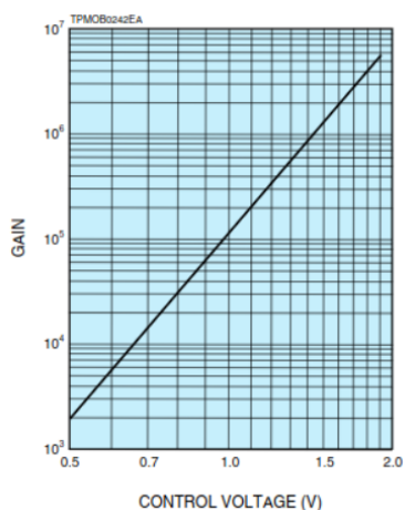
Figure 4.7. | The gain of the PMT with respect to the control voltage [149].
