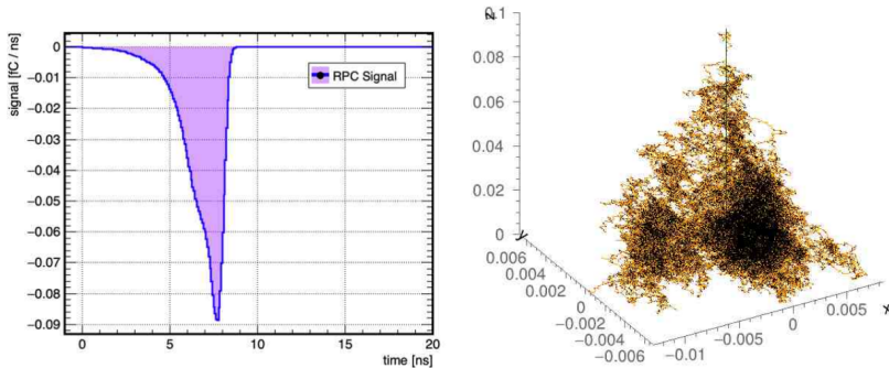
Figure 4.62. | Signal and Avalanche Electron Drift (in cm) in ambient conditions and 60 kV/cm.
