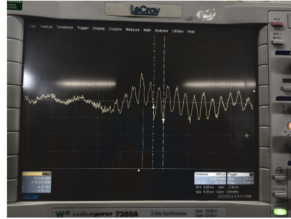
Figure 4.33. | Oscilloscope displaying a noise signal at a frequency around 433 MHz.
