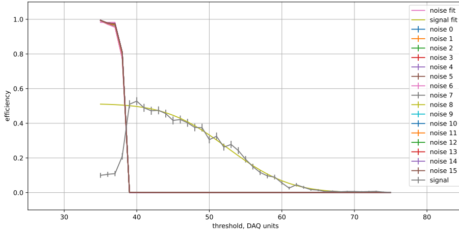
Figure 4.54. | Threshold scan for signal and noise in the RPC, the high voltage supplied for the RPC is -5.8 kV.
