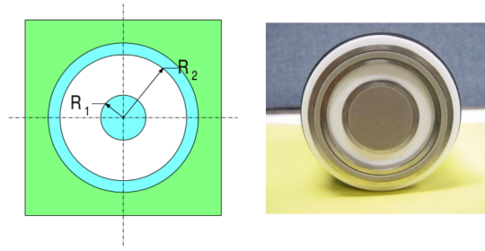
Figure 4.19. | Left: Configuration for measuring surface resistivity using concentric ring electrodes ( R_1 : Outer radius of the center electrode, and R_2 : Inner radius of the outer electrode). Right: Concentric ring probe. [157]
