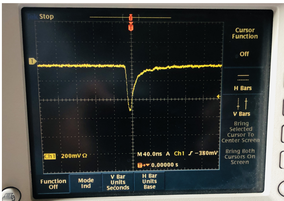
Figure 4.9. | Oscillogram showing the scintillator signal from the Top(A) PMT. The oscilloscope has an input impedance of 50\Omega , a voltage scale of 200 mV per square, and a time scale of 40 ns per square. The oscilloscope trigger is set at -380 mV.
