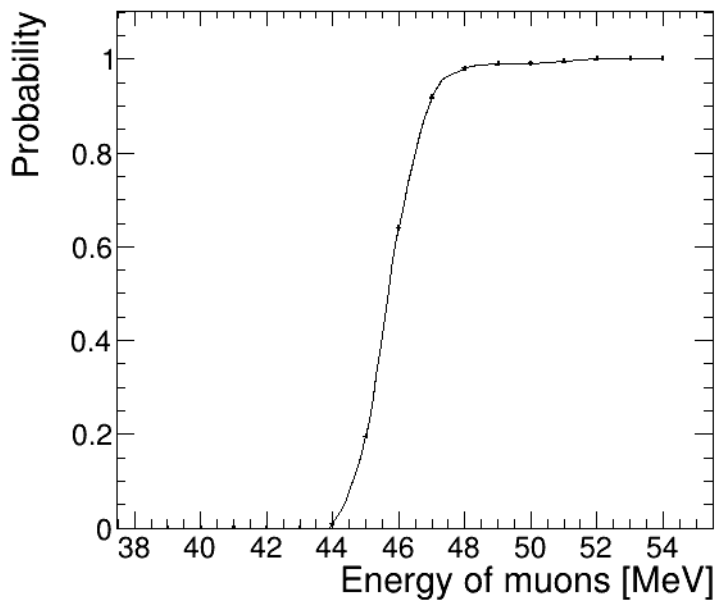
Figure 5.10. | Probabilty for a muon to survive the passage through our muoscope setup (see Figure 2.8), as a function of its energy.
