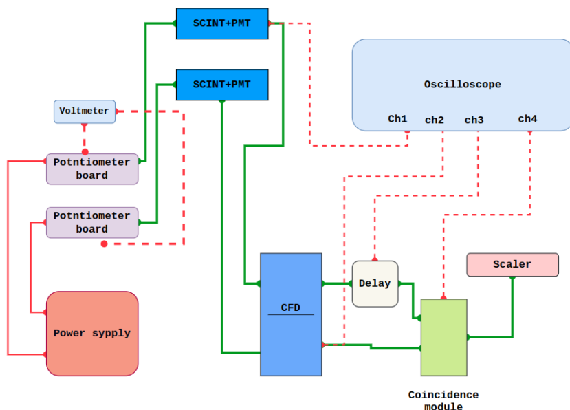
Figure 4.11. | Schematics of a coincidence circuit with two scintillator + PMT Setup.
