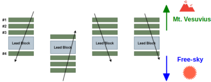
Figure 3.10. | Schematic illustrating the container layout.
