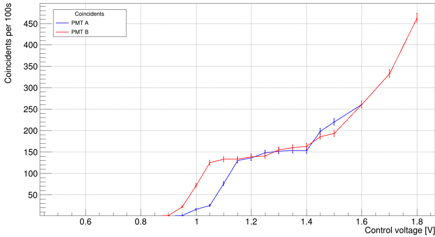
Figure 4.13. | The graph illustrates how coincidence counts for both PMTs change with respect to the control voltage. The plateau for PMT A (blue curve) falls within the range of 1.15 V to 1.4 V, while for PMT B (red curve), it extends from 1.05 V to 1.4 V
