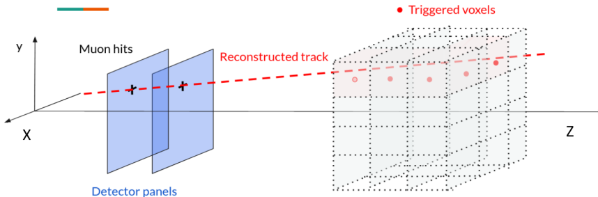
Figure 5.8. | Sketch for the back-projection algorithm.
