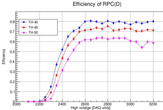
Figure 4.51. | High voltage scan for RPC (readout Version 2.2) at varying threshold values.
