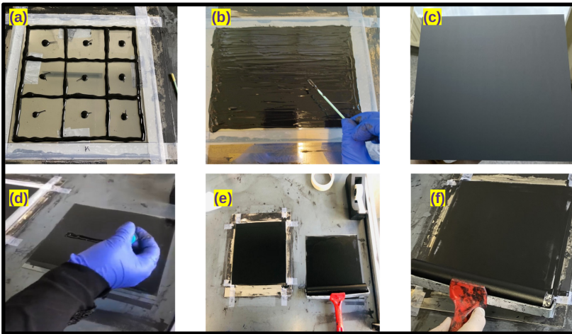
Figure 4.28. | (a) Depositing the first layer. (b) Spreading the paint on the plate using the sponge wand. (c) The plate after banking the first layer. (d) Pipping a couple of lines on a secondary plate. (e) Coating the roller with the secondary plate. (f) Coating the first plate with the wet roller.
