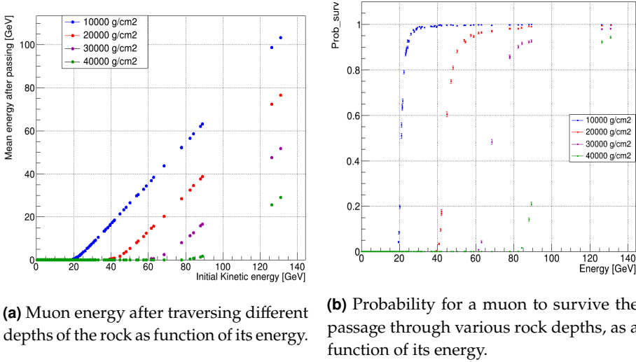
Figure 2.4. | Study with MUSIC of the muon interaction in different standard rock thickness ( \rho = 2.65 \text{ g/cm}^3 ), where CRY was employed as the primary muon generator.
