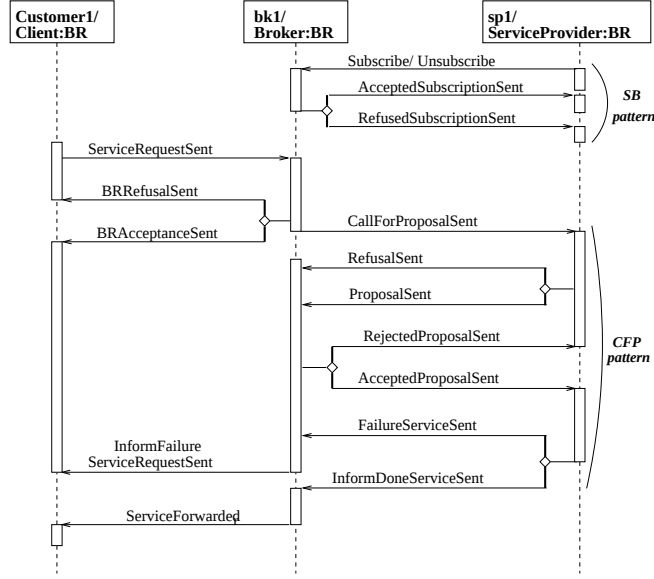
Figure 4: Communication Diagram - Broker
