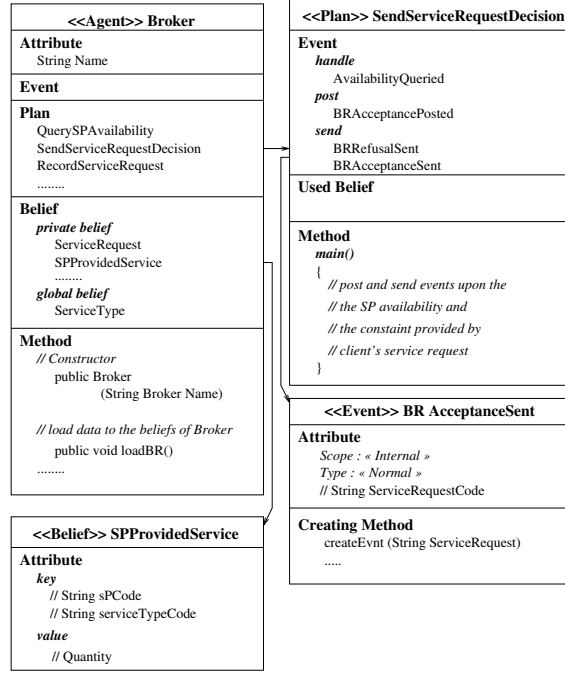
Figure 3: Structural Diagram - Some components of the Broker pattern
