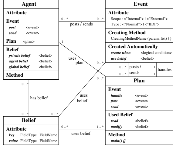
Figure 2: Structural Diagram Template
