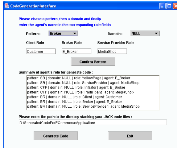
Figure 6: JACK Code Generation
