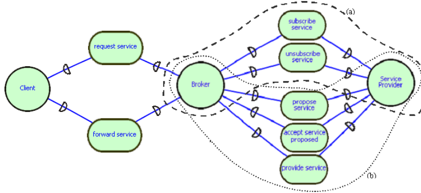
Figure 1: Social diagram for the Broker pattern
