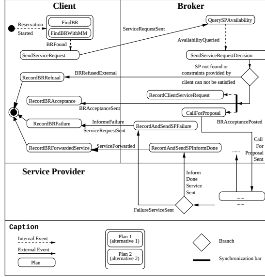
Figure 5: Dynamic Diagram - Broker
