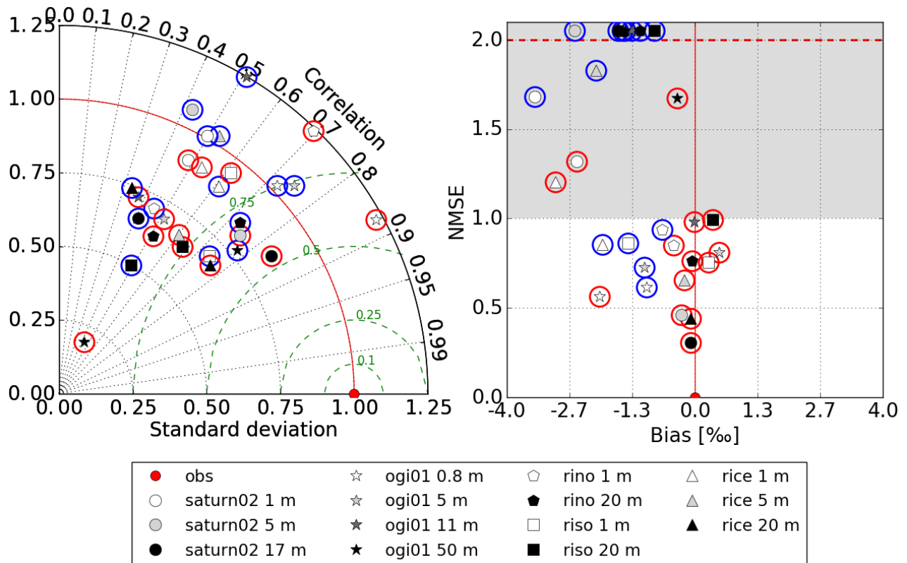
Figure 7: Normalized Taylor diagram (left) and NMSE versus bias (right) for SLIM 3D (red circles) and SELFE (blue circles) models outputs on the shelf for salinity. The grayscale of the markers indicate the depth: white is shallower, dark is deeper. In the Taylor diagram, normalized standard deviation is on the radial axis; correlation coefficient is on the angular axis; green dashed lines indicate NCRMSE. On the right panel, NMSE larger than 2 are placed just above the red dashed line irrespective of their values (see Table 2 for exact values). SLIM 3D skill is in general better than SELFE in terms of biases, NMSE and correlations.
