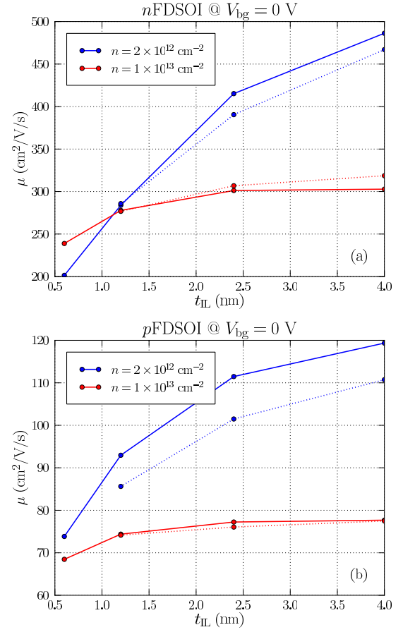
Fig. 5. Room-temperature (a) electron and (b) hole mobility as a function of t_{IL} , at two carrier densities n = 2 \times 10^{12} cm ^{-2} and n = 1 \times 10^{13} cm ^{-2} . The solid lines are the NEGF calculations, the dotted lines the experimental data.
