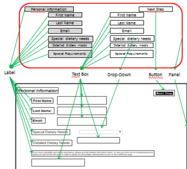
Figure 8. Mapping UI elements with concrete GUI widgets.
