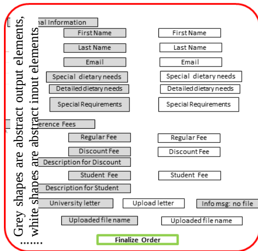
Figure 5. Outcome on the semantic level. “Finalize Order” is a task input element.
