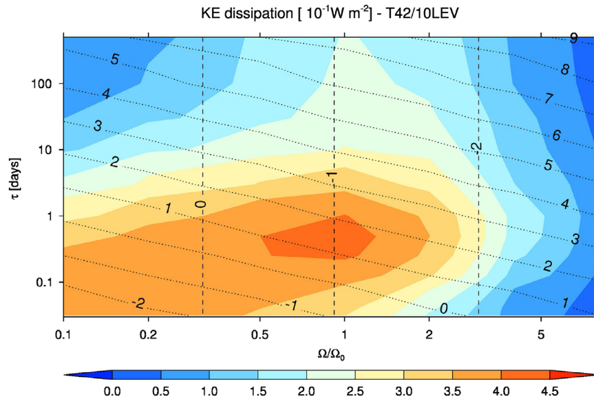
Fig. 4. Total kinetic energy dissipation; overplotted (as in all the following plots) are the values of \log_{10} \mathcal{R}o (dashed) and \log_{10} \mathcal{F}_f (dotted).
