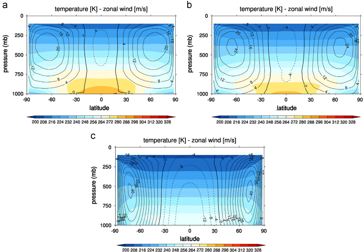
Fig. 2. Zonal winds and temperature for. (a) \mathcal{F}_f = 1.5 \times 10^{-3} , Ro = 8 . (b) \mathcal{F}_f = 1 , Ro = 8 . (c) \mathcal{F}_f = 4 \times 10^5 , Ro = 8 . (d) \mathcal{F}_f = 10^{-1} , Ro = 0.08 . (e) \mathcal{F}_f = 10^2 , Ro = 0.08 . (f) \mathcal{F}_f = 4 \times 10^5 , Ro = 0.08 . (g) \mathcal{F}_f = 10 , Ro = 10^{-3} . (h) \mathcal{F}_f = 10^4 , Ro = 10^{-3} . (i) \mathcal{F}_f = 10^9 , Ro = 10^{-3} .
