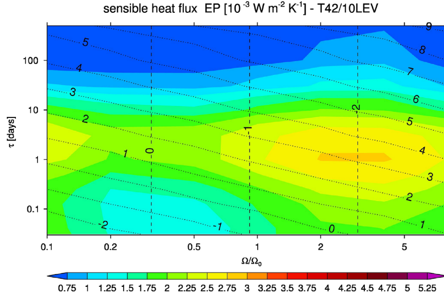
Fig. 8. Entropy production associated with sensible heat flux. Units in 10^{-3} \text{ W m}^{-2} \text{ K}^{-1} .
