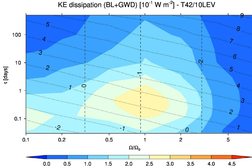
Fig. 5. Contribution to the total kinetic energy dissipation due to parametrizations representing boundary layer stresses and gravity wave drag, D_{phys} .
