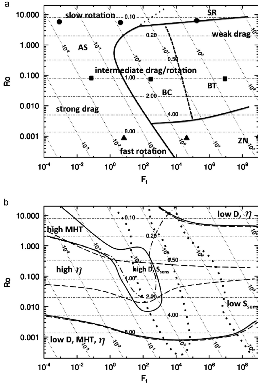
Fig. 1. (a) Schematic diagram of the (F_f, Ro) parametric space spanned in this study. Overplotted are the values of \Omega^* (dashed-dotted) and \tau (dotted). We have schematically sketched the boundaries between different circulation regimes found for dry PlaSim on the base of the circulations (AS, axisymmetric; BC, baroclinic; BT, barotropic; ZN, zonostrophic; SR, super-rotation). Circles, pentagons and triangles represent the simulations performed with \Omega^* = 0.1, 1, 8 respectively (see Figs. 3 and 2). (b) The same regime diagram is summarizing schematically the properties of kinetic energy dissipation (continuous line, high and low D ), meridional energy transport (dotted-dashed line, high MHT), thermal material entropy production (dotted line, high and low S_{sens} ), efficiency (dashed line, high and low \eta ).
