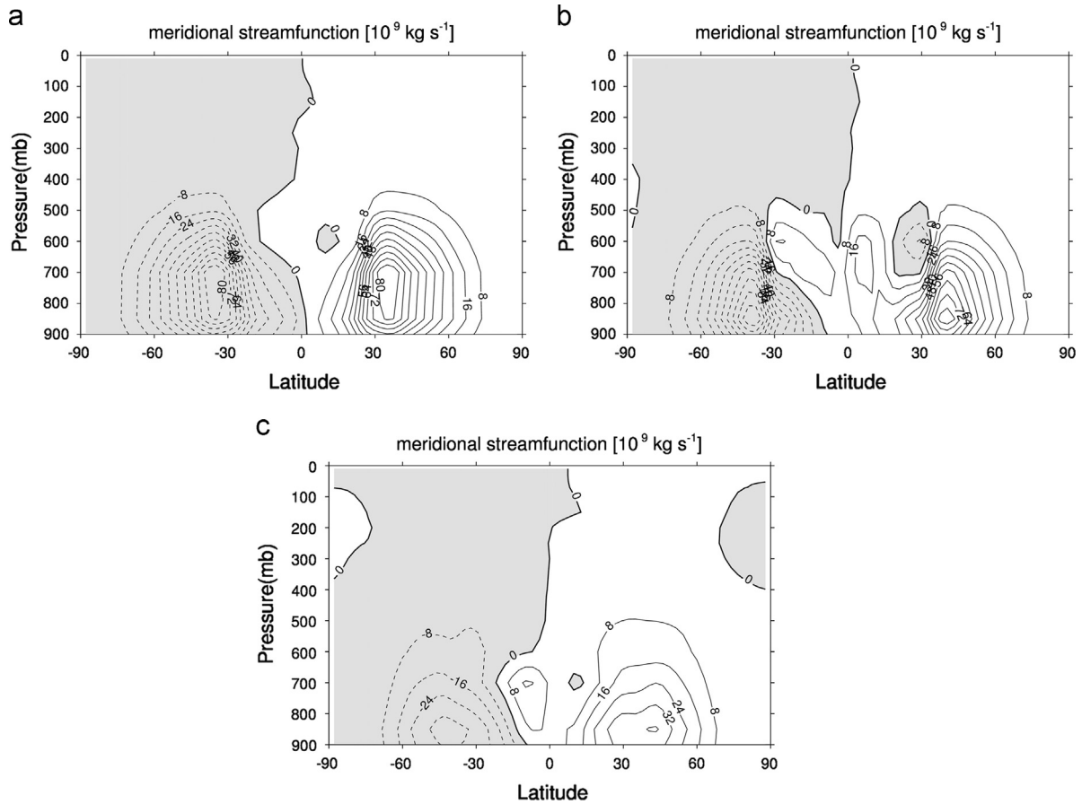
Fig. 3. As in Fig. 5 but for the meridional mass streamfunction (units 10 9 kg s -1 ). (a) \mathcal{F}_f = 1.5 \times 10^{-3} , Ro = 8 . (b) \mathcal{F}_f = 1 , Ro = 8 . (c) \mathcal{F}_f = 4 \times 10^5 , Ro = 8 . (d) \mathcal{F}_f = 10^{-1} , Ro = 0.08 . (e) \mathcal{F}_f = 10^2 , Ro = 0.08 . (f) \mathcal{F}_f = 4 \times 10^5 , Ro = 0.08 . (g) \mathcal{F}_f = 10 , Ro = 10^{-3} . (h) \mathcal{F}_f = 10^4 , Ro = 10^{-3} . (i) \mathcal{F}_f = 10^9 , Ro = 10^{-3} .
