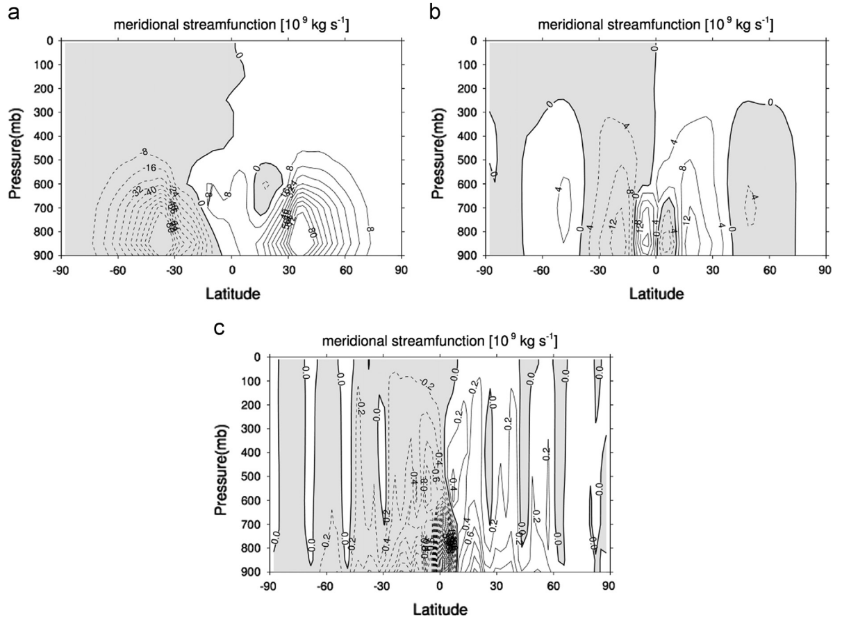
Fig. 14. Meridional streamfunction for \Omega^* = 1/10 (a), \Omega^* = 1 (b) and \Omega^* = 8 for the BLS simulations.
