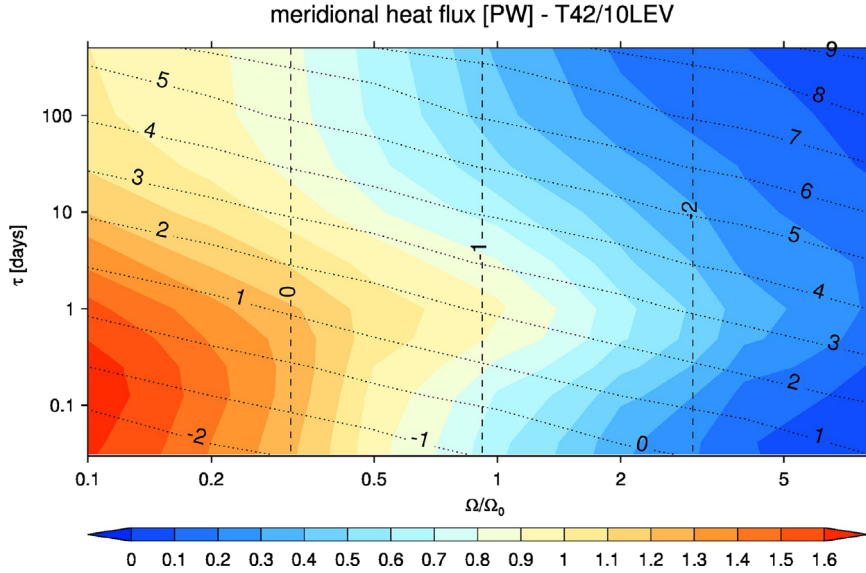
Fig. 6. Atmospheric meridional energy transport index MHT .
