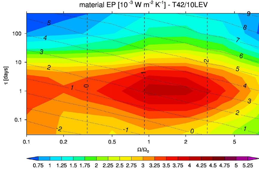
Fig. 10. Total material entropy production. Units in 10^{-3} \text{ W m}^{-2} \text{ K}^{-1} .
