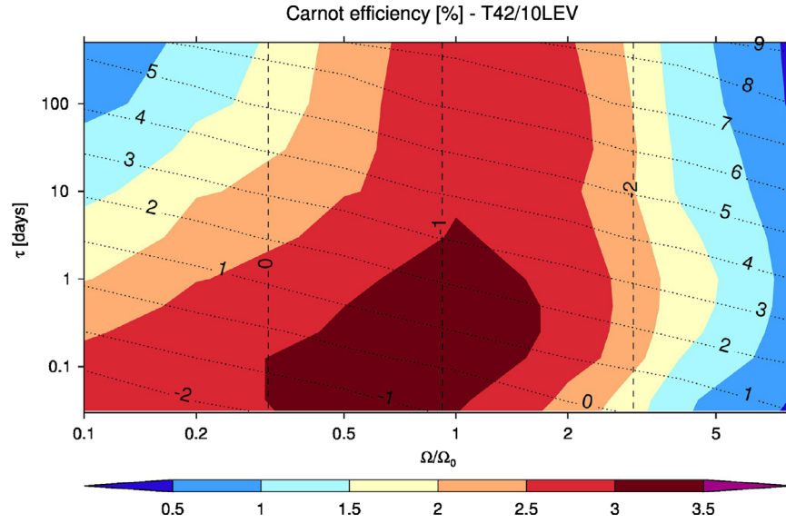
Fig. 7. Carnot efficiency \eta .
