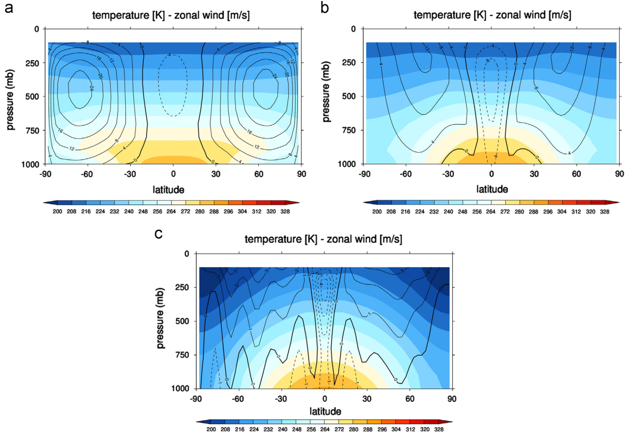
Fig. 13. Zonal winds and temperature for \Omega^* = 1/10 (a), \Omega^* = 1 (b) and \Omega^* = 8 for the BLS simulations.
