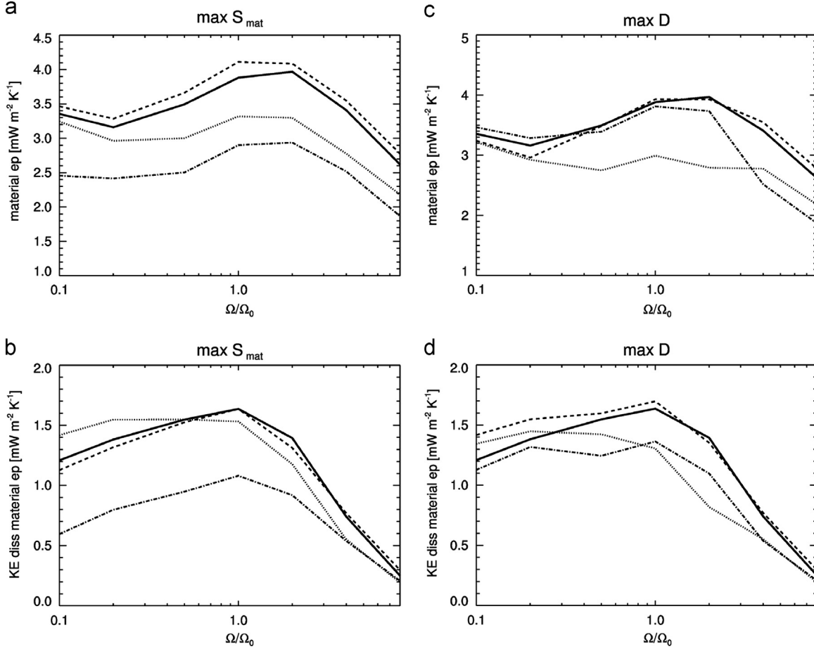
Fig. 12. \dot{S}_{mat} (a) and \dot{S}_{kediss} (b) for the control runs BLS (continuous line), for \tau_{max}(\Omega^*) maximizing \dot{S}_{mat} (dashed) and for \tau = 0.1\tau_{max} (dotted) and \tau = 10\tau_{max} (dotted–dashed) days. (c)–(d) Same as in (a) and (b) but for \tau_{max} maximising \dot{S}_{kediss} .
