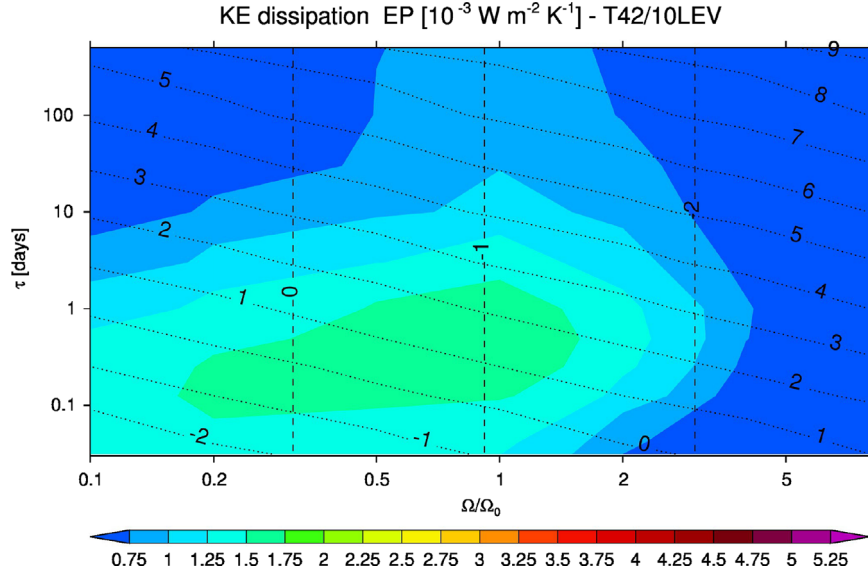
Fig. 9. Material entropy production associated with dissipation of kinetic energy. Units in 10^{-3} \text{ W m}^{-2} \text{ K}^{-1} .
