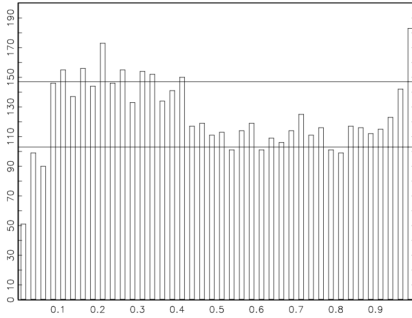
Figure 8: \zeta -histogram (40 cells) for 5000 one-step-ahead forecasts. DGP with st(0, 1, \exp(0.3), 8) errors. The MLEs were computed assuming the innovations are Student-t distributed.
