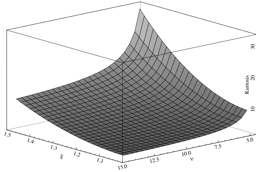
Figure 4: Kurtosis implied by several combinations of 1 \leq \xi \leq 1.5 and 4.5 \leq v \leq 15
