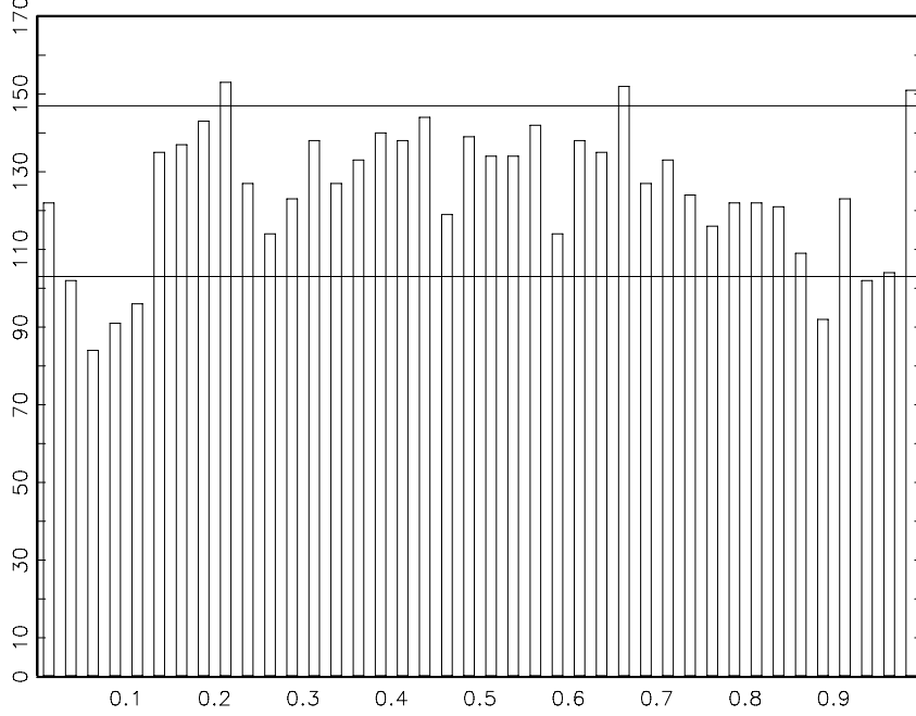
Figure 7: \zeta -histogram (40 cells) for 5000 one-step-ahead forecasts. DGP with t(0, 1, 8) errors. The MLEs were computed assuming normality for the innovations.
