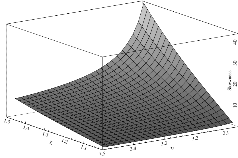
Figure 3: Skewness implied by several combinations of 1 \leq \xi \leq 1.5 and 3.05 \leq v \leq 3.5
