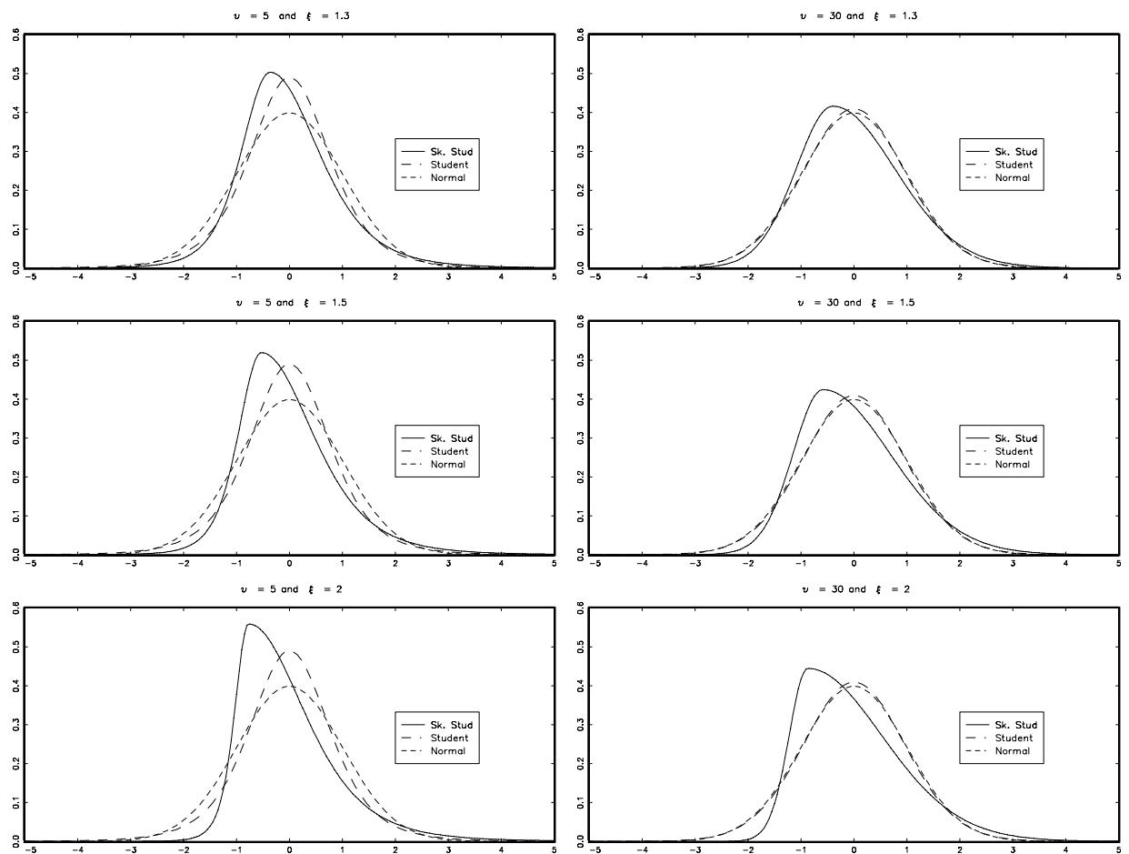
Figure 6: Normal, Student and skewed Student densities.
