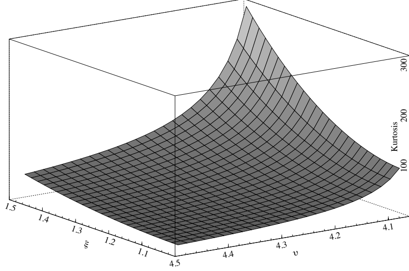
Figure 5: Kurtosis implied by several combinations of 1 \leq \xi \leq 1.5 and 4.05 \leq \nu \leq 4.5
