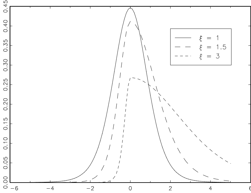
Figure 1: Skewed Student densities with v = 8 and \xi = 1, 1.5 and 3 .
