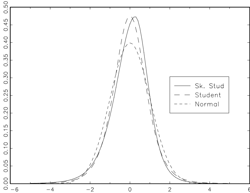
Figure 10: st(0, 1, \exp(-0.179), 6.039) (solid line), t(0, 1, 5.57) (dashed line) and N(0, 1) (short dashes).
