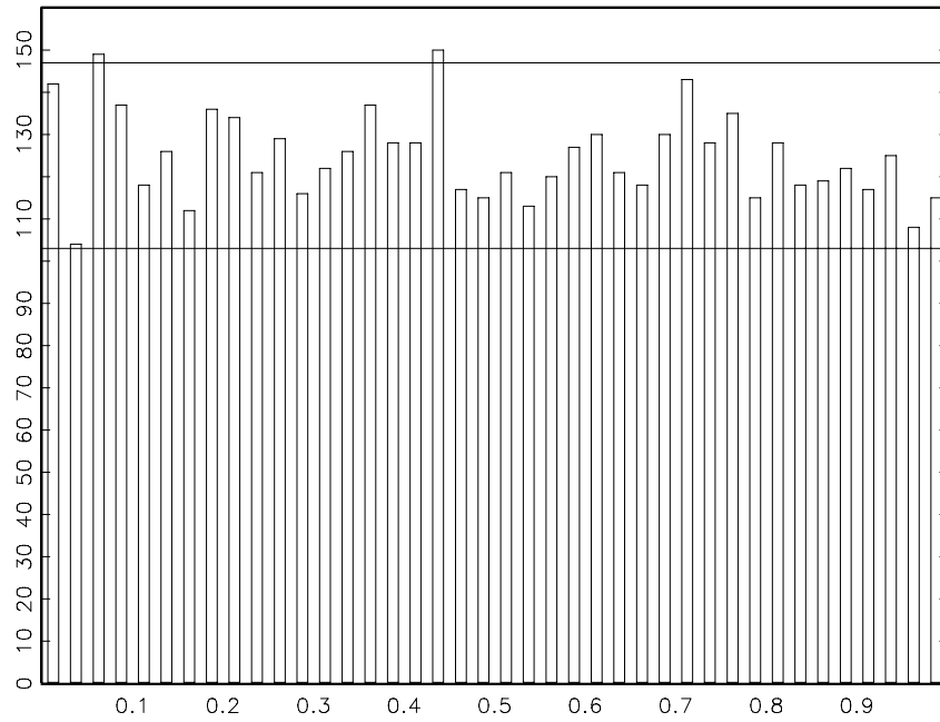
Figure 9: \zeta -histogram (40 cells) for 5000 one-step-ahead forecasts. DGP with st(0, 1, \exp(0.3), 8) errors. The MLEs were computed assuming the innovations are skewed Student-t distributed.
