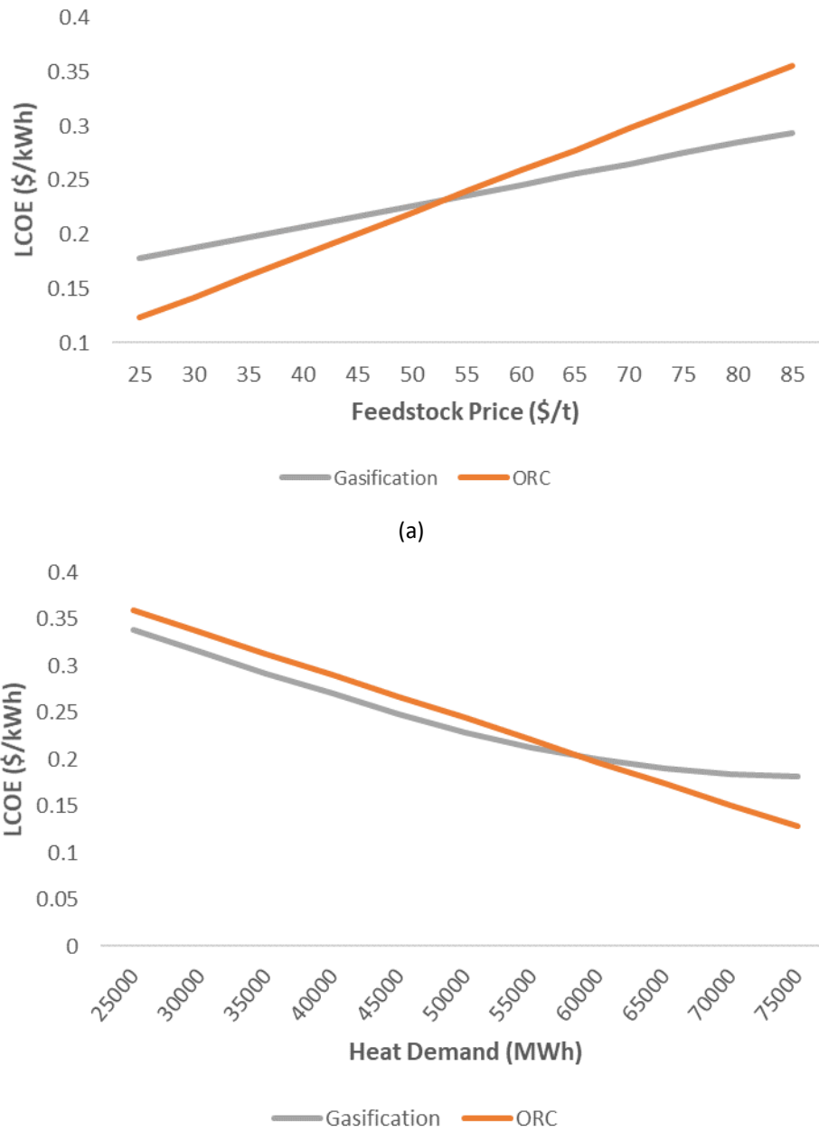
Figure 12. Variation of LCOE versus feedstock price (a) and annual heat demand (b).
