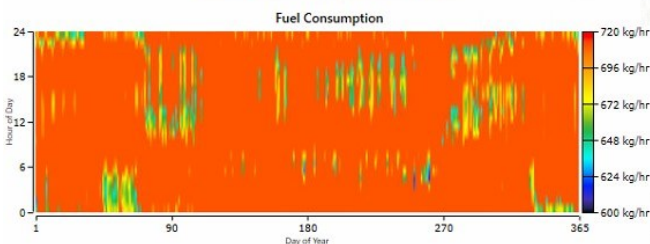
Fig 18. Diesel consumption of Diesel-Biomass scenario throughout a year
