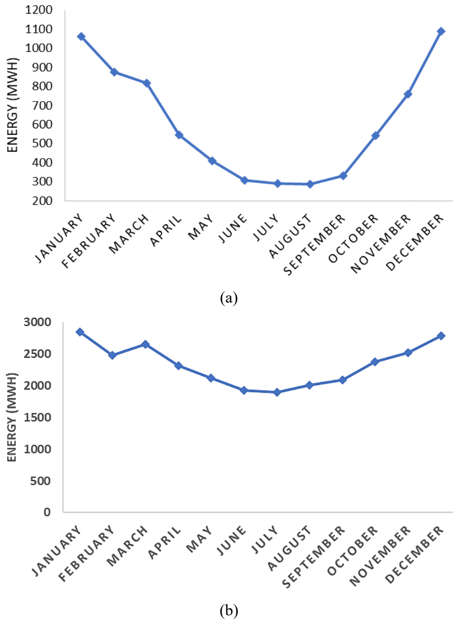
Figure 7. Monthly heating demand profile in residential (a) and industrial sector (b).
