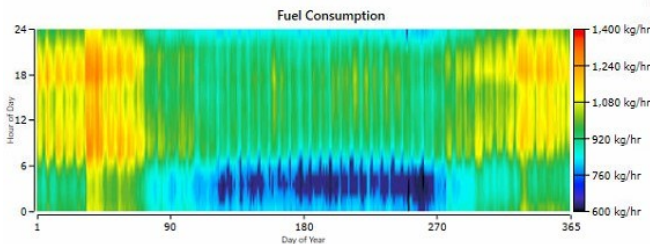
Fig 17. Diesel consumption of base-scenario throughout a year
