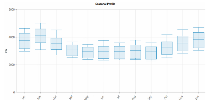
Fig 13. Load variations throughout a year
