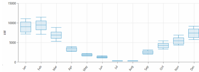
Fig 15. Load variations of community load throughout a year
