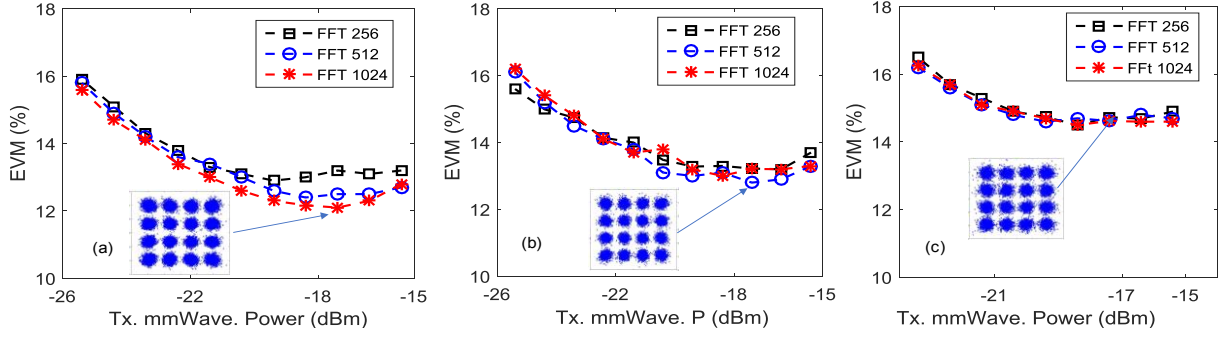
Fig. 4. Performance of OFDM signal for different FFT sizes and fiber transmission lengths: (a) 10-km SMF; (b) 20-km SMF; (c) 30-km SMF.
