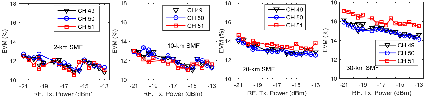
Fig. 10. Uplink signal performance for different RF transmit powers and different fiber lengths.
