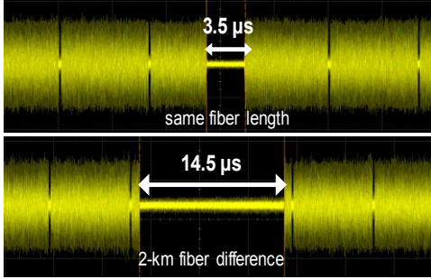
Fig. 12. The spectral and interrupted time during radio cell switching.
