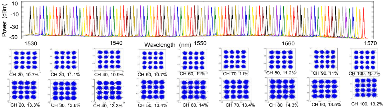
Fig. 11. Spectra of the switched optical SSB signals and examples of the signal performance for systems using 10-km SMF (upper) and 20-km SMF (lower).
