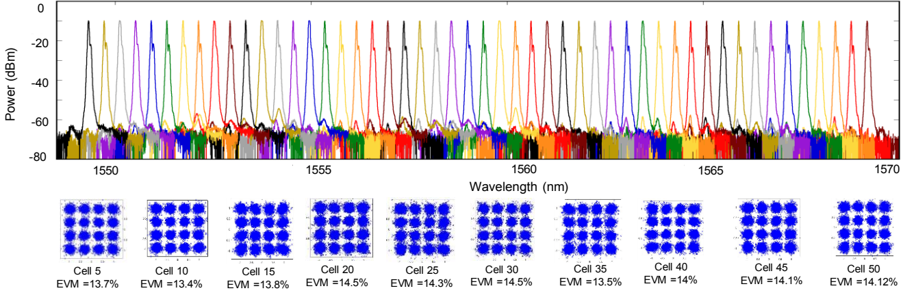
Fig. 8. Spectrum of switched optical SSB signals and examples of signal performance at different cells.
