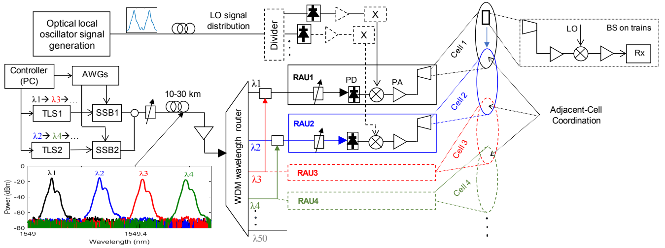
Fig. 2. Experimental setup for a handover-free communication to high-speed trains by switched WDM fiber-wireless system. Dashed-line parts were not performed in the proof-of-concept demonstration.
