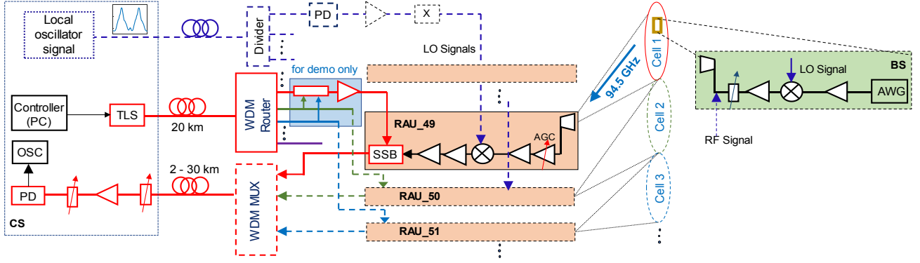
Fig. 9. Experimental setup for a proof-of-concept demonstration of uninterrupted communications from HSTs to the CS on the ground. Dashed-line parts were not performed in our proof-of-concept demonstration.
