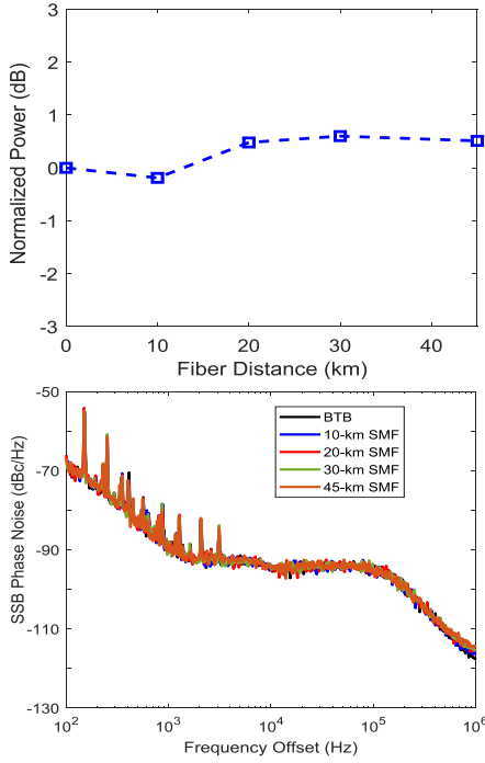
Fig. 3. (a) LO normalized power; and (b) SSB phase noise characteristics.
