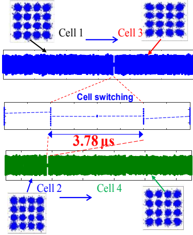
Fig. 7. Cell switching by the wavelength-tunable lasers.
