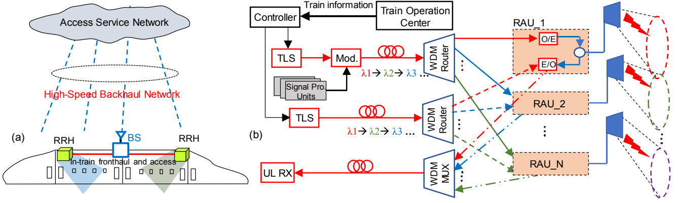
Fig. 1. (a) Concept of a cell-less network for HSTs; (b) A cell-less network for HSTs by a moving fiber-wireless backhaul system.
