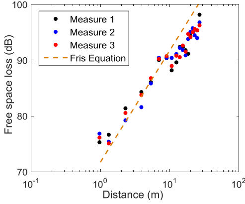
Fig. 13. Free space loss measurement for a carrier signal at 92 GHz.
