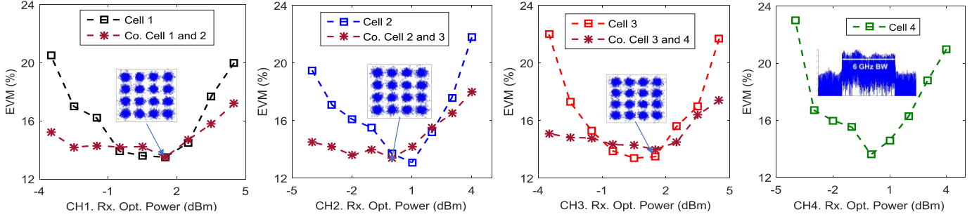
Fig. 6. Transmission performance of fiber-wireless links and joint coordination between adjacent cells.
