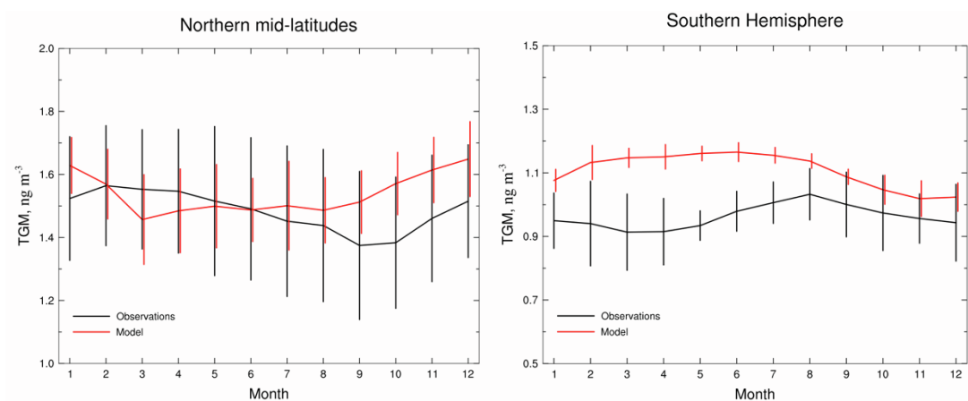
Fig. S2. The modeled seasonal cycle of atmospheric Hg concentrations against observations in typical sites
