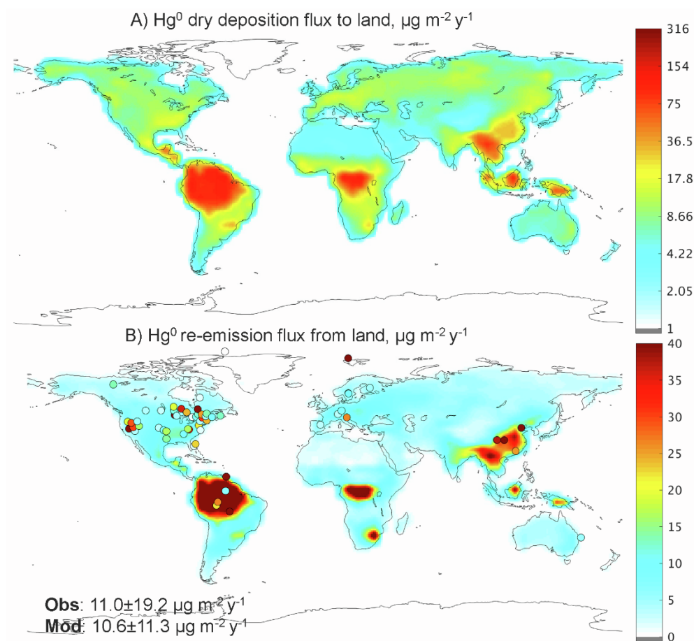
Fig. S3. Modeled air-land exchange fluxes of \text{Hg}^0 against observations
