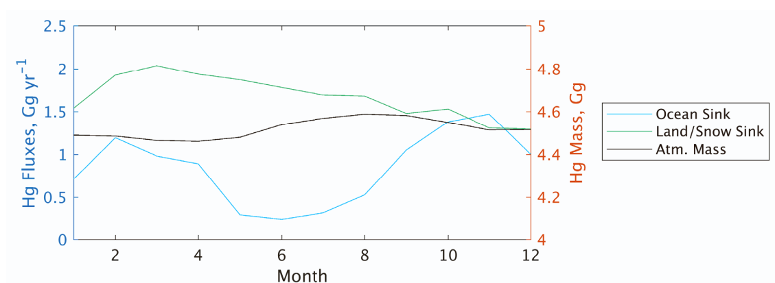
Fig. S9 Monthly variability of burial of Hg by land and ocean.
