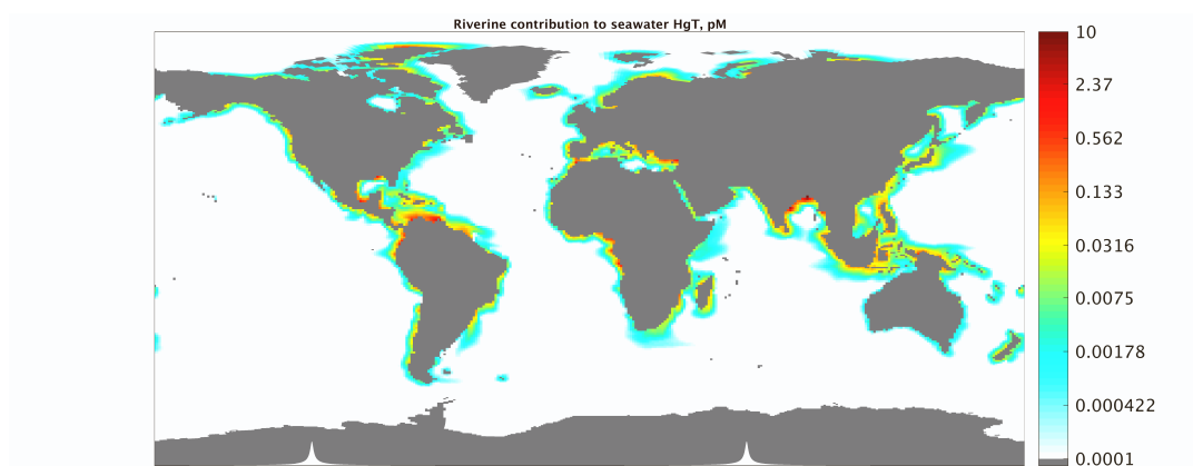
Fig. S7 Contribution of riverine sources to seawater total Hg concentrations Unit: pM ( 1 \text{ pM} = 10^{-12} \text{ mol/L} ).
