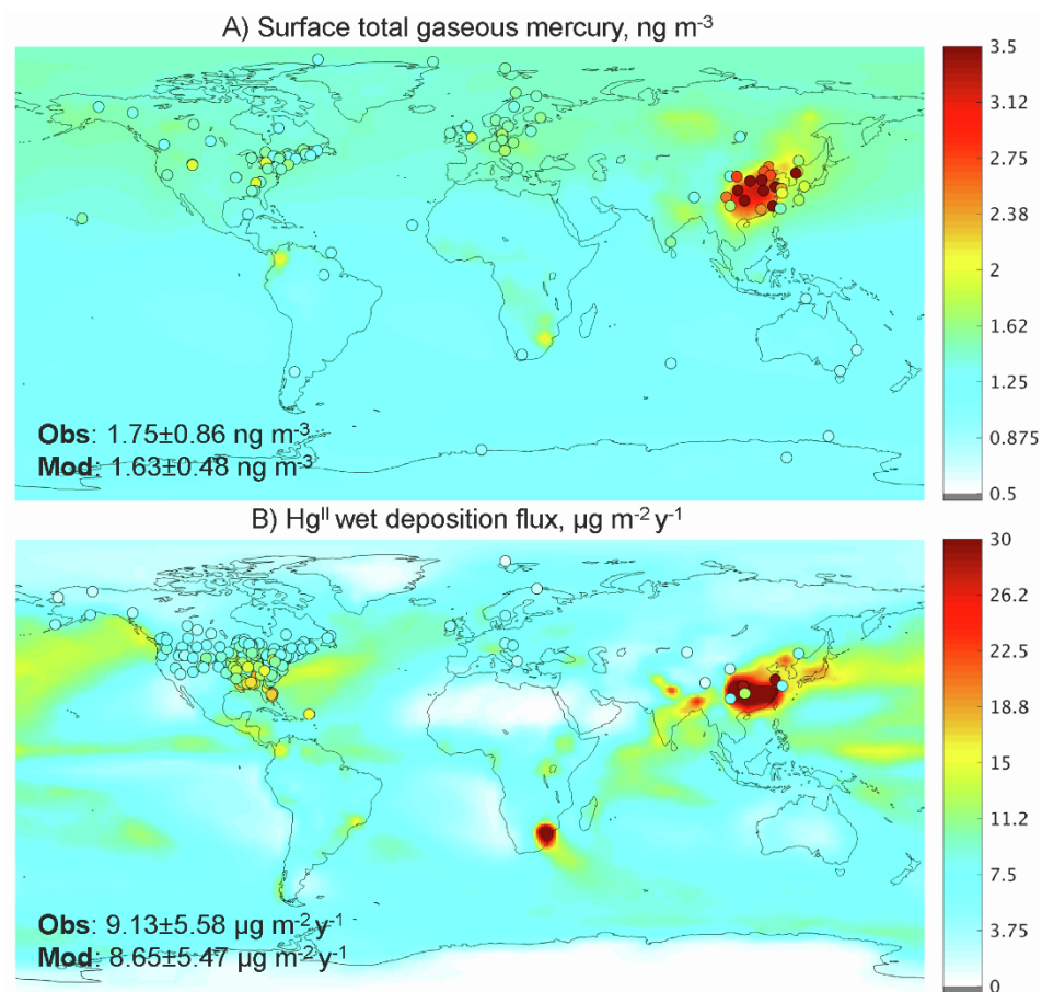
Fig. S1. Comparison between model and observations for the atmosphere Hg abundance
