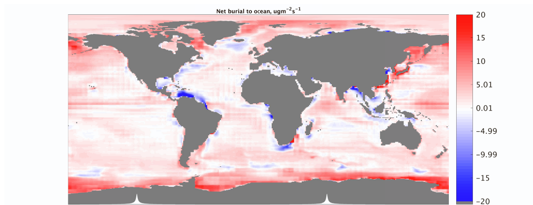
Fig. S11 Burial of primary atmospheric emissions to the ocean
