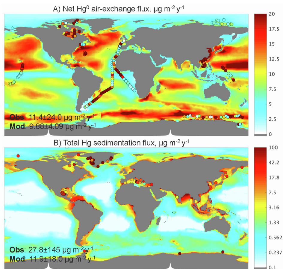
Fig. S5. Comparison between model and observations for ocean-related Hg fluxes Comparison against observed net \text{Hg}^0 air-sea exchange at the ocean surface: (A) and Hg sedimentation fluxes at the ocean floor (B) ( \mu\text{g m}^{-2} \text{yr}^{-1} ). The data sources are summarized by Huang and Zhang et al. 4 and Liu et al. 5
