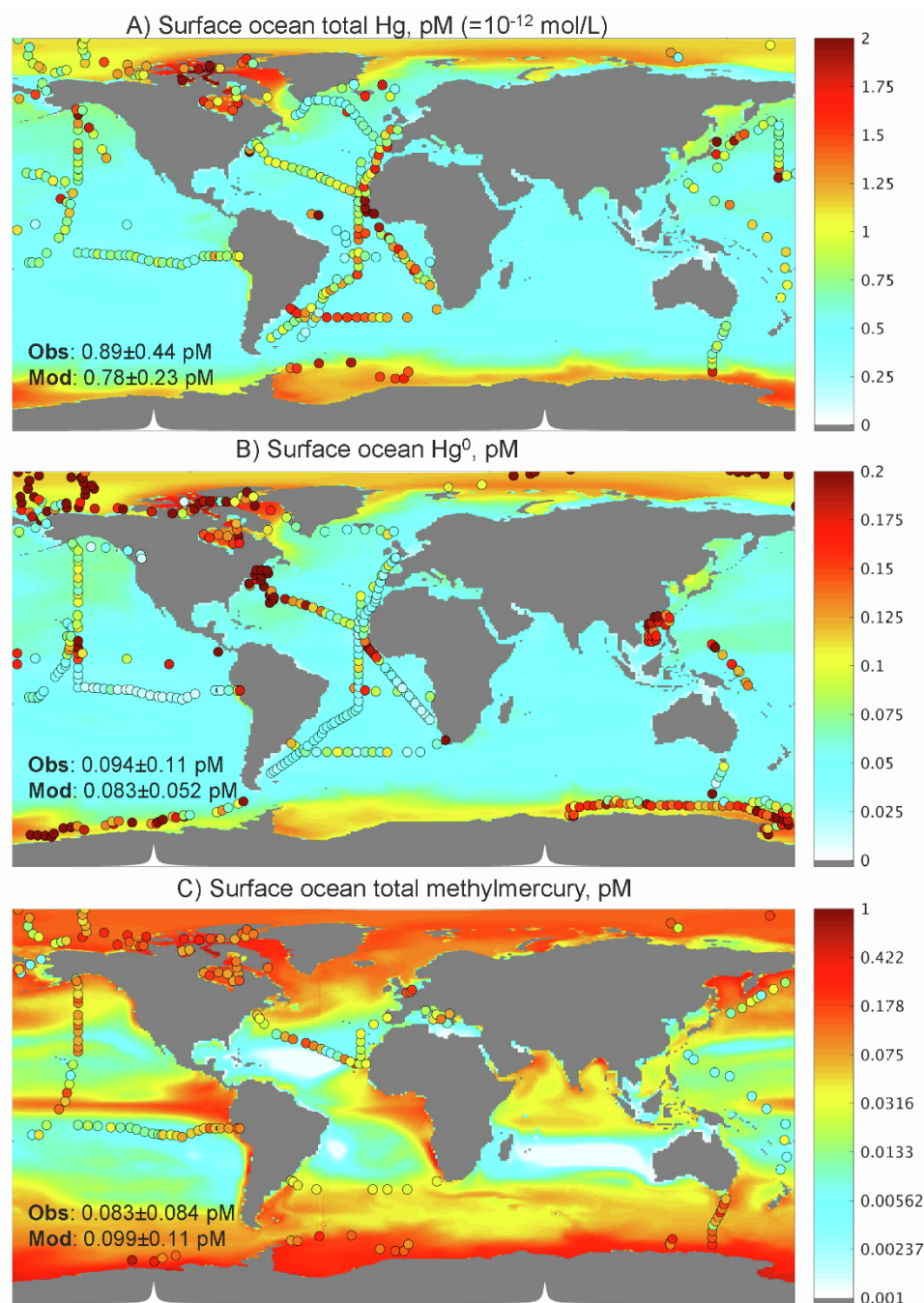
Fig. S4. Comparison between model and observations for Hg abundance in the ocean
