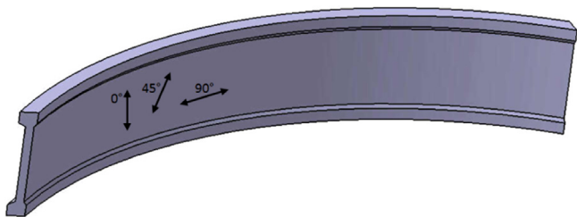
Fig. 1. Forged part made of alloy Ti-6Al-4V (with extraction directions).
