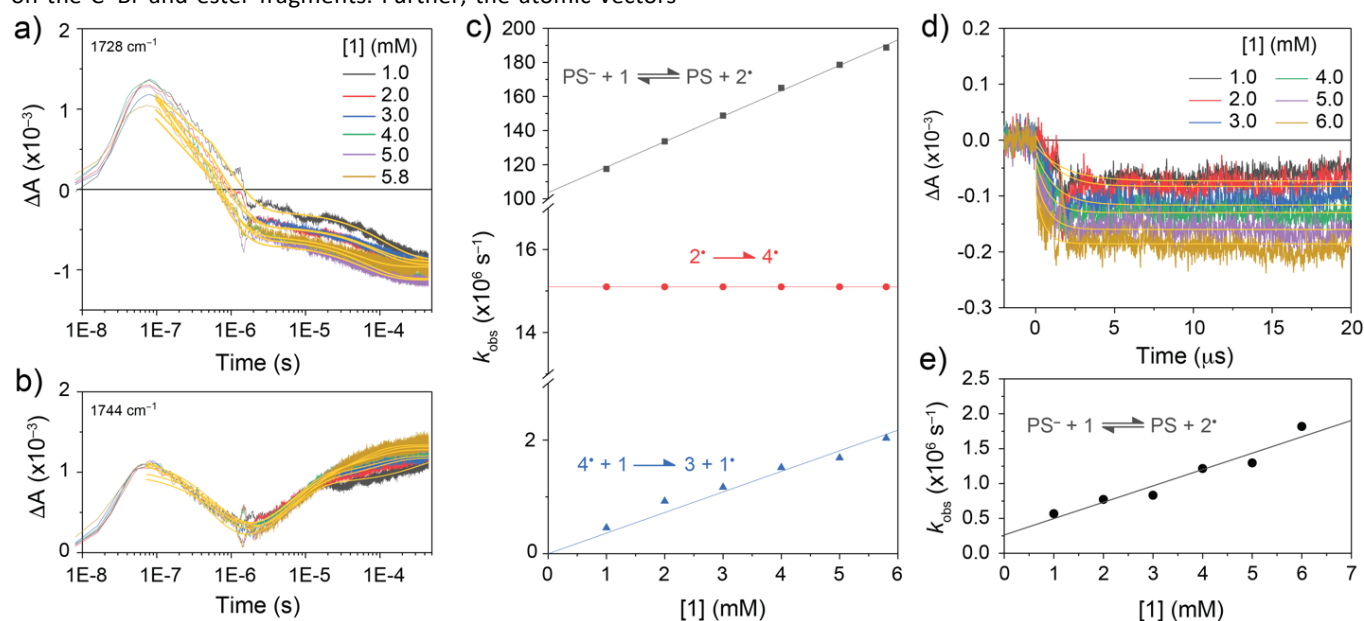
Figure 9. Absorption changes following pulsed 532 nm excitation of RuPS monitored at a) 1728 cm -1 and b) 1744 cm -1 with the indicated concentration of 1 in CH 2 Cl 2 . c) Pseudo-first-order observed rate constants rates extracted from data in a) and b) plotted against [1]; the corresponding reaction chemistries are indicated for each dataset. d) Absorption changes measured at 1728 cm -1 for FePS following pulsed 532 nm laser excitation at the indicated [1]. e) Pseudo-first-order observed rate constants rates extracted from data in d) plotted against [1].
