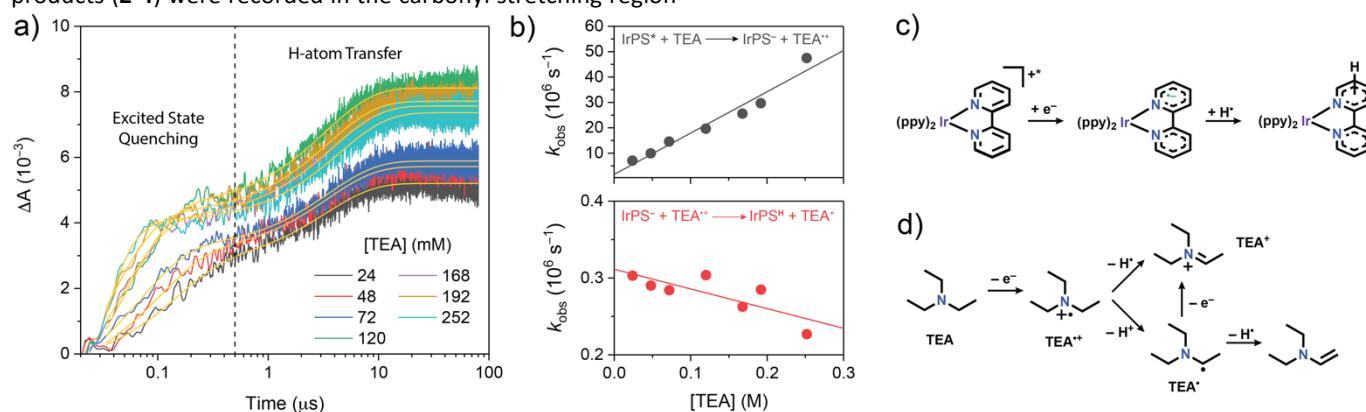
Figure 7. a) Single wavelength kinetics traces measured for [\text{Ir}(\text{ppy})_2(\text{bpy})]^{+} in \text{CH}_3\text{CN} at 420 \text{ nm} after pulsed 450 \text{ nm} excitation at the indicated amounts of titrated TEA. b) Observed rates measured for the indicated reactions versus [TEA]. c) Related reductive quenching of [\text{Ir}(\text{ppy})(\text{bpy})]^{+} to generate the monoreduced [\text{Ir}(\text{ppy})(\text{bpy})]^- , which is followed by H-atom transfer to the reduced bipyridine ligand. d) Cascade chemistry associated with \text{TEA}^{+\bullet} when TEA is oxidized by one electron. 70-74
