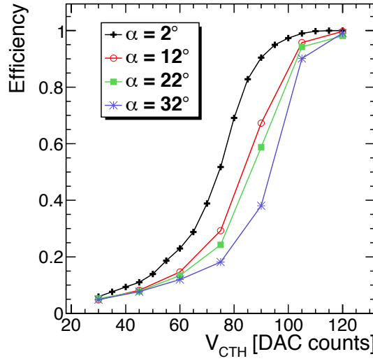
Figure 17. Per-sensor efficiency for DUT sensor S0 as function of V_{\text{CTH}} , for different incident angles \alpha .
