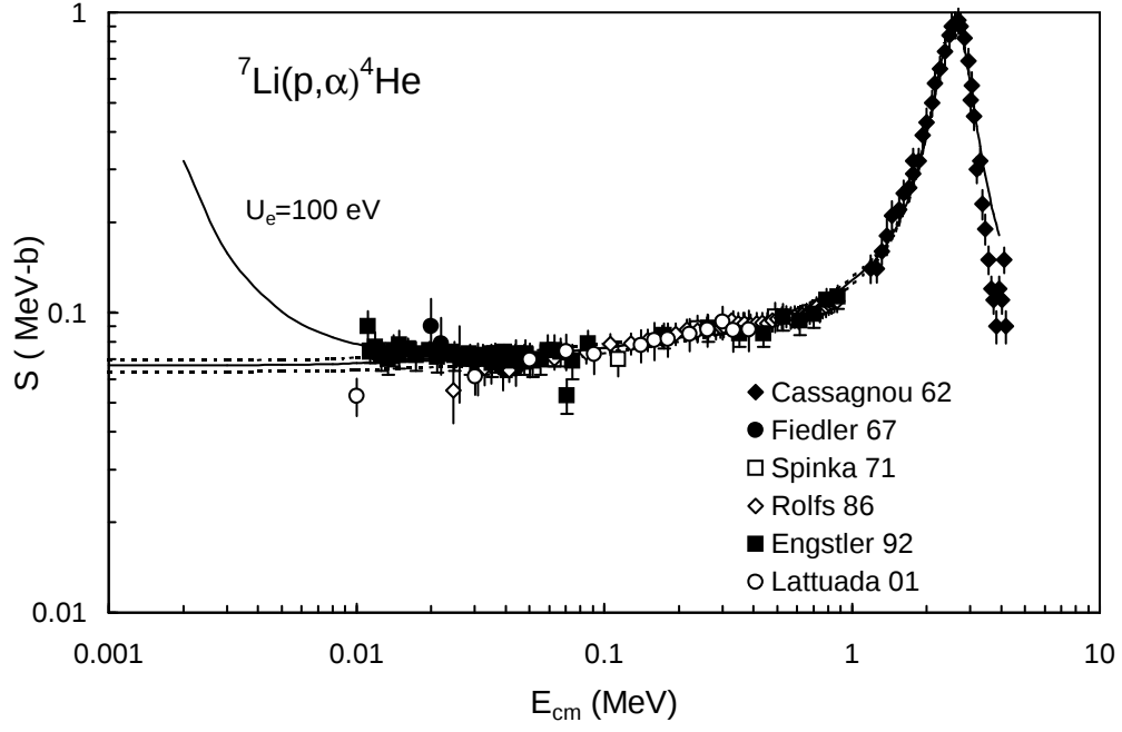
FIG. I.i. {}^7\text{Li}(p,\alpha){}^4\text{He} S factor. The data are taken from Ref. [76] (Cassagnou 62), Ref. [77] (Fiedler 67), Ref. [78] (Spinka 71), Ref. [79] (Rolfs 86), Ref. [80] (Engstler 92), and Ref. [49] (Lattuada 01).
