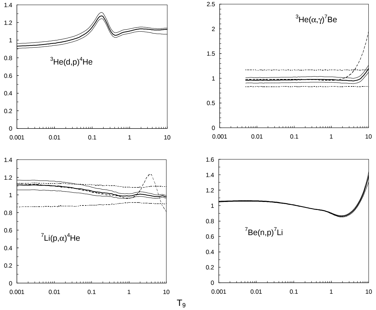
FIG. II.b. Ratios of the present reaction rates to the NACRE and SKM rates.
