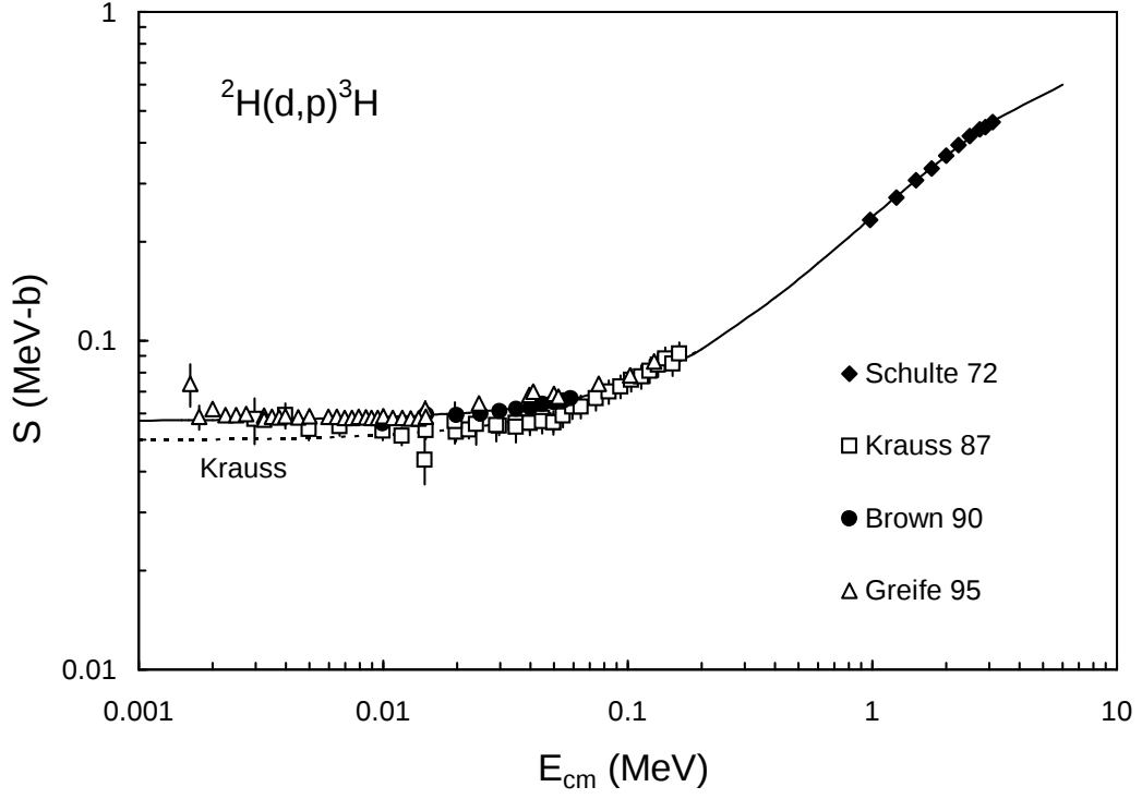
FIG. I.c. {}^2\text{H}(\text{d},\text{p}){}^3\text{H} S factor. The data are taken from Ref. [35] (Schulte 72), Ref. [32] (Krauss 87), Ref. [33] (Brown 90), and Ref. [34] (Greife 95). The dotted curve represents the individual fit to Ref. [32]. Individual fits of Ref. [33] and [34] are very close to the global fit.
