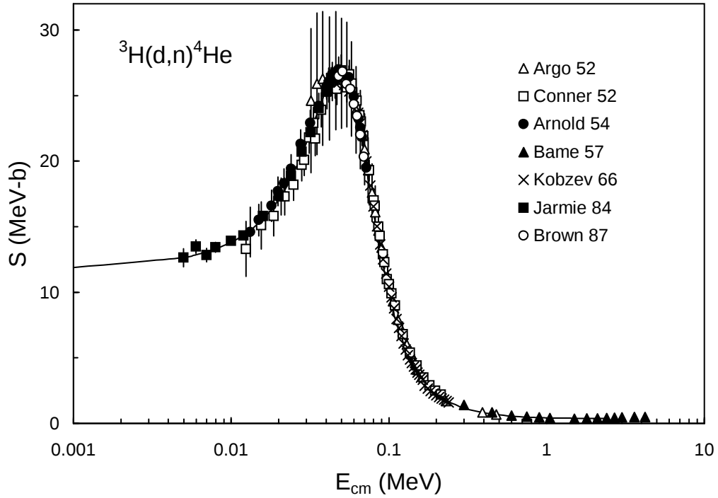
FIG. I.d. {}^3\text{H}(\text{d},\text{n}){}^4\text{He} S factor. The data are taken from Ref. [58] (Argo 52), Ref. [59] (Conner 52), Ref. [60] (Arnold 54), Ref. [61] (Bame 57), Ref. [62] (Kobzev 66), Ref. [63] (McDaniels), Ref. [64] (Jarmie 84), and Ref. [65] (Brown 87).
