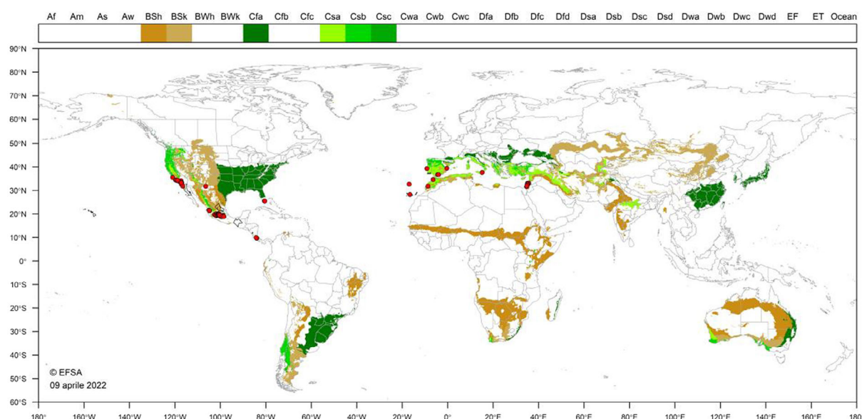
Figure 5: World distribution of Köppen-Geiger climate types that occur in the EU and which occur in sites where Oligonychus perseae has been reported (red dots)
