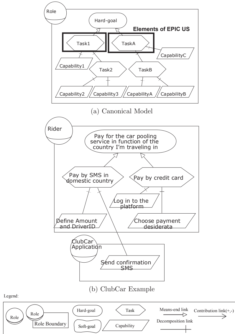
Fig. 3. Top-Level Hard-goal, Several Means-End Decompositions (from [15]).
