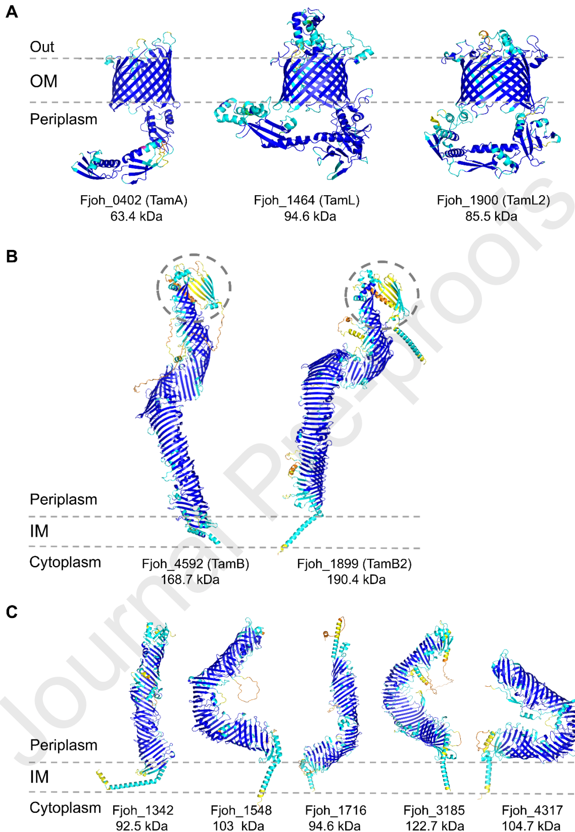
Fig. 1. Three-dimensional structures of TamA (A), TamB (B) and AsmA-like (C) homologs in F. johnsoniae as predicted by AlphaFold2 ( https://alphafold.ebi.ac.uk ) [86]. Protein names and their predicted molecular weights are reported below each structure. Structures are colored based on the per-residue confidence score (pLDDT) between 0 and 100: dark blue (pLDDT > 90), cyan (90 > pLDDT > 70), yellow (70 > pLDDT > 50), and orange (pLDDT < 50). In (A), the N-terminal
