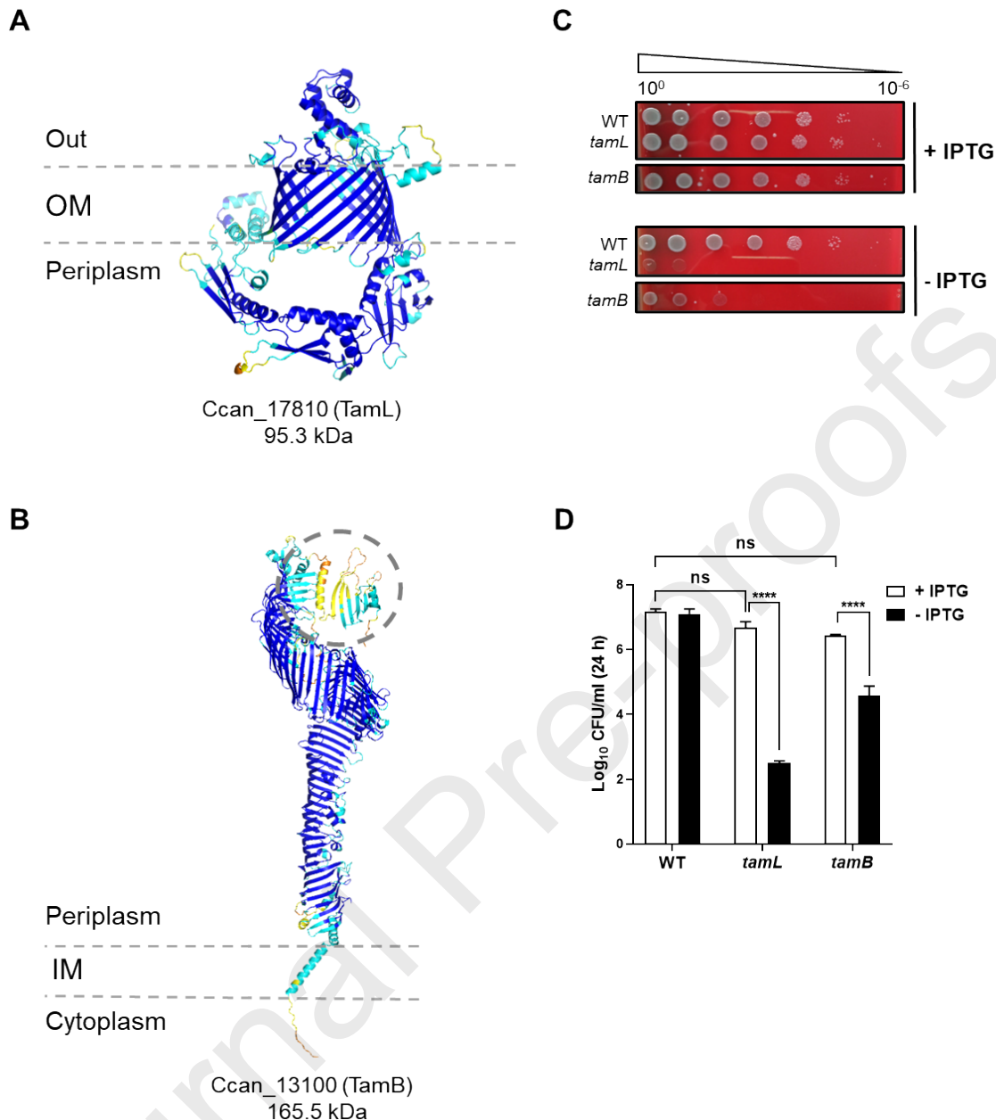
Fig. 9. C. canimorsus possesses one TamL and one TamB protein. (A and B), three-dimensional structures of TamA (A), TamB (B) homologs in C. canimorsus as predicted by AlphaFold2 [86]. Protein names and predicted molecular weights are reported below each structure. Structures are colored based on the per-residue confidence score (pLDDT) between 0 and 100: dark blue (pLDDT>90), cyan (90>pLDDT>70), yellow (70>pLDDT>50), and orange (pLDDT<50). In (A), the N-terminal lipid moiety that likely anchors TamL to the outer membrane is not shown. In (B), the predicted C-terminal pseudosubstrate domain is highlighted via a dashed circle. (C and D), effect of TamL depletion on cell viability in C. canimorsus . (C) Spot assay of wild-type (WT), P_{ompA}::lacI-P_{cfxA-lacO}::tamL ( tamL ) and P_{ompA}::lacI-P_{cfxA-lacO}::tamB ( tamB ) strains grown in SB (+/- IPTG). Plates were incubated at 37°C, 5% CO 2 and photographed after 48 hours. (D) End-point growth of the same strains as in (C) in heat-inactivated human serum. After 24 hours of growth, cells were plated on SB to enumerate the CFUs/ml. Data were then Log 10 -transformed and displayed as mean \pm standard deviation from at least three independent experiments. A one-way ANOVA followed by Tukey's multiple comparison test was performed. Statistical significance is displayed as following: ns = not significant; **** = p < 0.0001 .
