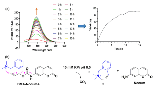
Fig. 2 (a) Stability study of DMA-NcoumA (6 \mu M) in 1% DMSO in KPi (10 mM, pH 8.0) for 15 h at 37 ^{\circ} C, \lambda_{\text{ex}} = 342 nm, \lambda_{\text{em}} = 375 –600 nm. (b) Proposed degradation mechanism.
