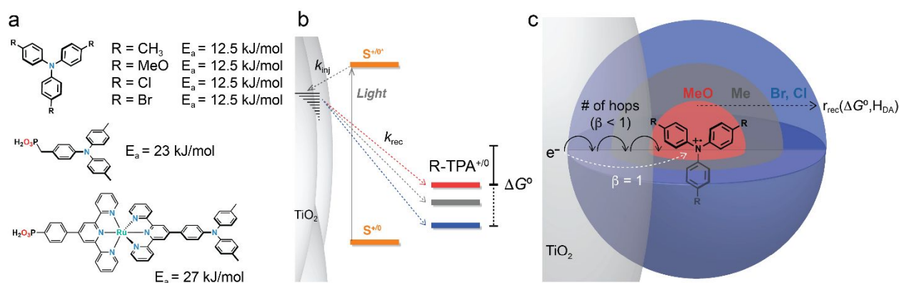
Figure 10. a) The TPA compounds utilized and the measured activation barriers for the recombination reactions. b) The dye-sensitization mechanism utilized to generate the \text{TiO}_2(\text{e}^-) and \text{TPA}^+ reactants. c) Reaction sphere model for the TPA in fluid solution. When the driving force for electron transfer was large (red) electron transfer followed a first-order kinetic model consistent with transfer from \text{TiO}_2 directly to the \text{MeO-TPA}^+ , while increasingly dispersive kinetics were observed as -\Delta G^0 decreased from black to blue.
