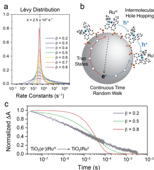
Figure 5. a) Lévy distribution of rate constants with k = 2.5 \times 10^4 \text{ s}^{-1} and the indicated \beta values. b) Illustration of injection electron, intermolecular self-exchange ‘hole-hopping’ and electron transport between trap states modelled as a continuous time random walk. c) Time resolved absorption change associated with \text{TiO}_2(\text{e}^-)|\text{Ru}^{\text{III}} \rightarrow \text{TiO}_2|\text{Ru}^{\text{II}} charge recombination with overlaid fits to the KWW function, Equation 3 .
