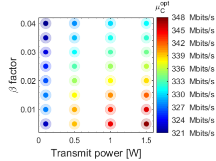
(b) Associated maximal average capacity \mu_C^{\text{opt}} .
