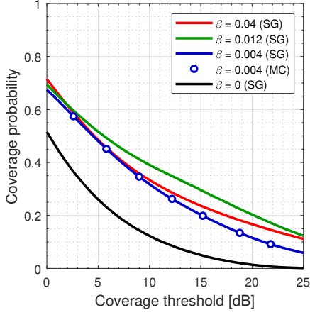
(a) Coverage probability P_c(\theta_c) for an arbitrary UE.
