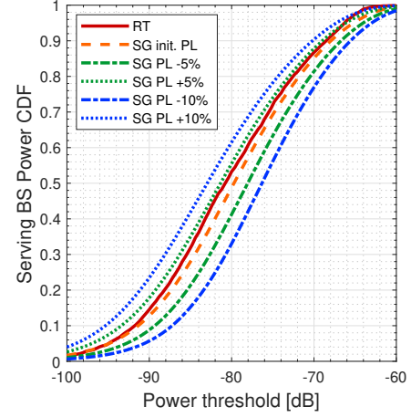
(a) Impact of PL exponents estimation errors on the CDF of the useful received power
