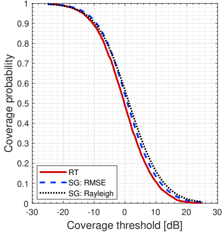
(a) Coverage probability P_c(\theta_c) .
