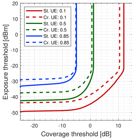
(b) Isocurves of the lower bound for the joint distribution for F(\theta_c, \theta_e) \in \{0.1, 0.5, 0.85\} , \alpha_L = 2.5 , \alpha_N = 2.7 and W = 0\text{W} .
