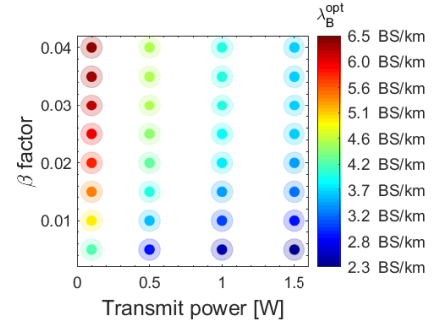
(a) Optimal BS density \lambda_B^{\text{opt}} .
