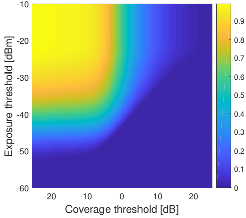
(a) Lower bound on joint metric F(\theta_c, \theta_e) for an arbitrary UE.
