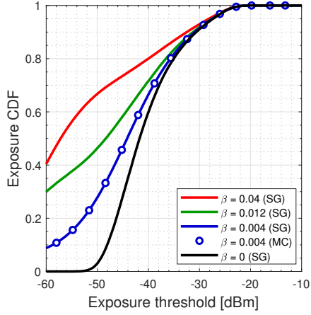
(b) Exposure CDF P_e(\theta_e) for an arbitrary UE.
