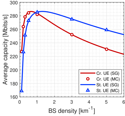
(a) Average UE capacity for \alpha_L = 2 , \alpha_N = 2.25 and W = -93\text{dBm} .
