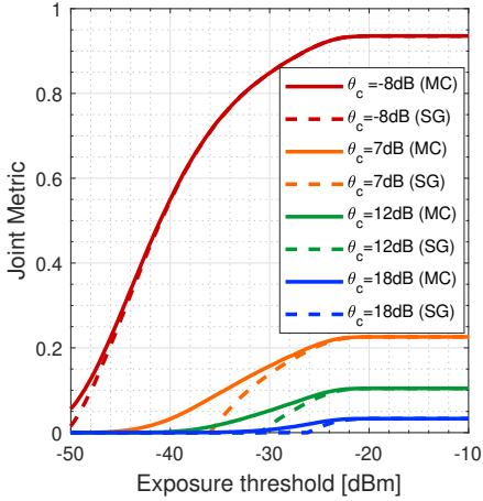
(b) Assessment of the SG lower bound for fixed values of \theta_c .
