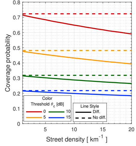
(a) Impact of \lambda_S on P_{c,1} .
