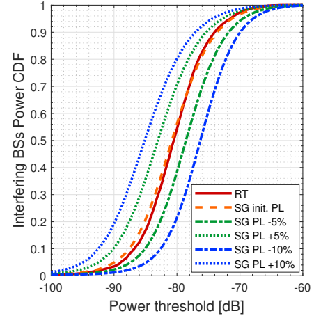
(b) Impact of PL estimation errors on the CDF of the aggregate interference
