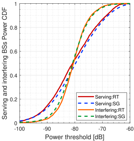
(c) Received and interfering powers (RMSE only)
