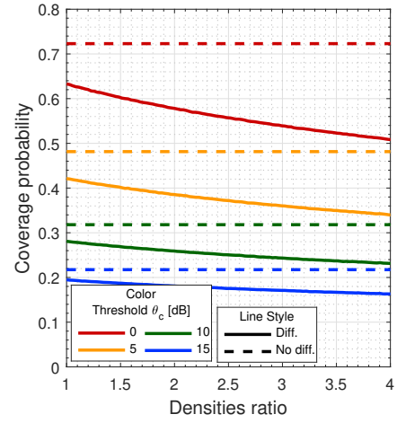
(b) Impact of \lambda_B^d/\lambda_B^t on P_{c,1} .
