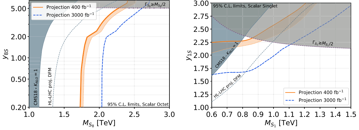
FIG. 2. Projected 95% C.L. exclusions for the scalar color-octet (left) and scalar color-singlet (right) simplified models, presented in mass versus coupling planes, considering luminosities of 400 (orange) and 3000 \text{fb}^{-1} (dashed blue). The solid orange lines represent exclusions obtained with conservative top-tagging performance, while the dashed orange lines refer to a more optimistic assumption. These limits are compared to the currently excluded region of the parameter space, obtained from a recast of the CMS-TOP-18-003 analysis (dark shades) [19], and its naive extrapolation for the HL-LHC with 3000 \text{fb}^{-1} (dashed gray). In addition, light gray regions in the top-right corners of the figures represent configurations in which the width of the new scalar is very large, rendering our approach unreliable.
