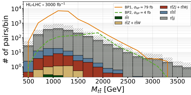
FIG. 1. Distribution of the reconstructed top pair invariant mass M_{\bar{t}t} , normalized to 3000 \text{ fb}^{-1} , resulting from events passing the SR1 selection with conservative top-tagging performance. Predictions are provided for two signal scenarios (defined in the text) alongside all background contributions accounting for theory uncertainties stemming from scale variation. The last bin incorporates overflow events.
