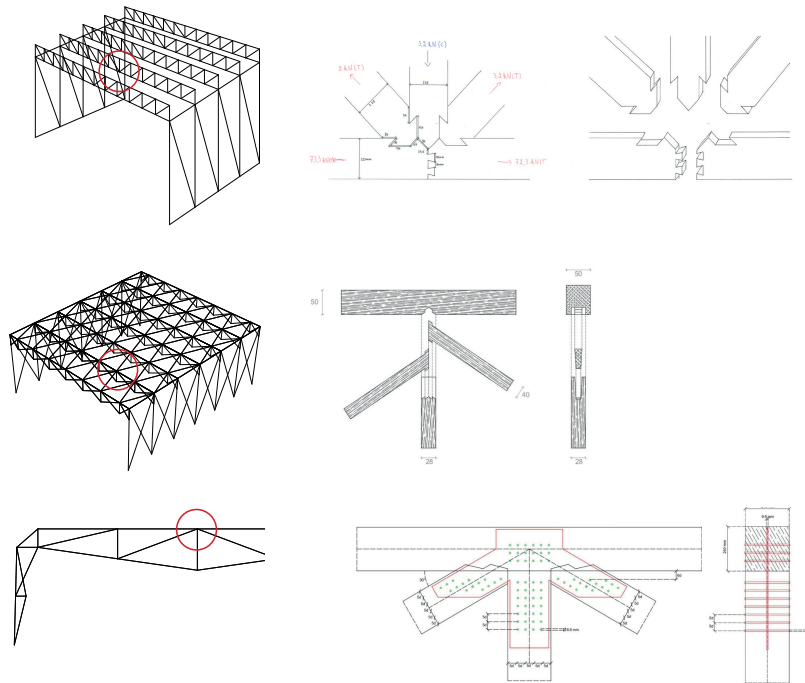
Fig. 9b Structural model (left) and timber-to-timber joint (right). Each line represents a project.
