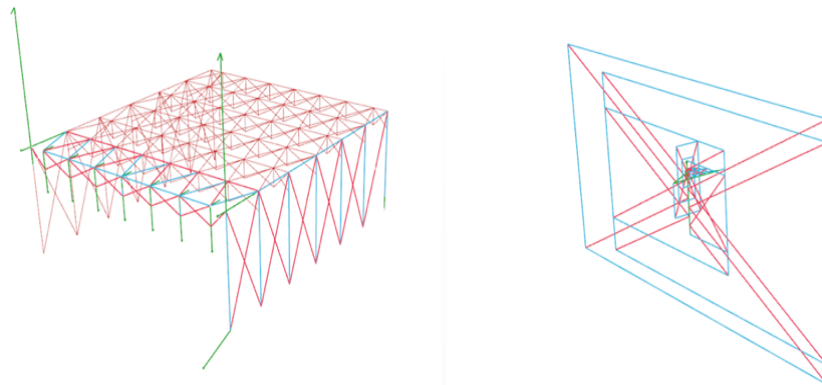
Fig. 8a: Form diagram (left) and forces diagram (right) of the primary structure
