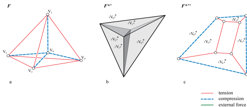
Fig. 2 Graphic statics in 3 dimensions: Form diagram F of a self-stressed tetrahedron (left), polyhedral based force diagram (b), vector-based force diagram (c) . (from D'acunto et al. 2019)
