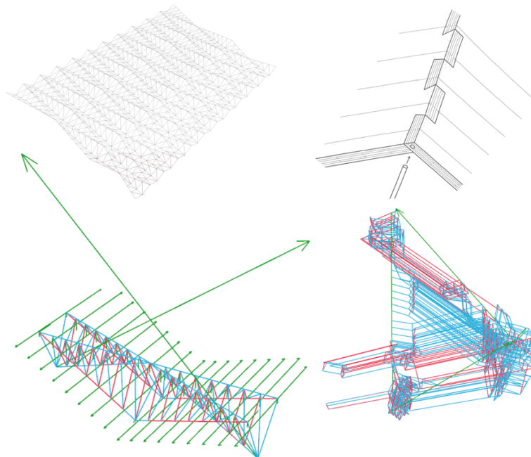
Fig. 7 Synoptic of the final results of group 06 - from top left to bottom right: structural model, assembly proposal, form diagram, force diagram
