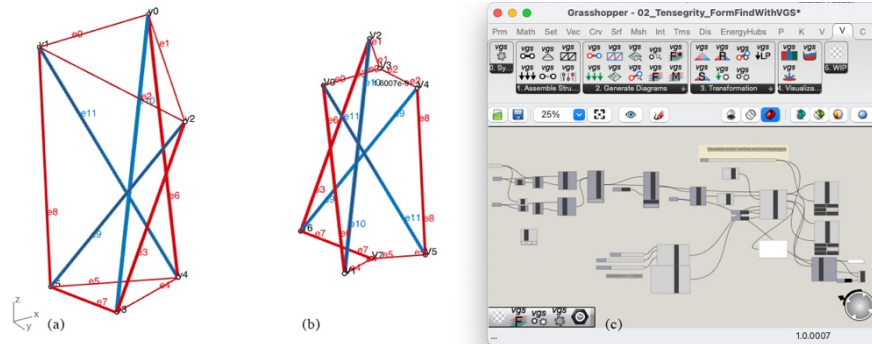
Fig. 3 View of a structural model of a 3D tensegrity structure in the VGS tool within the McNeel Rhinoceros and Grasshopper digital environment. From left to right: Form diagram (a), corresponding Force Diagram (b), parametric definition with the VGS modules in Grasshopper (c)
