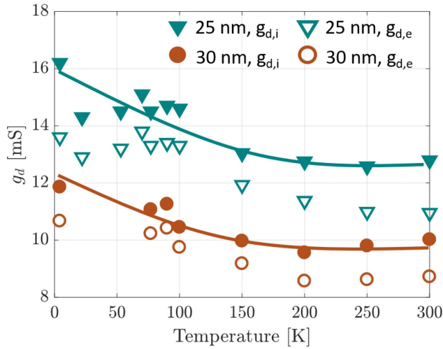
FIGURE 10. g_{d,i} (solid line, filled markers) and g_{d,e} (empty markers) versus temperature for 25 (‘v’) and 30 nm-long devices (‘o’), at V_{ds} = 1 V and V_{gs} corresponding to g_{m,max} .
