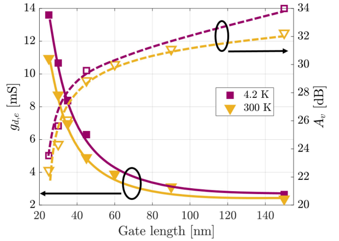
FIGURE 12. g_{d,e} (solid lines, left) and A_v (dashed lines, right) versus gate length at 4.2 K (‘s’) and 300 K (‘v’), at V_{ds} = 1 V and V_{gs} corresponding to g_{m,max} .
