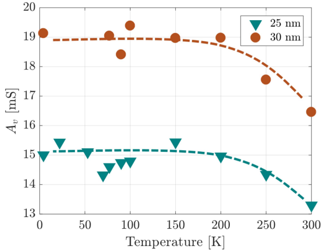
FIGURE 11. A_v versus temperature for 25 (‘v’) and 30 nm-long devices (‘o’), at V_{ds} = 1 V and V_{gs} corresponding to g_{m,max} .
