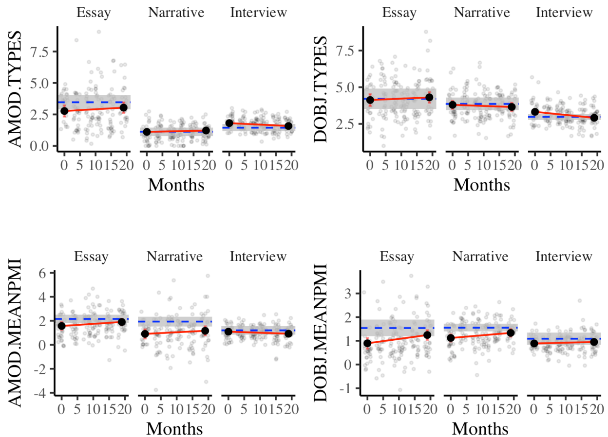
Figure 1. Predicted estimates and raw values of phraseological complexity measures over time (solid red line) compared to L1 benchmark (blue dashed line)
