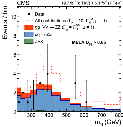
Figure 2: Distributions of the four-lepton invariant mass after a selection requirement on the MELA likelihood discriminant \mathcal{D}_{gg} > 0.65 . Points represent the data, filled histograms the expected contributions from the reducible (Z+X) and q\bar{q} backgrounds, and from the gluon fusion (gg) and vector boson fusion (VV) SM processes (including the Higgs boson mediated contributions). The dashed line corresponds to the total expected yield for a Higgs boson width and a squared product of the couplings scaled by a factor 10 with respect to their SM values. The bin size varies from 20 to 85 GeV and the last bin includes all entries with masses above 800 GeV.
