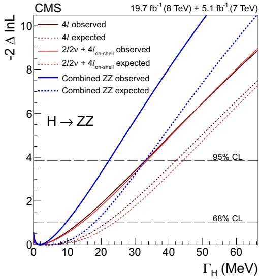
Figure 4: Scan of the negative log-likelihood, -2\Delta\ln\mathcal{L} , as a function of \Gamma_H for the combined fit of the 4\ell and 2\ell 2\nu channels (blue thick lines), for the 4\ell channel alone in the off-shell and on-shell regions (dark red lines), and for the 2\ell 2\nu channel in the off-shell region and 4\ell channel in the on-shell region (light red lines). The solid lines represent the observed values, the dotted lines the expected values.
