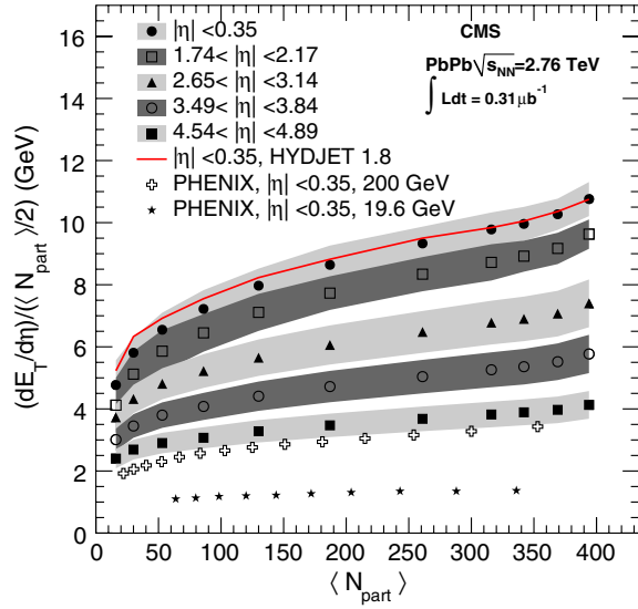
FIG. 2 (color online). Transverse energy density normalized by (\langle N_{\text{part}} \rangle / 2) versus \langle N_{\text{part}} \rangle for Pb-Pb collisions at \sqrt{s_{\text{NN}}} = 2.76 TeV at several values of |\eta| . The bands show the total systematic uncertainties. The statistical uncertainties are negligible. For \eta = 0 , lower-energy PHENIX data and results from the HYDJET 1.8 model are also shown.
