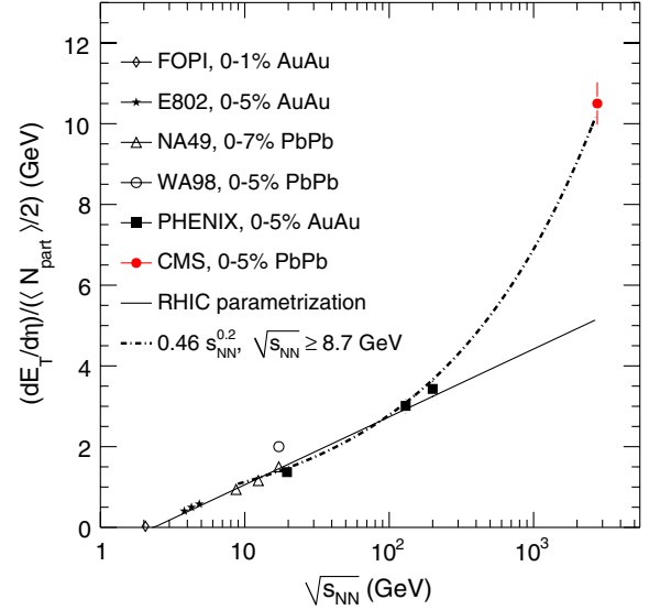
FIG. 3 (color online). Transverse energy density normalized by (\langle N_{\text{part}} \rangle / 2) for central collisions at \eta = 0 versus \sqrt{s_{\text{NN}}} . The vertical bar on the CMS point is the full systematic uncertainty. The statistical uncertainty is negligible. The solid line is a parametrization of lower-energy data compiled by the PHENIX Collaboration; see [22,30–37]. The dashed line corresponds to a power-law fit s_{\text{NN}}^n for \sqrt{s_{\text{NN}}} \geq 8.7 GeV.
