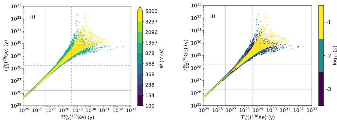
Figure 9. Comparison of ^{136}\text{Xe} and ^{76}\text{Ge} 0\nu\beta\beta decay lifetimes for a scan of points that produce correct BAU and are not ruled out by peak searches or BBN constraints, marginalising over \mu \in \{10^{-1}, 10^{-2}, 10^{-3}\} , and 100 \text{ MeV} \lesssim \bar{M} \lesssim 100 \text{ GeV} in the inverted hierarchy. The different colours represent the largest possible \bar{M} and \mu (for specific values of the ^{136}\text{Xe} and ^{76}\text{Ge} 0\nu\beta\beta decay lifetimes) found by our scan. The current 0\nu\beta\beta limits are shown with solid grey lines [13, 164], while the dotted lines denote an improvement of two orders of magnitude.
