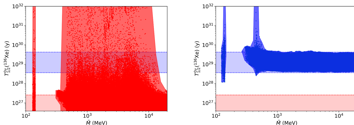
Figure 11. Population of the non-standard T_{1/2}^{0\nu} region in the IH (red, left panel) and NH (blue, right panel). The standard bands with 3 light neutrino exchange 0\nu\beta\beta decay are shown in light blue (NH) and light red (IH). Only points that survive experimental and BBN constraints and are consistent with the measured BAU are shown, and the regions containing all the points found are shaded in dark red (IH) and blue (NH). Below \sim 300 MeV, a combination of cosmological and experimental limits exclude the entire parameter region apart from the window near the pion mass (see figure 6).
