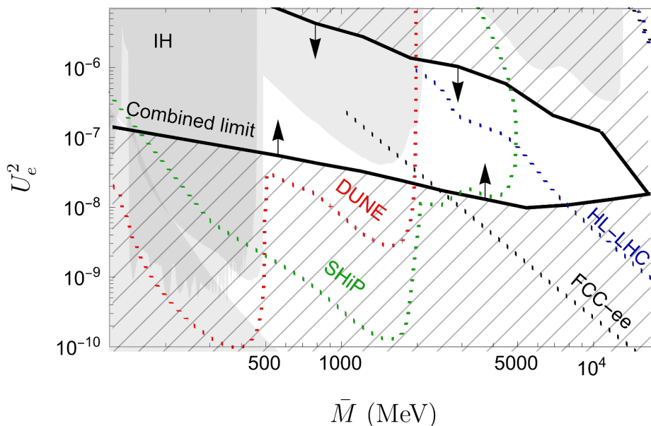
Figure 8. Future (projected) constraints on U_e^2 for IH marginalized over \mu in absence of any observation of 0\nu\beta\beta . Combined limits from T_{1/2}^{0\nu}(^{136}\text{Xe}) > 3.8 \cdot 10^{28} y, leptogenesis, and current experimental and BBN constraints, would force the mixing angle to lie within the region bounded in black (the arrows point towards the allowed region). The dotted lines represent projected upper bounds on U_e^2 from DUNE, SHiP, HL-LHC, and FCC-ee, while the currently constrained regions are shaded in grey (see figure 6 for details).
