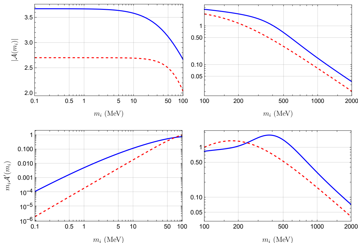
Figure 1. |\mathcal{A}(m_i)| and m_i \mathcal{A}'(m_i) for ^{136}\text{Xe} in the low (left panels) and intermediate (right panels) mass regime. The red dashed lines represent the prediction from eq. (4.5) whereas the blue line is based on the chiral EFT approach.
