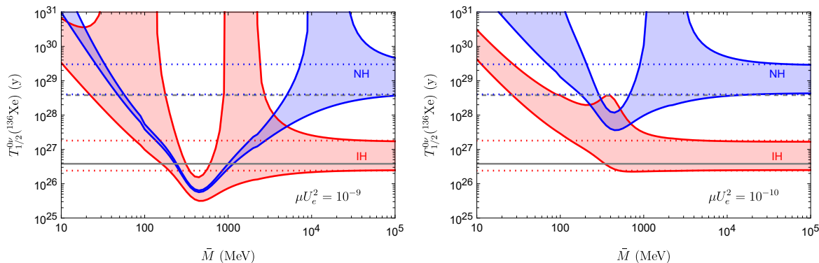
Figure 2. 0\nu\beta\beta lifetimes for selected values of \mu U_e^2 as a function of \bar{M} . The existing 0\nu\beta\beta limits are shown with grey solid lines, while the dashed lines represent a 100\times improvement on the limits. The dotted lines (blue for NH and red for IH) indicate the bands obtained when no contribution from HNLs is considered.
