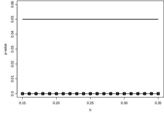
Figure 2: Graphics of the p -values as function of the bandwidth h obtained from 1000 bootstrap replications with the test statistics T_{KS}^1 (line with circles) and T_{CM}^1 (line with crosses). The solid horizontal line corresponds to a p -value of 0.05.
