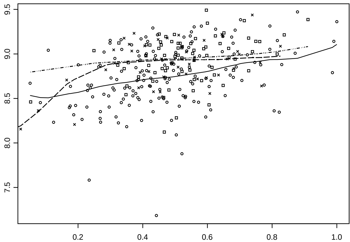
Figure 1: Scatter plot of 'log(food expenditure)' versus 'log(total expenditure)' and estimated regression curves of households consisting of 2 members (circles and solid line), 3 members (crosses and dashed line) and 4 members (squares and dashed dotted line).
