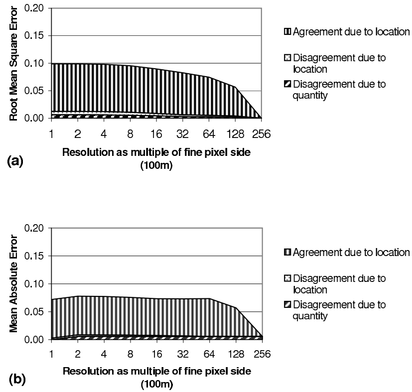
Figure 6.4: Multiple resolution budget of components of information based on (a) Root Mean Square Error and (b) Mean Absolute Error. Eq. 5.5 to 5.10 are used to compare the maps of the CI and IC approaches for the AF_T model, as a function of the level of spatial aggregation.
