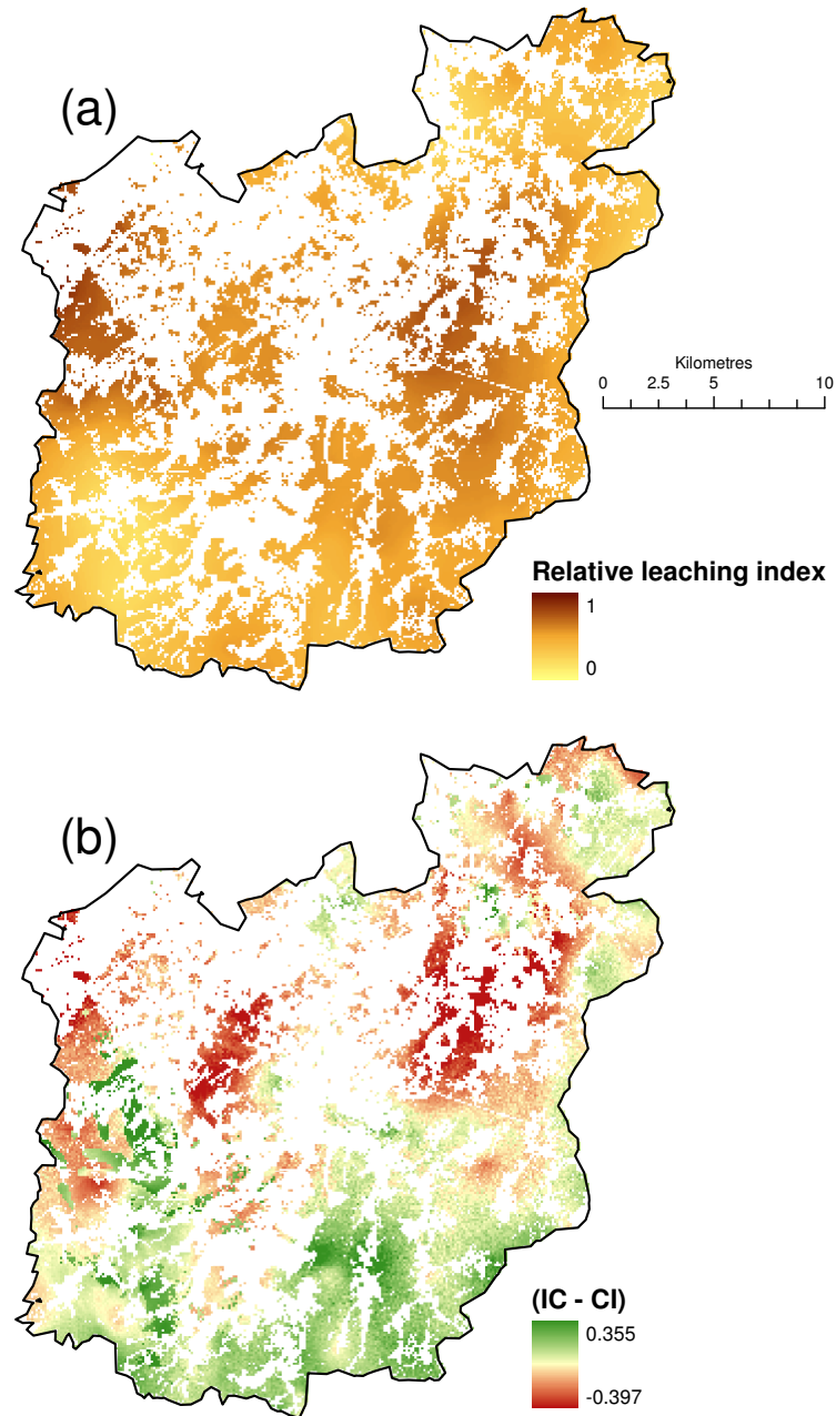
Figure 6.5: Maps showing the relative leaching index calculated by the non-linear GeoPEARL model. (a) CI approach and (b) difference between IC and CI. White areas are non-arable land.
