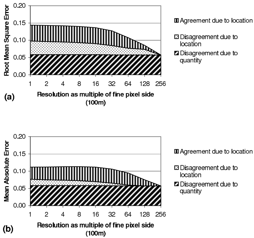
Figure 6.6: Multiple resolution budget of components of information based on (a) Root Mean Square Error and (b) Mean Absolute Error. Eq. 5.5 to 5.10 are used to compare the maps of the CI and IC approaches for the GeoPEARL model, as a function of the level of spatial aggregation.
