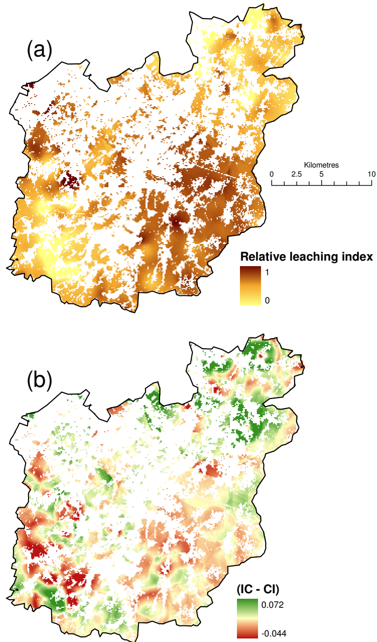
Figure 6.3: Maps showing the relative leaching index calculated by the linear AF_T model. (a) CI approach and (b) difference between IC and CI. White areas are non-arable land.
