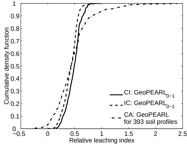
Figure 6.8: Cumulative density function of relative leaching scores calculated with the GeoPEARL model.
