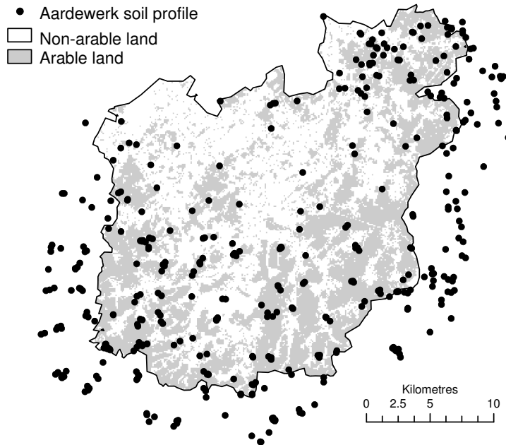
Figure 6.1: Land use and spatial distribution of the soil profiles in the study area (including a buffer zone of 4 km). Only the soil profiles located on arable land were selected in the Aardewerk database.
