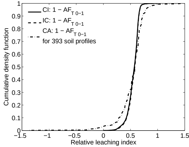
Figure 6.7: Cumulative density function of relative leaching scores calculated with the AF_T method.
