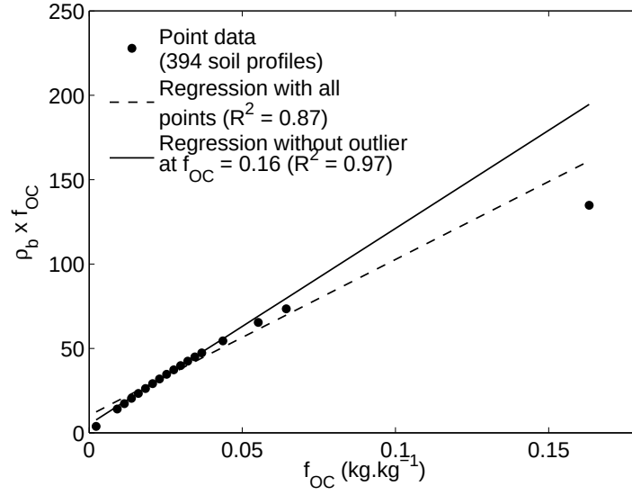
Figure 6.2: Linear regression with [\rho_b \times f_{OC}] as the dependent variable and f_{OC} as the independent variable. The regression fit is shown with all data (dashed line; N = 394 and R^2 = 0.87 ) and without the outlier plotted at f_{OC} = 0.16 (solid line; N = 393 and R^2 = 0.97 ).
