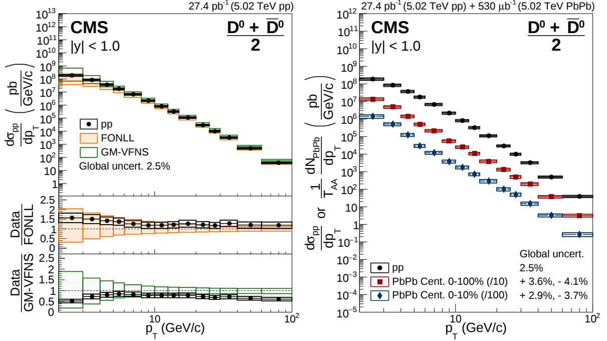
Figure 2: (left) The p_T -differential production cross section of D^0 mesons in pp collisions at \sqrt{s} = 5.02 TeV. The vertical bars (boxes) correspond to statistical (systematic) uncertainties. The global systematic uncertainty, listed in the legend and not included in the point-to-point uncertainties, comprises the uncertainties in the integrated luminosity measurement and the D^0 meson \beta . Results are compared to FONLL [32] and GM-VFNS [34–36] calculations. (right) The p_T -differential production yields of D^0 mesons divided by the nuclear overlap functions T_{AA} for PbPb collisions in the 0–100% (red) and 0–10% (blue) centrality ranges compared to the same pp cross sections shown in the left panel (black).
