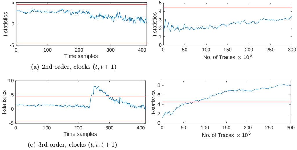
Figure 7: Multivariate non-specific t -test results with 300 million measurements for a single GF(2^4) multiplier masked by means of CMS with d = 3 . The left column depicts the t -values over time, the right column illustrates the evolution of the absolute maximum t -value over the number of traces.
