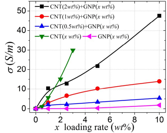
Figure 2. Measured conductivity of polycarbonate nanocomposite with various CNT, GNP loading rate.
