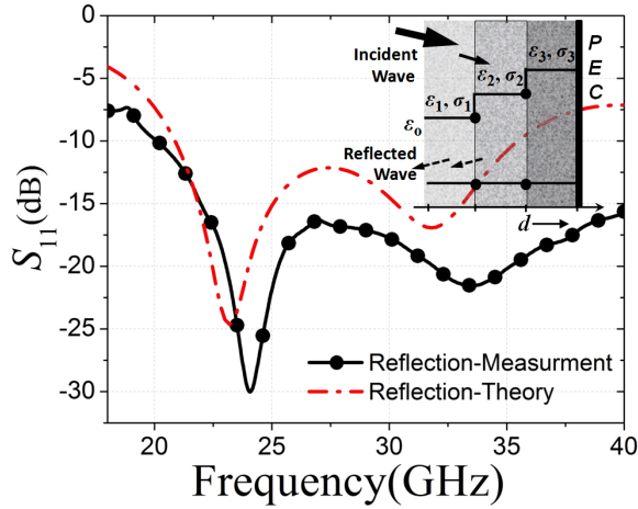
Figure 5. Reflection coefficient ( S_{11} ) for 3-layer absorber of thickness 3.2 mm. Inset: absorber schematic.
