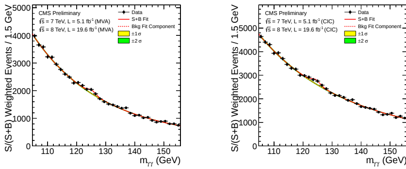
Figure 3. The diphoton invariant mass distribution with each event weighted by the S/(S+B) value of its category, for the mass-fit-MVA (left) and cut-based (right) analyses on the 7 and 8 TeV data sets combined. The lines represent the fitted background and signal, and the coloured bands represent the \pm 1 and \pm 2 standard deviation uncertainties in the background estimate.
