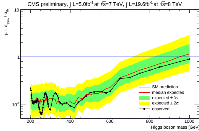
Figure 8. Observed (black line) and expected (red line) 95% CL upper limit on the ratio of the product of the production cross section and branching fraction to the SM expectation for the Higgs boson decaying into two Z bosons obtained using the asymptotic CLs technique. The 68% and 95% CL ranges of expectation for the background-only model are also shown with green and yellow bands, respectively. The horizontal solid line at unity indicates the SM expectation. Result is combination of all individual channels: H \rightarrow ZZ \rightarrow 2l2l , H \rightarrow ZZ \rightarrow 2l2\nu and H \rightarrow ZZ \rightarrow 2l2q .
