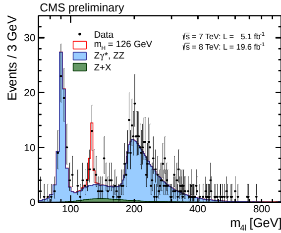
Figure 1. Distribution of the four-lepton reconstructed mass in for the sum of the 4e, 4\mu , and 2e2\mu channels. Points represent the data, shaded histograms represent the background and the unshaded histogram the signal expectation. The expected distributions are presented as stacked histograms. The measurements are presented for the sum of the data collected at \sqrt{s} = 7 TeV and \sqrt{s} = 8 TeV. No event is observed for m_{4l} > 800 GeV.
