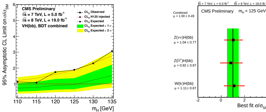
Figure 5. Expected and observed 95% CL upper limits on the product of the VH production cross section times the Hbb branching ratio, with respect to the expectations for a standard model Higgs boson. The median expected limit and the 1- and 2-sigma bands are obtained with the LHC CLs method as implemented in RooStats, as are the observed limits at each mass point. The limits are combined for the 2011 7 TeV and the 2012 8 TeV data. The red dashed line represents the expected observed limits obtained from replacing the data with the sum of expected background and signal for a Higgs boson at a mass of 125 GeV (left). The most likely value of the production cross section for a 125 GeV Higgs boson, relative to the standard model cross section, for each channel and for all channels combined (right).
