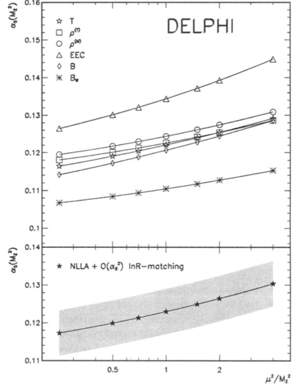
Fig. 9. Upper plot: Values of \alpha_s(M_Z^2) obtained at different scales \mu^2/M_Z^2 from fits to the distributions in thrust, heavy jet masses, jet broadening variables and back-to-back energy-energy correlation. All fits are performed by using the \ln R -scheme. Lower plot: Combined \alpha_s values as a function of the scale \mu^2/M_Z^2 using the \ln R -scheme. The width of the band corresponds to the full experimental and theoretical error of the combined value
