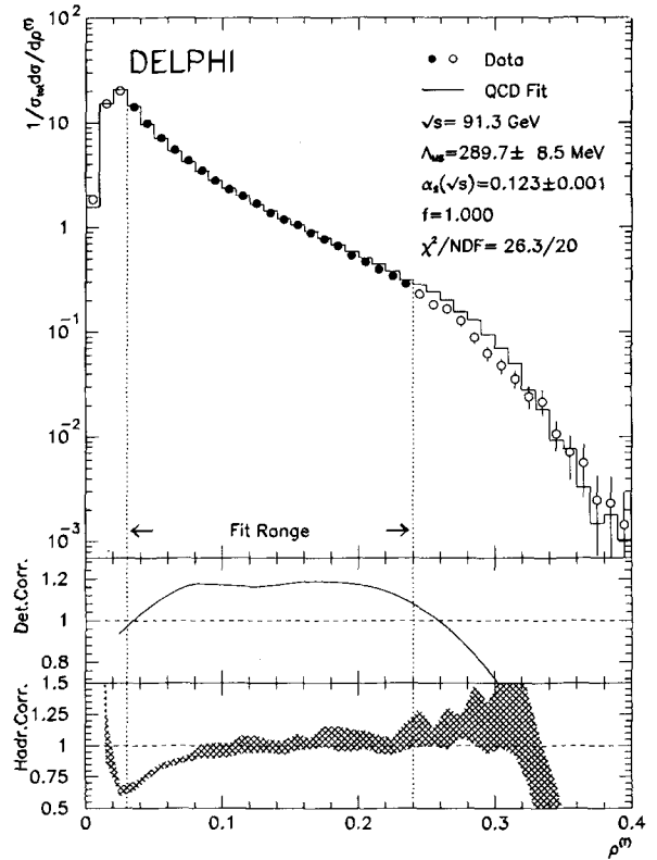
Fig. 4. As Fig. 3 but for the heavy jet mass (thrust definition)
