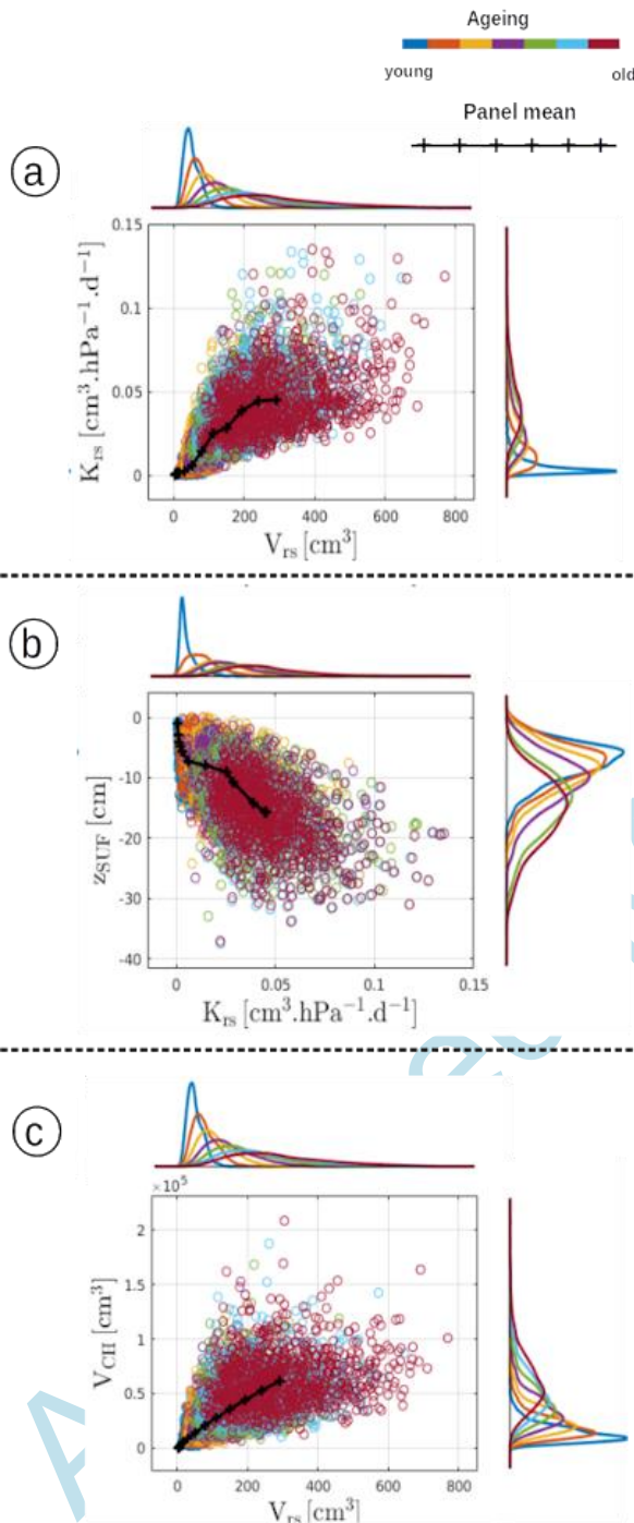
Figure 3: Example of maize virtual panel generation ( N = 10\,000 ). The three subplots represent the relationships between root system hydraulic and/or architectural properties for a large number of maize individuals as they age (see Table 1), as well as the panel mean (black solid lines). The resulting density distributions are also represented over time with the same colour scale.
