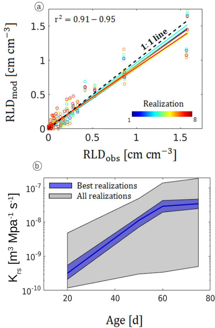
Figure 5: Maize root length density profile goodness of fit using MARSHAL for the 8 best realizations (a) and corresponding RS conductance change envelopes (b) with age for the whole panel of 10 000 simulation runs (grey) and the eight best simulations (blue).
