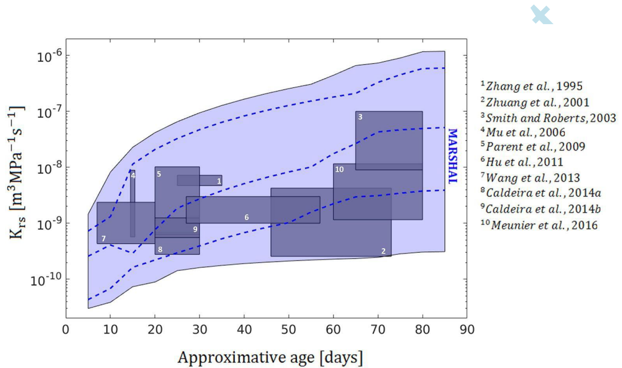
Figure 4: Comparison between maize root system conductances observed in the literature (grey boxes) and the range of conductances simulated using MARSHAL (blue envelope) over the full crop cycle. Dashed lines are three particular realizations of root system conductance trajectories.
