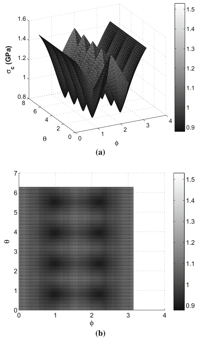
Fig. 4 Distribution of \sigma_c within a unit cube of polySi
