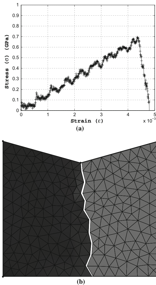
Fig. 21 a Stress versus strain plot, and b complete fracture of a polySi film, having a notch, at the macroscopic level
