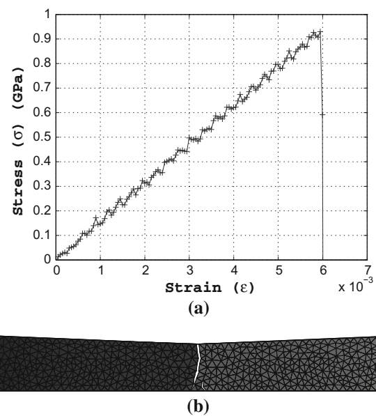
Fig. 22 a Stress versus strain plot, and b complete fracture of a thin polySi film having l = 23 \mu\text{m} at the macroscopic level
