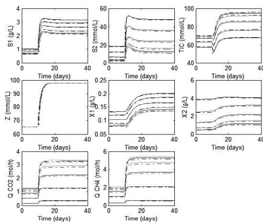
Figure 8. Comparison between the process (dash-dotted lines) and the observer (continuous lines) by placing the sensors at 3.4 m and 3.50 m.
