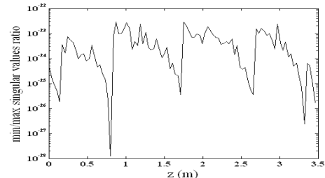
Figure 2. Gramian observability measure using 7 pts.
