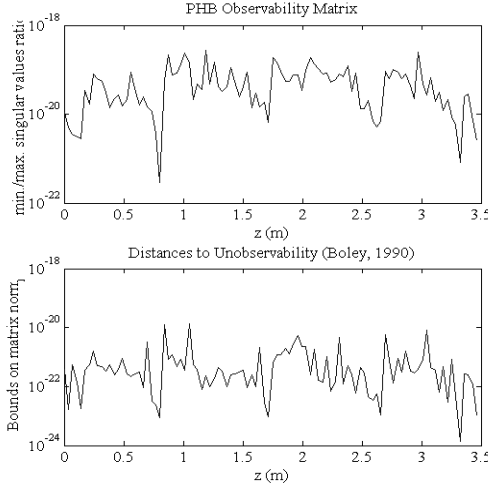
Figure 3. PHB observability measure using 7 points.
