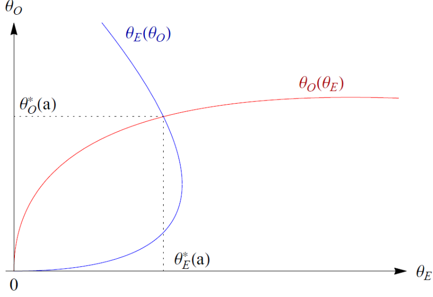
Figure 1: Reaction functions of groups E and O .
