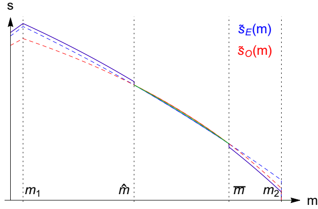
Figure 4: Peace-building, then peace-wrecking diaspora.
