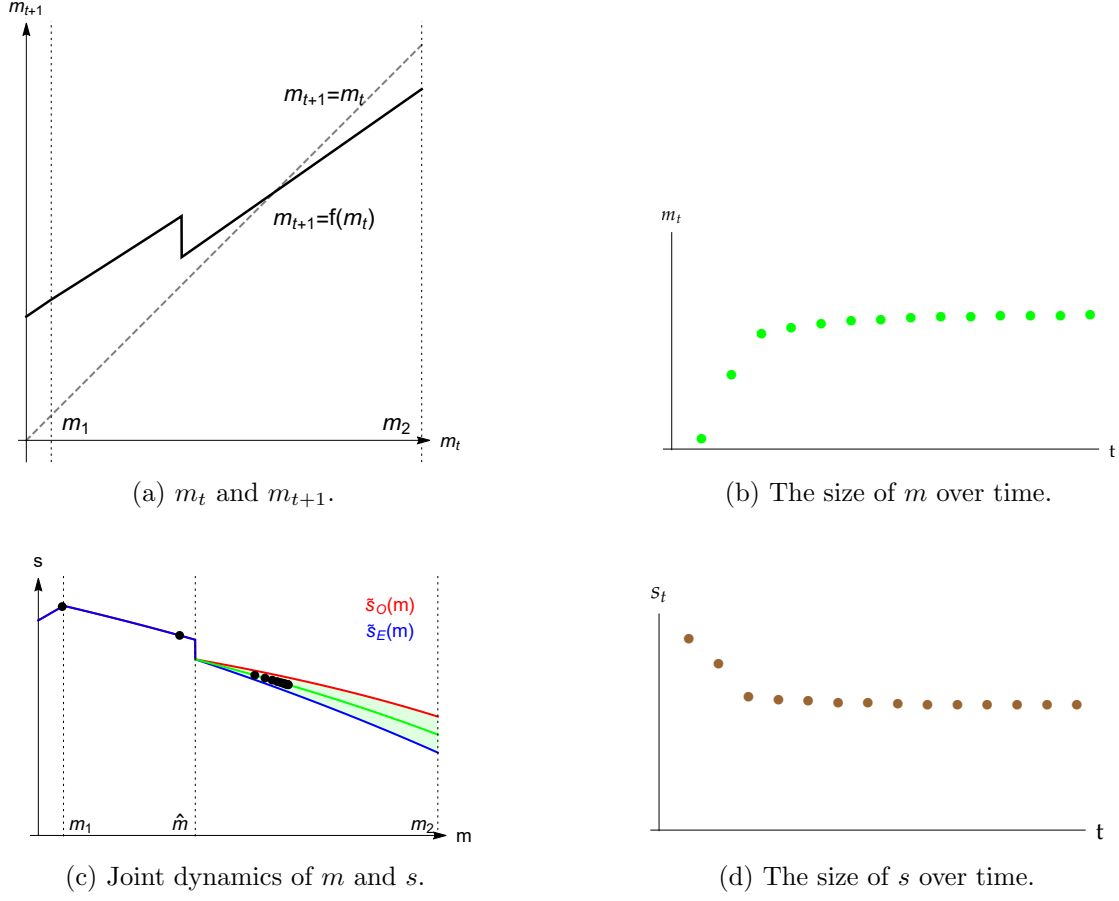
Figure 7: Peace-building scenario: dynamics with high b .
