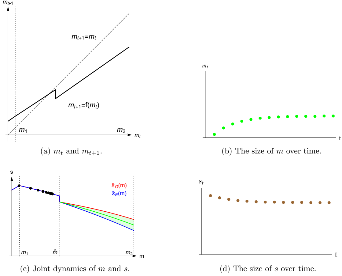
Figure 6: Peace-building scenario: dynamics with low b .
