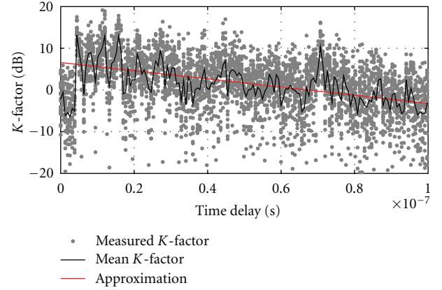
(a) In every scenario, the mean value of the Rice factor K(\tau) presents a linear regression that decreases with the delay
