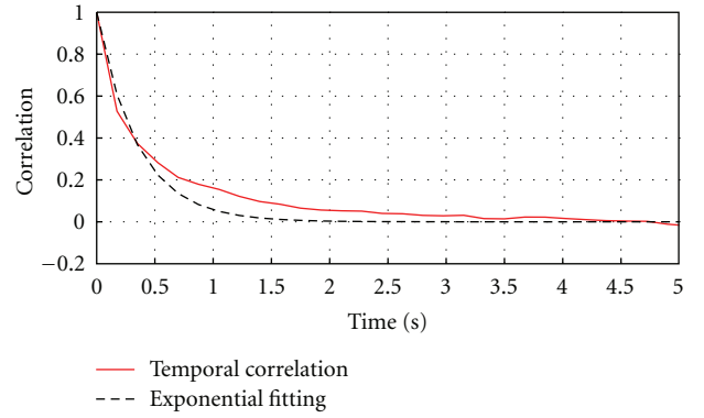
FIGURE 8: The averaged time auto-correlation is fitted with an exponential model.
