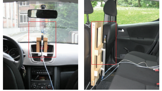
(a) Front Antenna (TX). The TX was placed in the center of the dashboard
