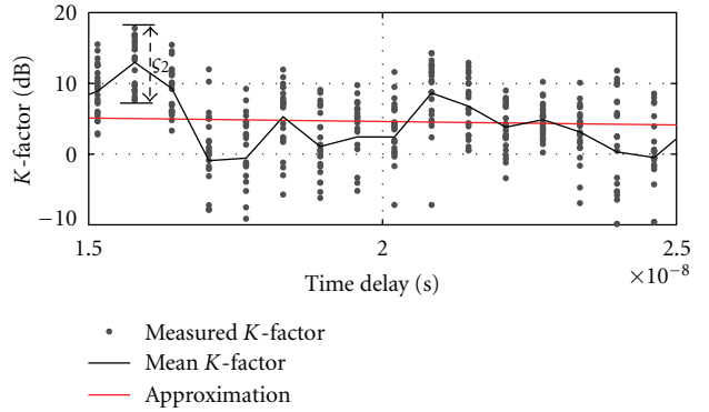
(b) Detailed view of the measured Rice factor K(\tau) . The K -factors present, for each delay, a normal distribution (in dB) around the mean value with a standard deviation represented by \varsigma_2
