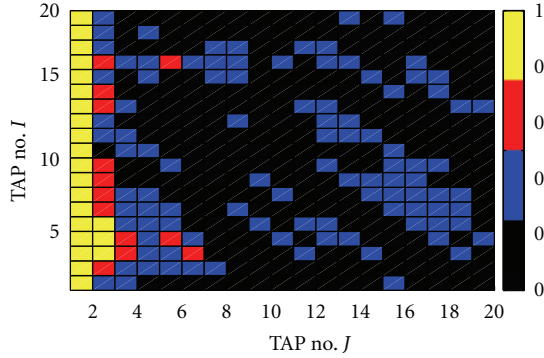
FIGURE 6: Delay correlation of the diffuse component. Only correlation coefficient with adjacent taps have significant values (above 0.5).
