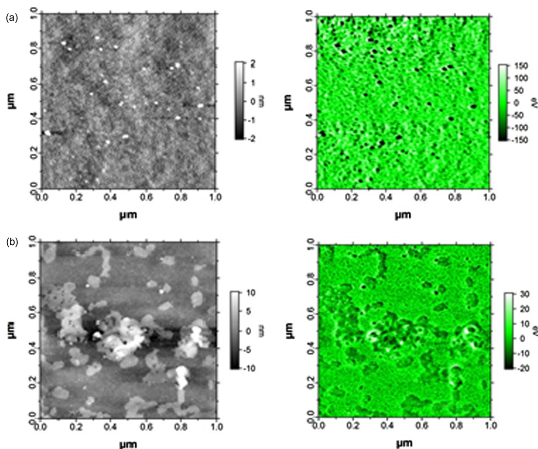
Fig. 8. AFM analysis comparing (a) P-pPDA + 0.5 wt% Bz 1. (b) P-pPDA + 3 wt% Bz 1. PeakForce QNM – topography in grey, energy dissipation in green. (For interpretation of the references to color in this figure legend, the reader is referred to the web version of this article.)
