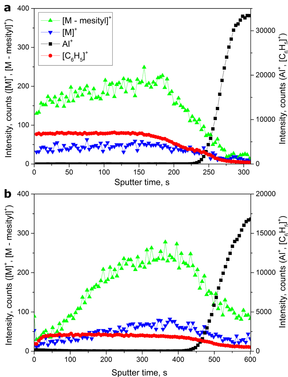
Fig. 10. In depth ToF-SIMS analysis of the quasi-molecular ion (between 661 u. and 666 u.) and the [M - \text{mesityl}]^+ (from 541 u. to 546 u.) in 10 wt% Bz1 coatings before (a) and after curing (b).
