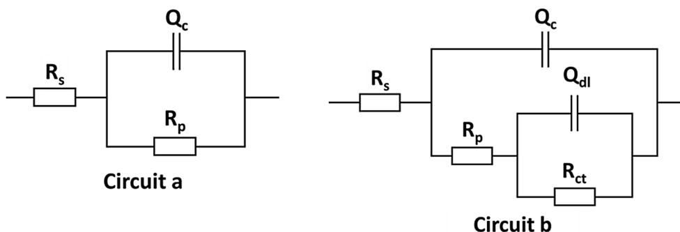
Fig. 12. Equivalent electrical circuits used to fit impedance data.
