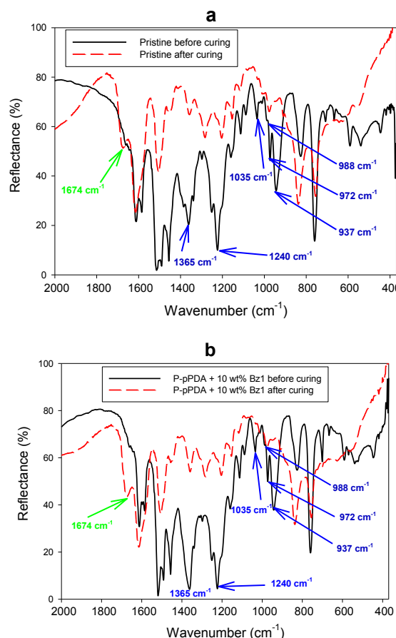
Fig. 2. Comparison of FTIR spectra before and after curing for (a) pristine coatings and (b) P-pPDA + 10 wt% borazine derivative loaded coatings.
