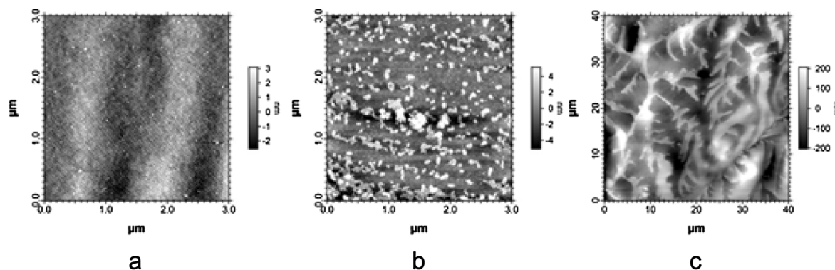
Fig. 7. AFM topography images of borazine 1 derivative containing pPDA polymer composites: (a) polymer pPDA with 0.5 wt% of borazine 1 derivative; (b) 3 wt% of borazine 1 derivative and (c) 10 wt% borazine 1 derivative.
