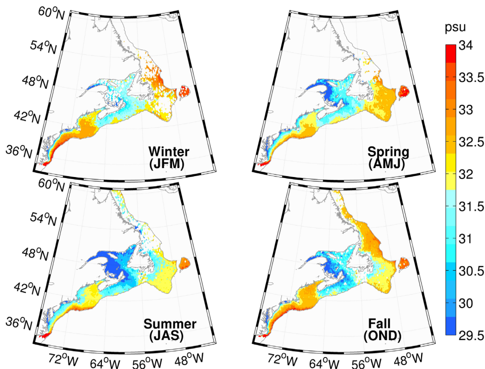
Fig. 15. Mean seasonal maps of SSS. The 600 m isobath is indicated with the gray contour.
