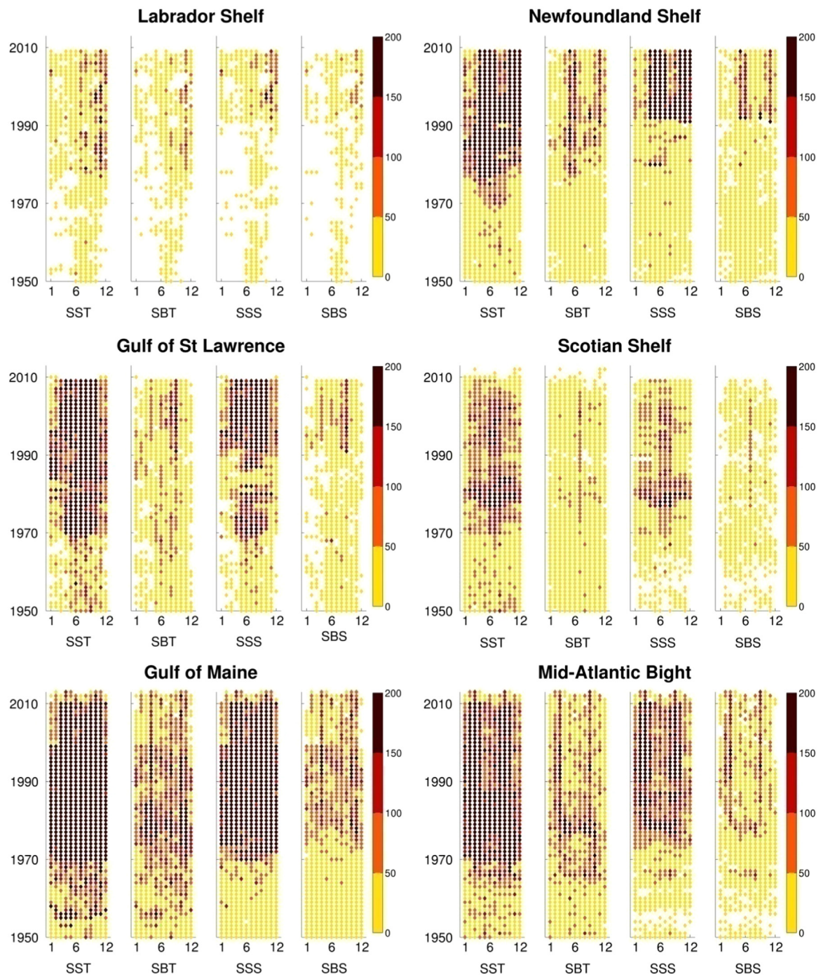
Fig. 8. Temporal distribution of available data, for all six regions, after extrapolation. Gap-filling was only applied to surface temperature between June and December on the Labrador Shelf, while surface temperature and salinity were filled year-round in all other regions. Colors indicate the number of stations. SST, SBT, SSS and SBS stand for sea-surface temperature, sea-bottom temperature, sea-surface salinity and sea-bottom salinity, respectively. (For interpretation of the references to color in this figure, the reader is referred to the web version of this article.)
