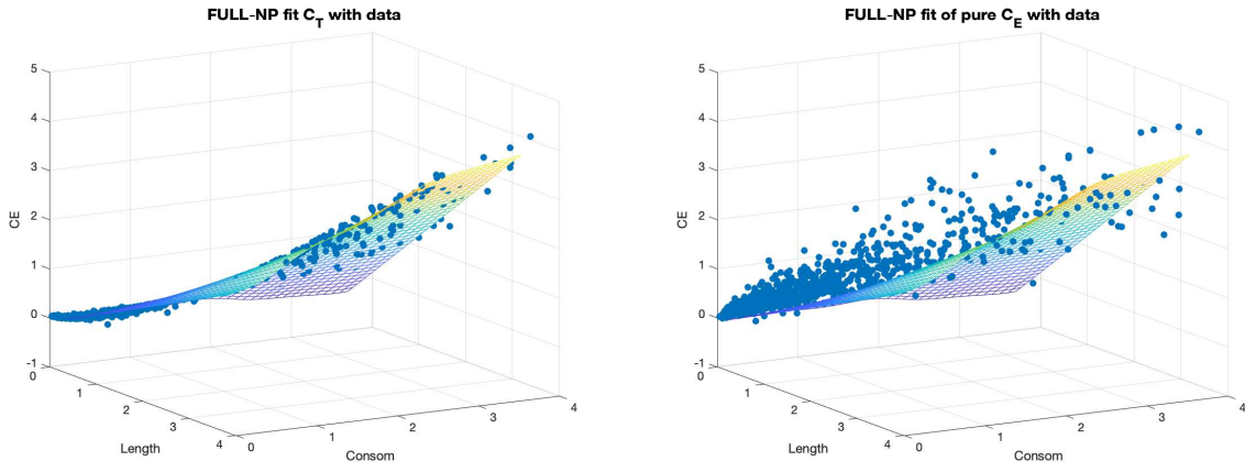
Figure 7: Nonparametric approach: left panel, data points of the observed technical costs C_T and the fitted cost frontier \hat{m}_0(X_i) . Right panel, data points of the observed economic costs C_E and the same fitted cost frontier.
