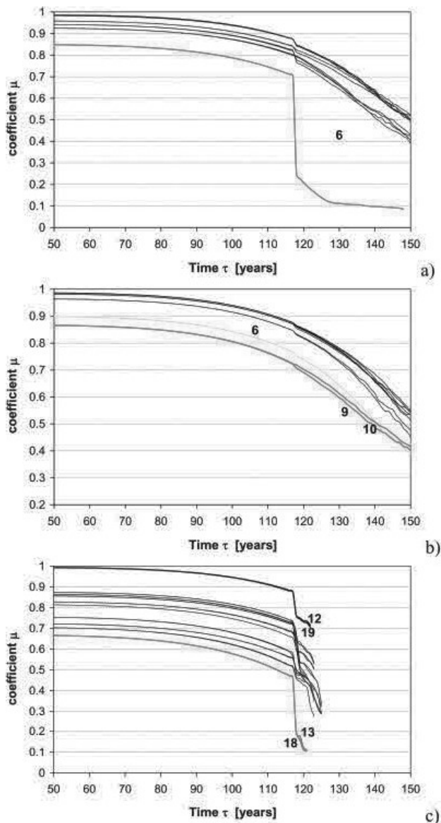
Figure 14. Comparison between index \mu evolution over time for all the members of each roof truss: a) Case 1; b) Case 2; c) Case 3. The most vulnerable components have been highlighted in red and yellow.
