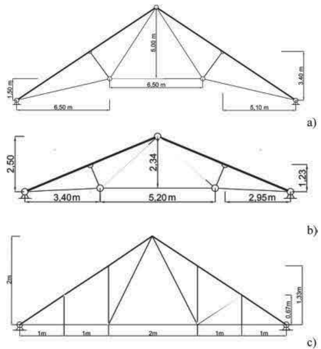
Figure 13. Case studies analysed without considering the members affected by possible failure (dashed lines): a) Case 1; b) Case 2; c) Case 3.
