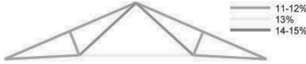
Figure 10. Damage percentage member by member.
