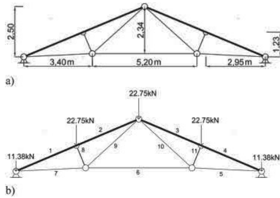
Figure 5. (a) Truss geometry (in metres); (b) Truss static model.
