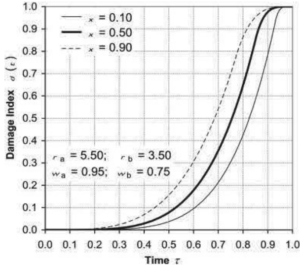
Figure 8. Damage index \delta versus normalized time \tau = t/T_f related to different performance loss percentage \xi .
