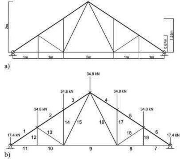
Figure 7. (a) Truss geometry (in metres); (b) Truss static model.
