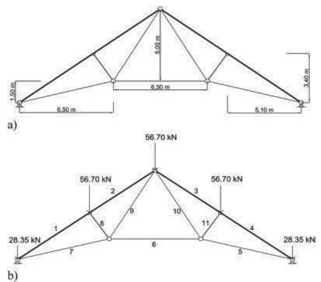
Figure 3. (a) Truss geometry (in metres); (b) Truss static model.
