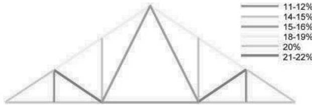
Figure 11. Damage percentage member by member.
