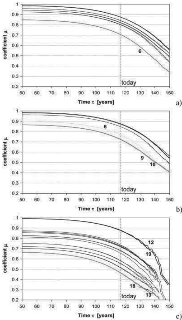
Figure 12. Comparison between index \mu evolution over time for all the members of each roof truss: a) Case 1; b) Case 2; c) Case 3. The most vulnerable components have been highlighted in red and yellow.
